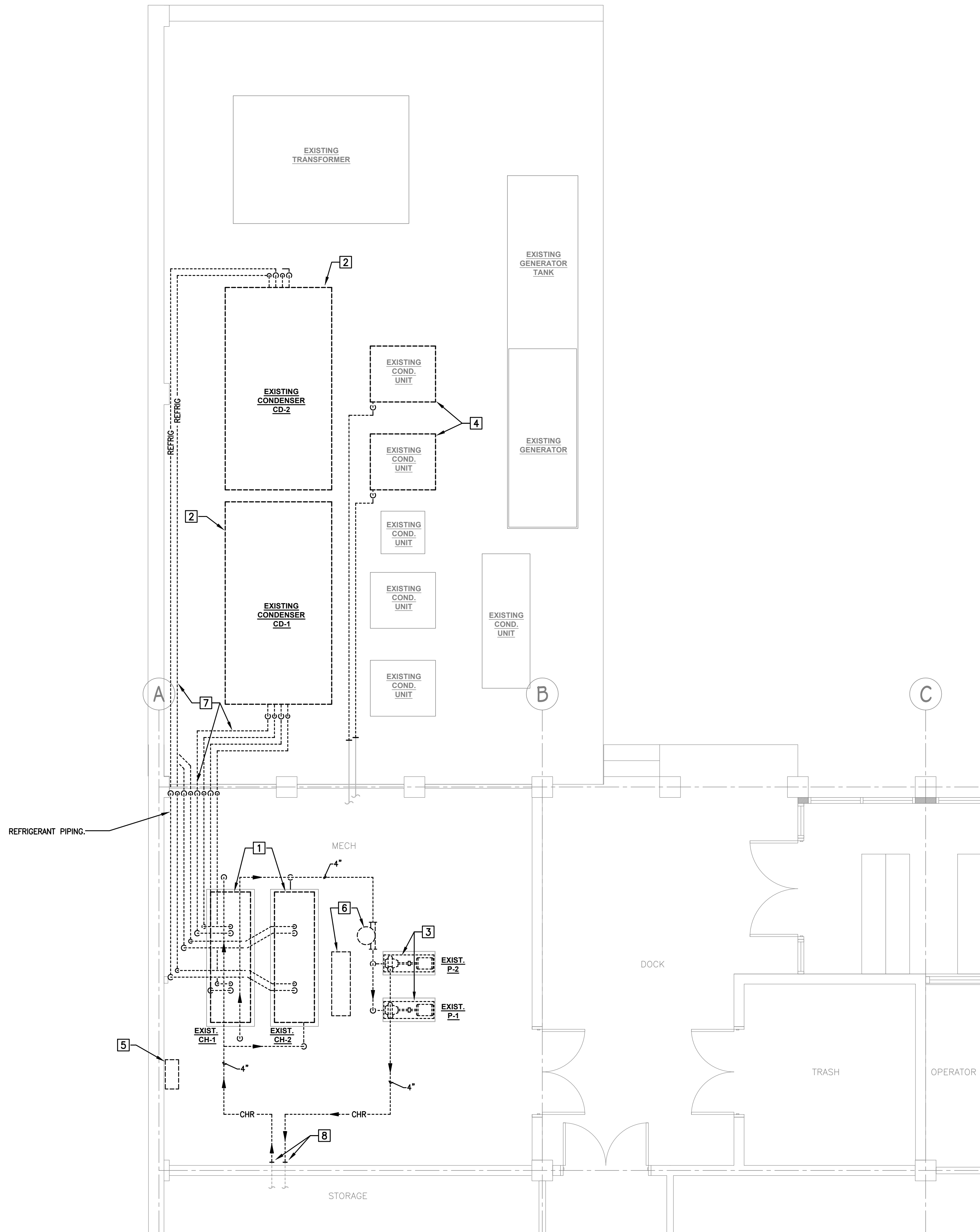
1 DEMOLITION PLAN - PARTIAL GROUND FLOOR - MECHANICAL SCALE : 1/4" = 1'-0"
