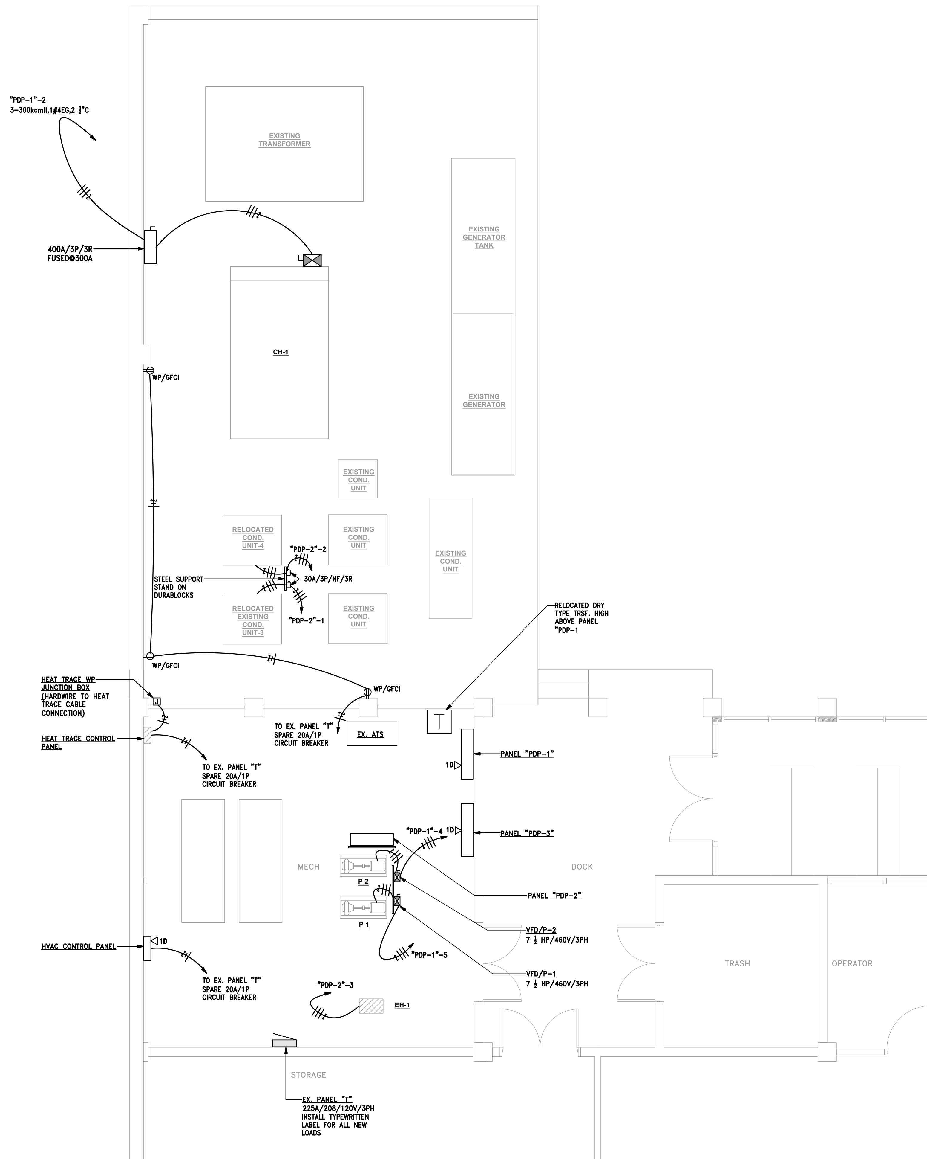
1 NEW PLAN - PARTIAL GROUND FLOOR - ELECTRICAL SCALE : 1/4" = 1'-0"
