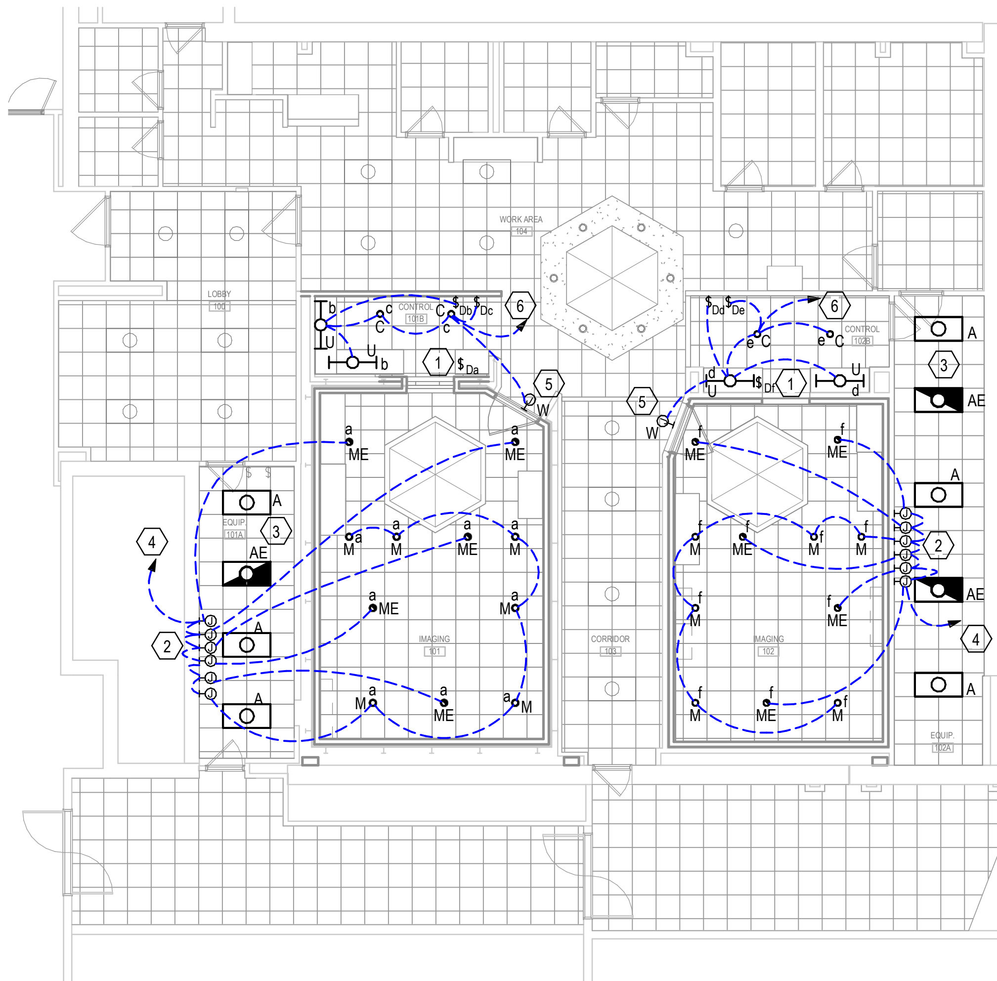
1 IMAGING SUITE LIGHTING PLAN 1/8" = 1'-0"
