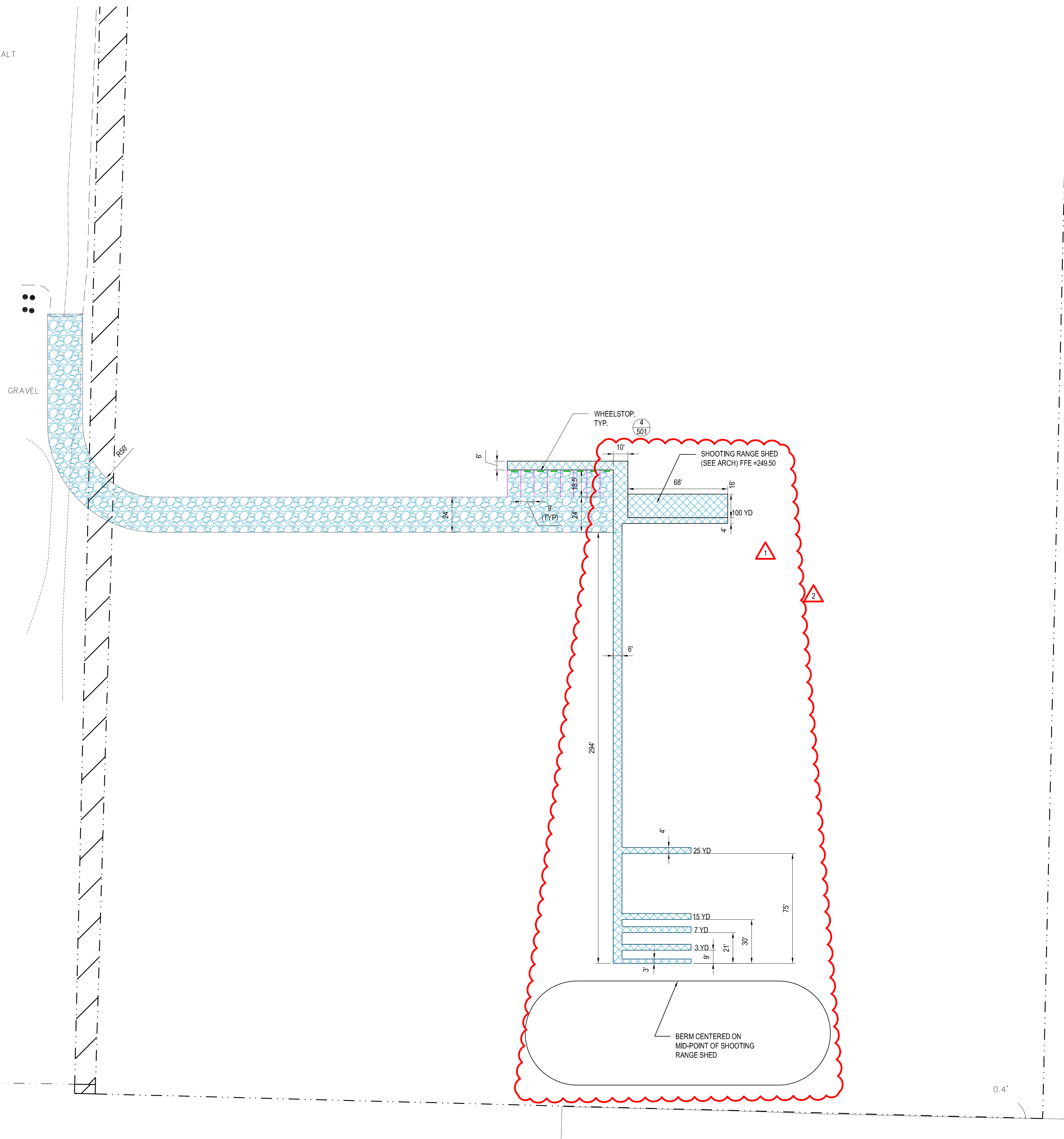
2 TURN DOWN SHED PAD DETAIL NOT TO SCALE
