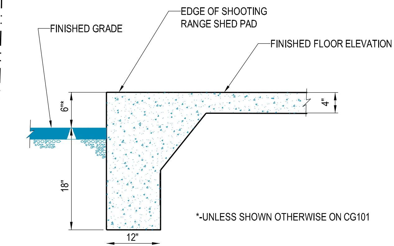
2 TURN DOWN SHED PAD DETAIL NOT TO SCALE
