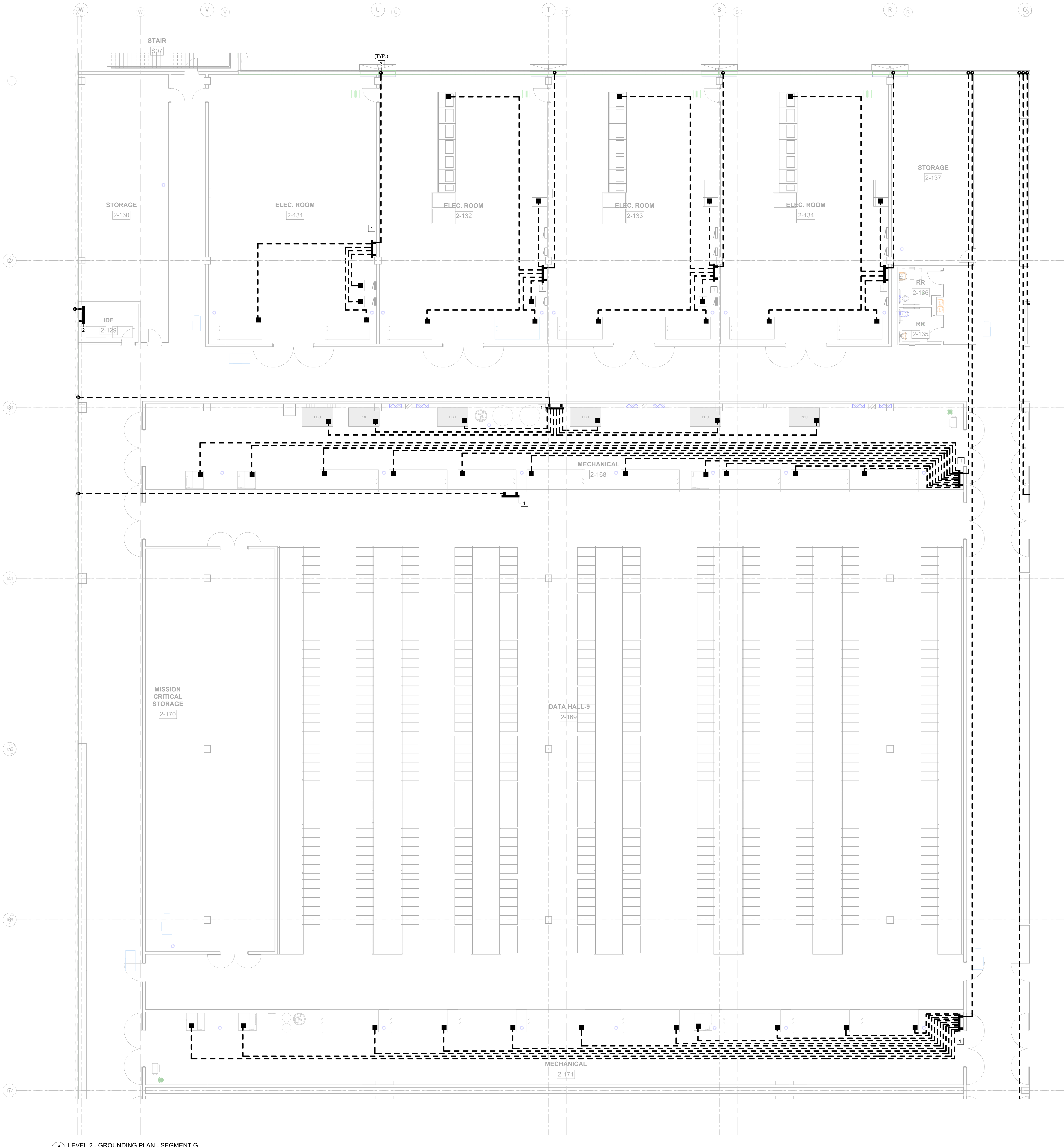
1 LEVEL 2 - GROUNDING PLAN - SEGMENT G 1/8" = 1'-0"
