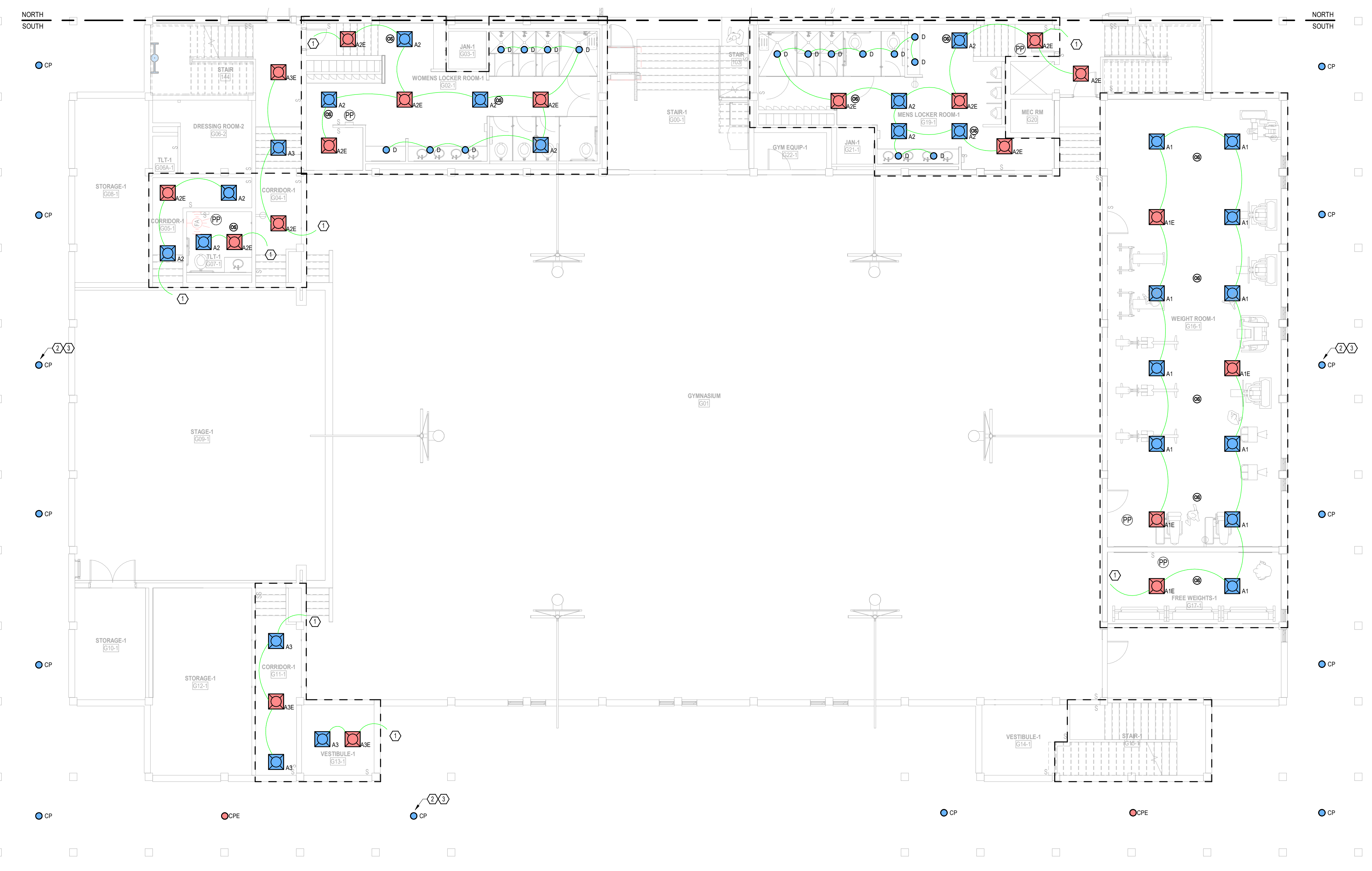
1 GROUND FLOOR PLAN - SOUTH - LIGHTING 1/8" = 1'-0"
