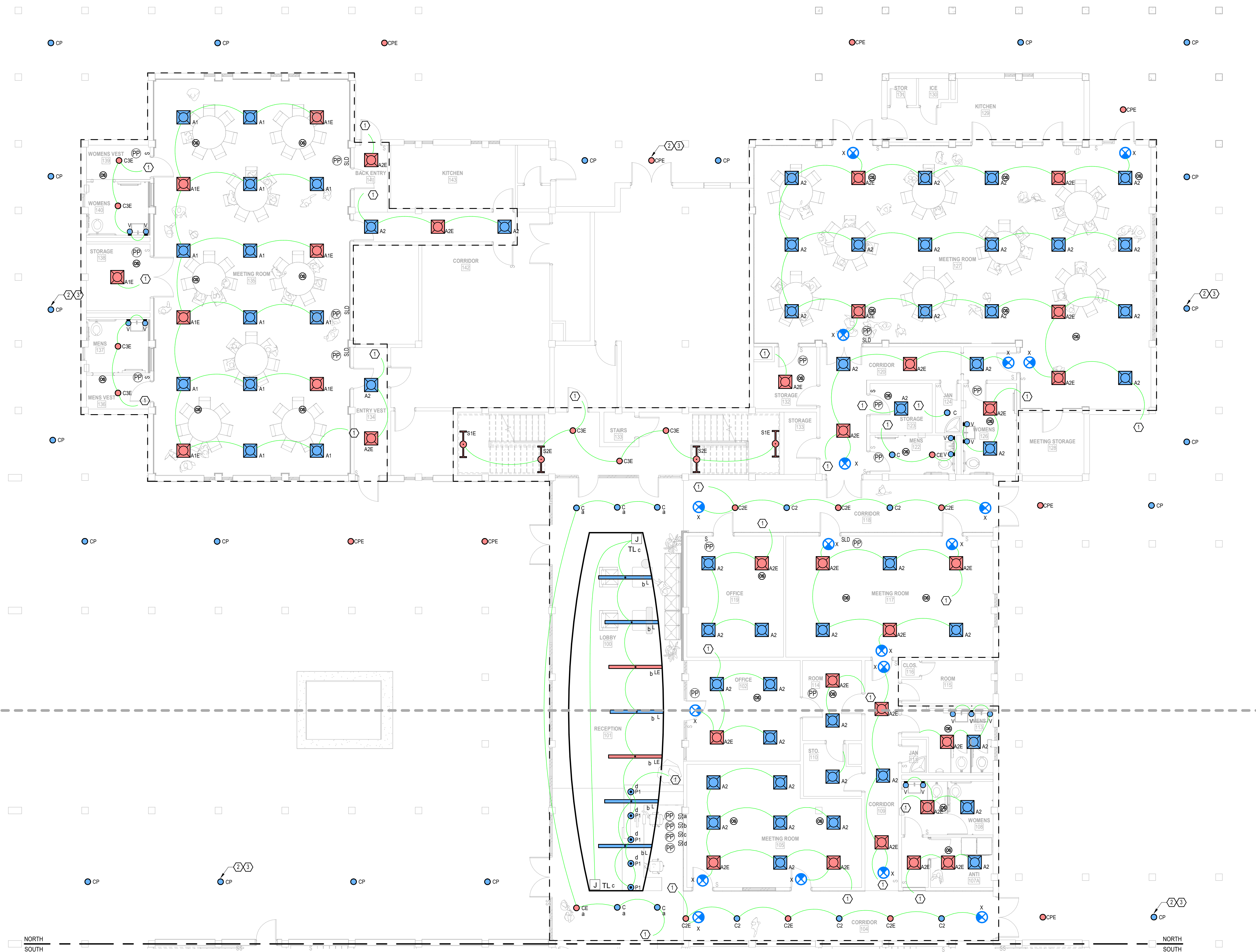
1 GROUND FLOOR PLAN - NORTH - LIGHTING 1/8" = 1'-0"
