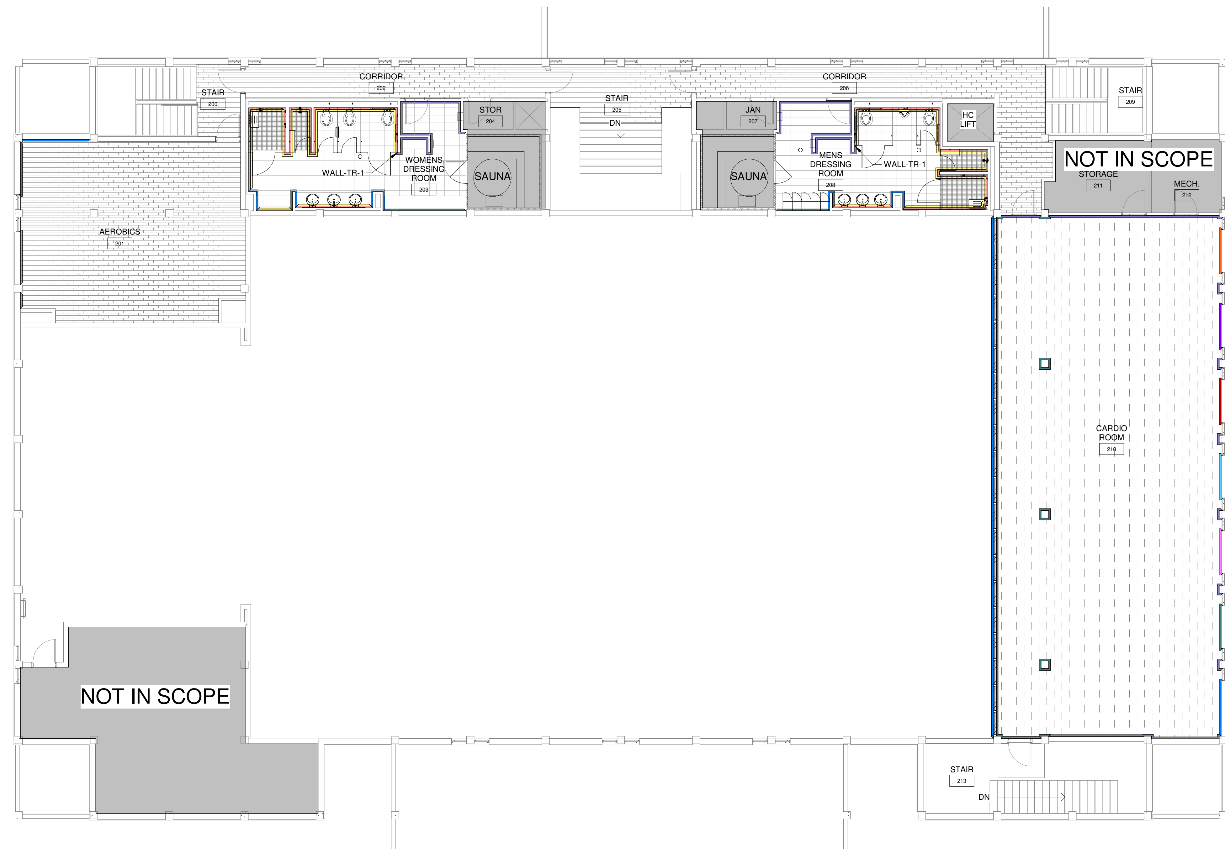
1 SECOND FLOOR FINISH PLAN - SOUTH 1/8" = 1'-0"
