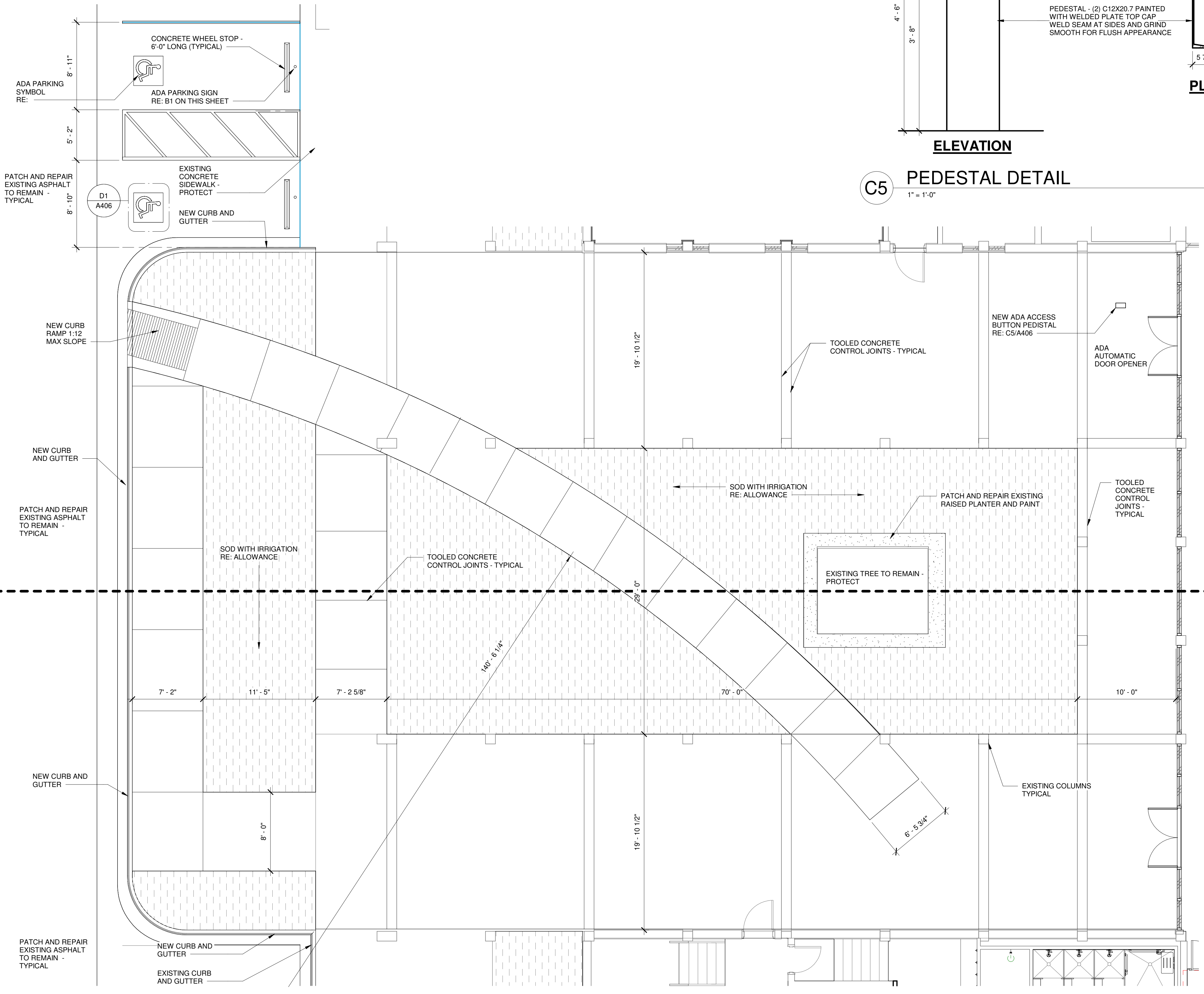
A2 ENLARGED COURTYARD PLAN 3/16" = 1'-0"
