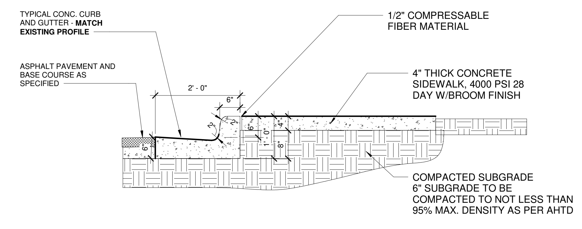
TYPICAL SIDEWALK SECTION
