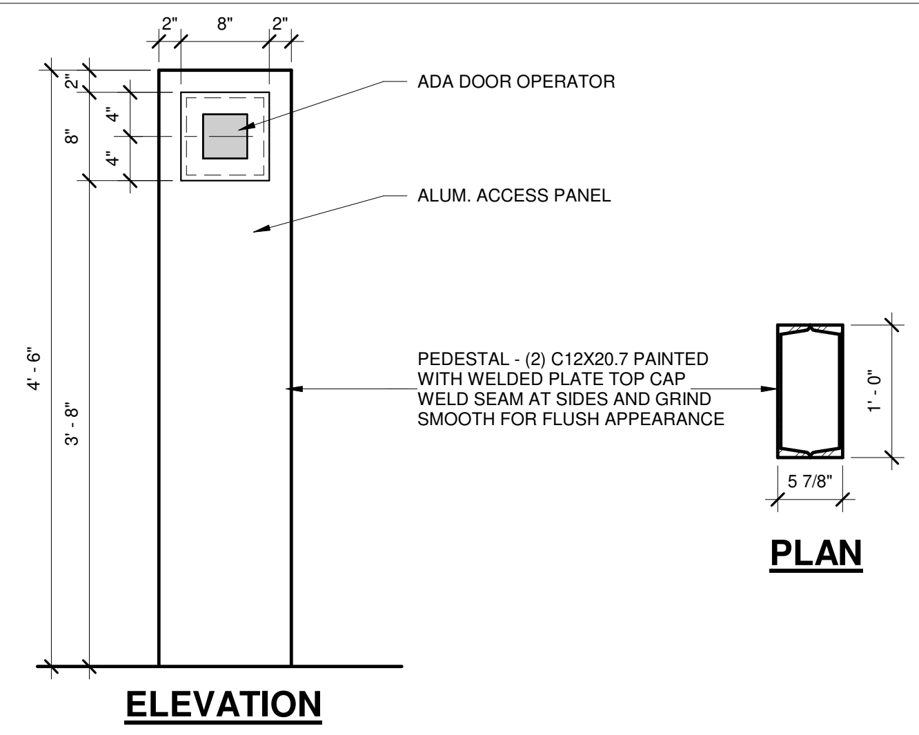
C5 PEDESTAL DETAIL 1" = 1'-0"
