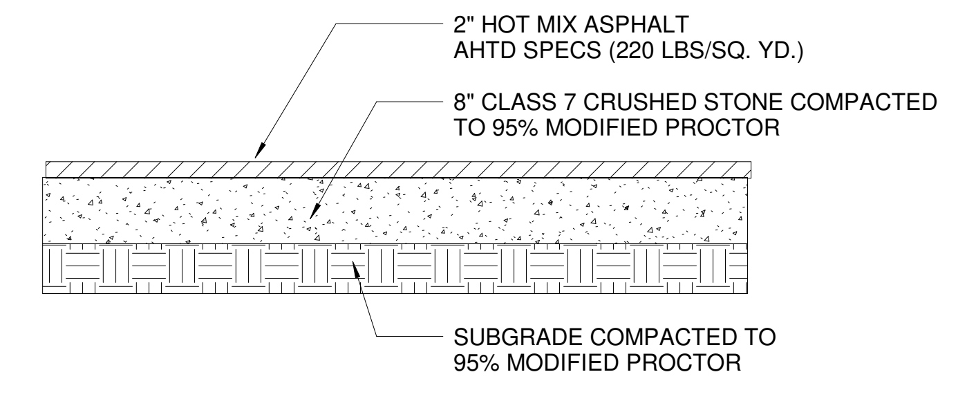
TYPICAL PAVEMENT SECTION - LIGHT DUTY
