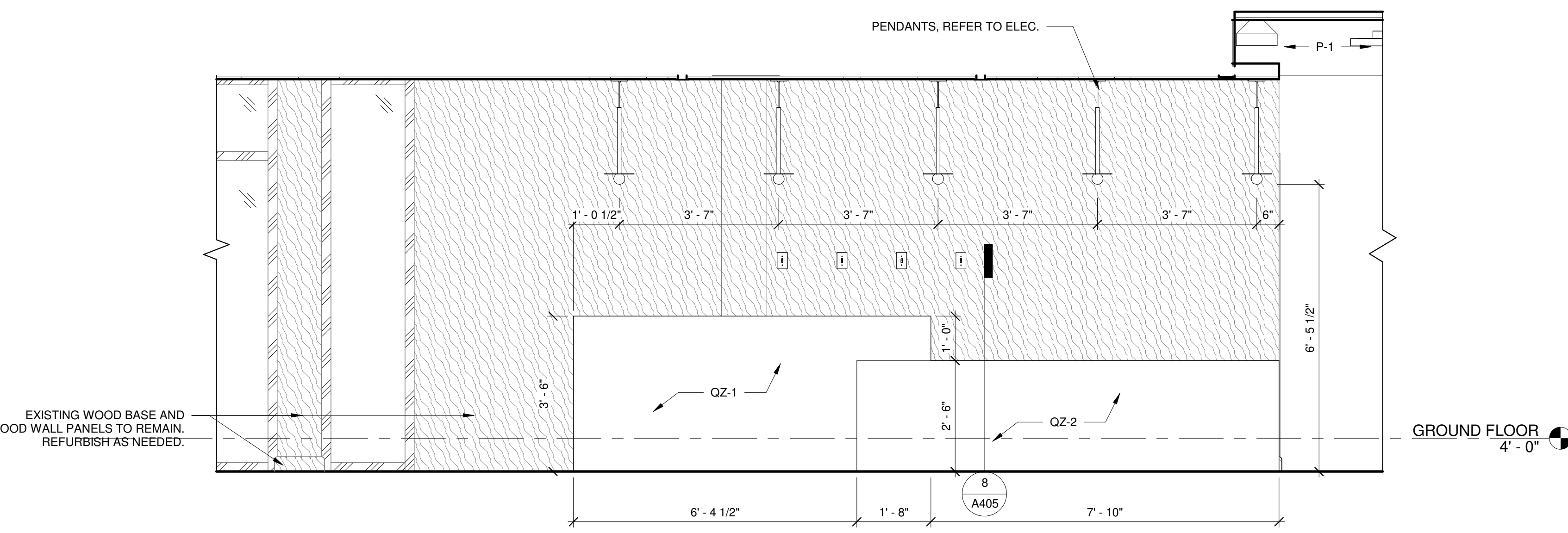
2 RECEPTION DESK - EAST 1/2" = 1'-0"
