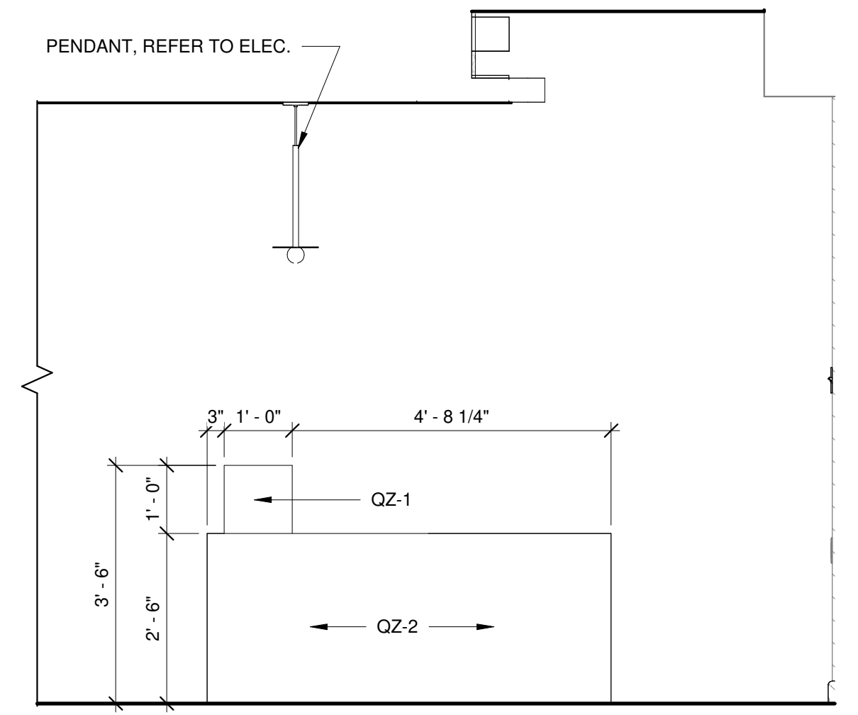
4 RECEPTION - NORTH 1/2" = 1'-0"
