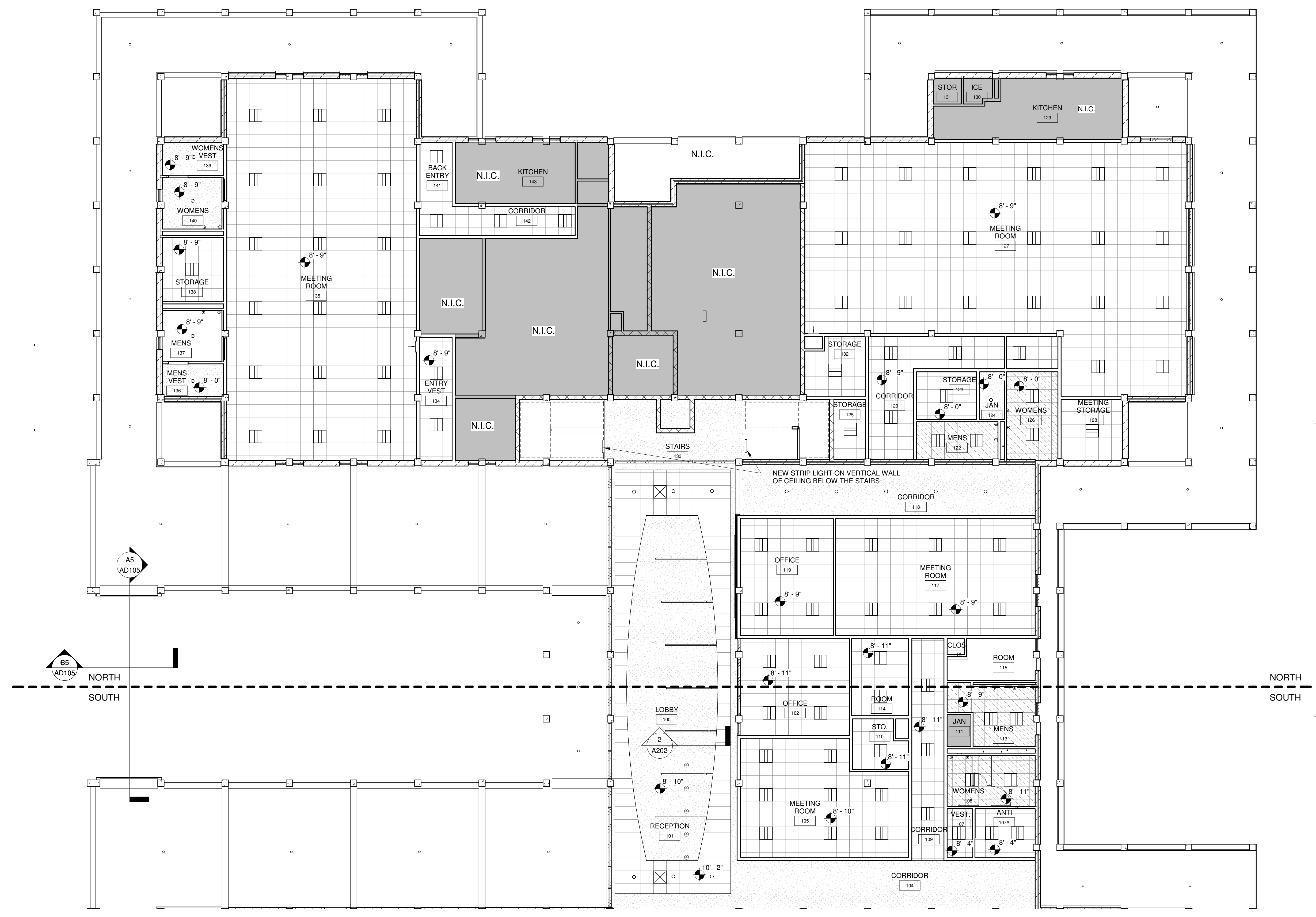
1 GROUND FLOOR PLAN - CEILING - RENOVATION - NORTH 1/8" = 1'-0"
