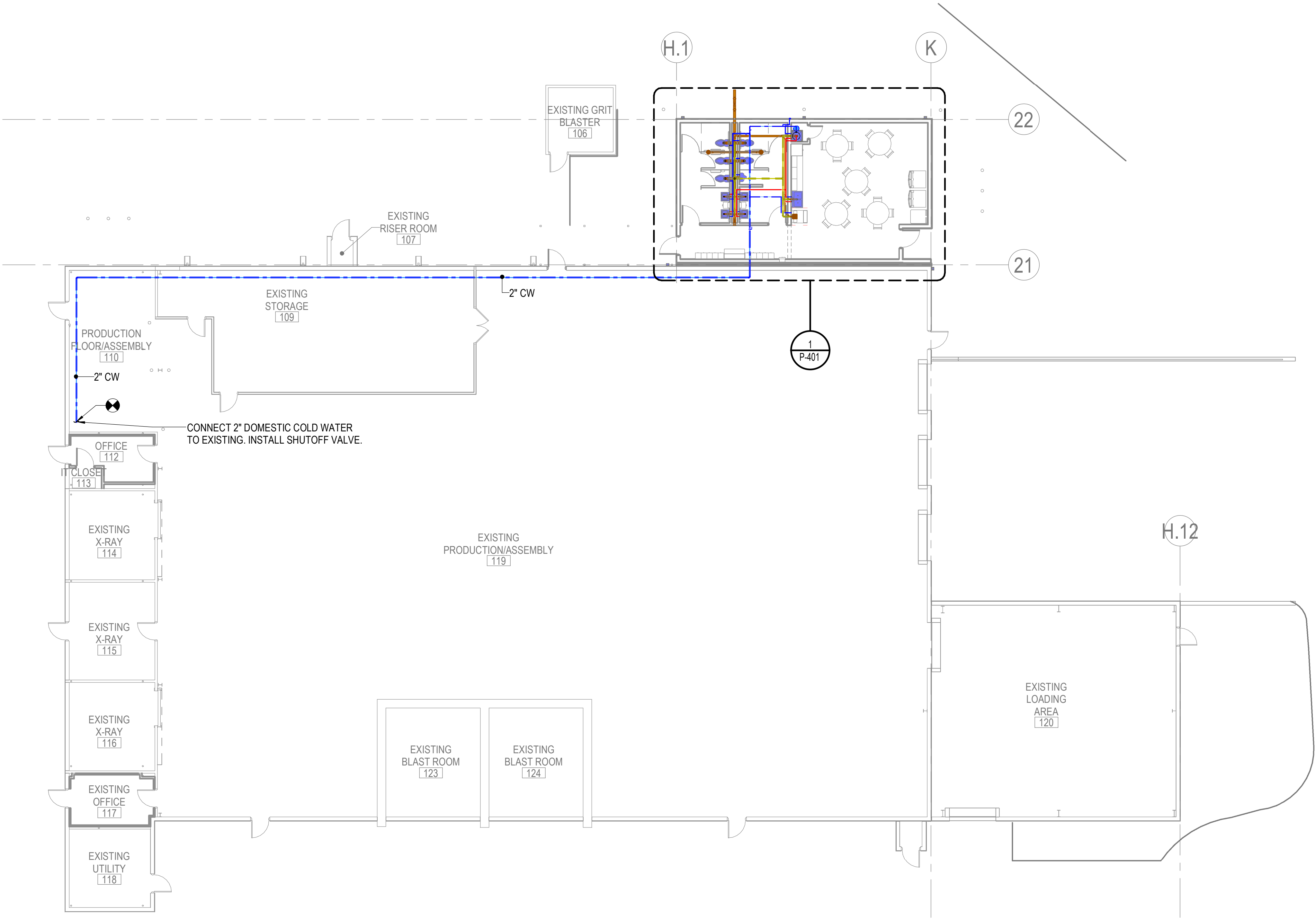
1 PLUMBING OVERALL PLAN 3/32" = 1'-0"
