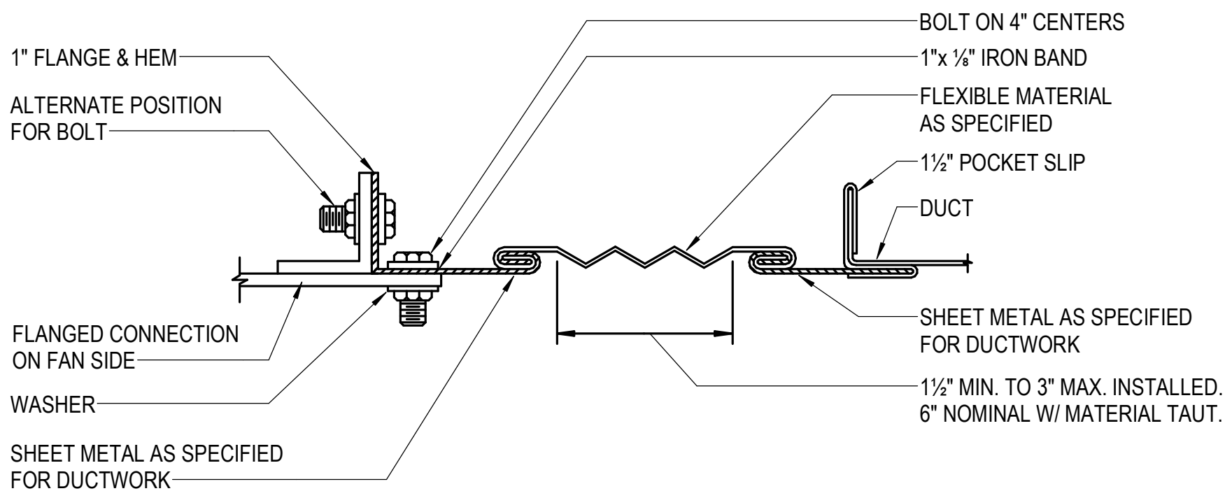
2 FLEXIBLE CONNECTION RECTANGULAR NOT TO SCALE
