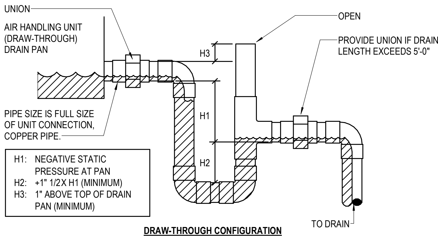
3 CONDENSATE PIPING - DRAIN TRAP - DRAW THROUGH 1/8" = 1'-0" 0 8 16 32
