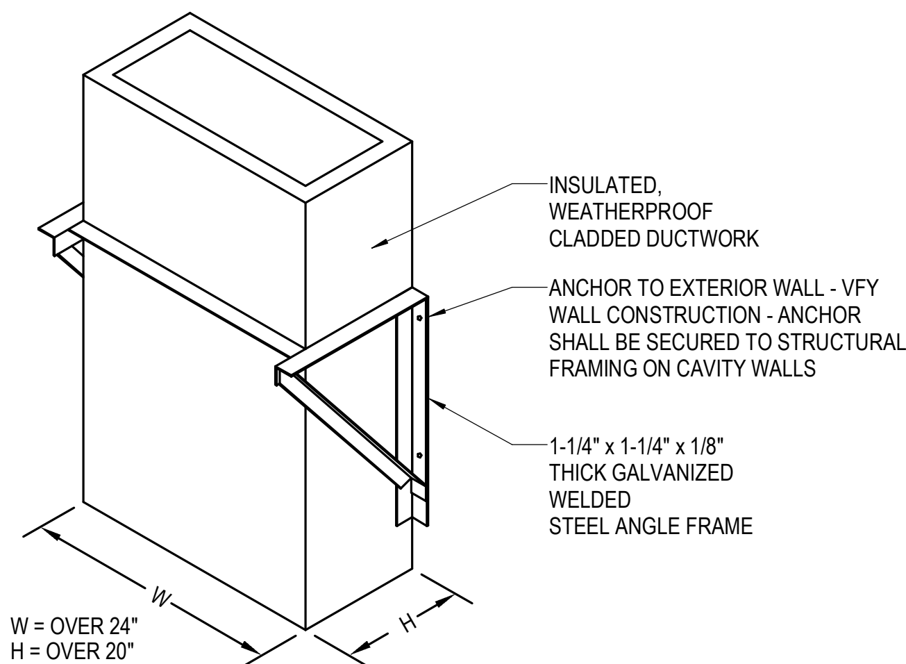
5 EXTERIOR VERTICAL RECTANGULAR DUCT SUPPORT NOT TO SCALE
