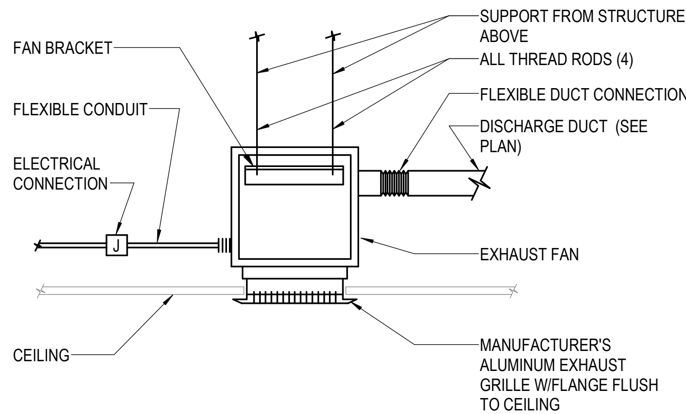
4 CEILING MOUNTED EXHAUST FAN NOT TO SCALE
