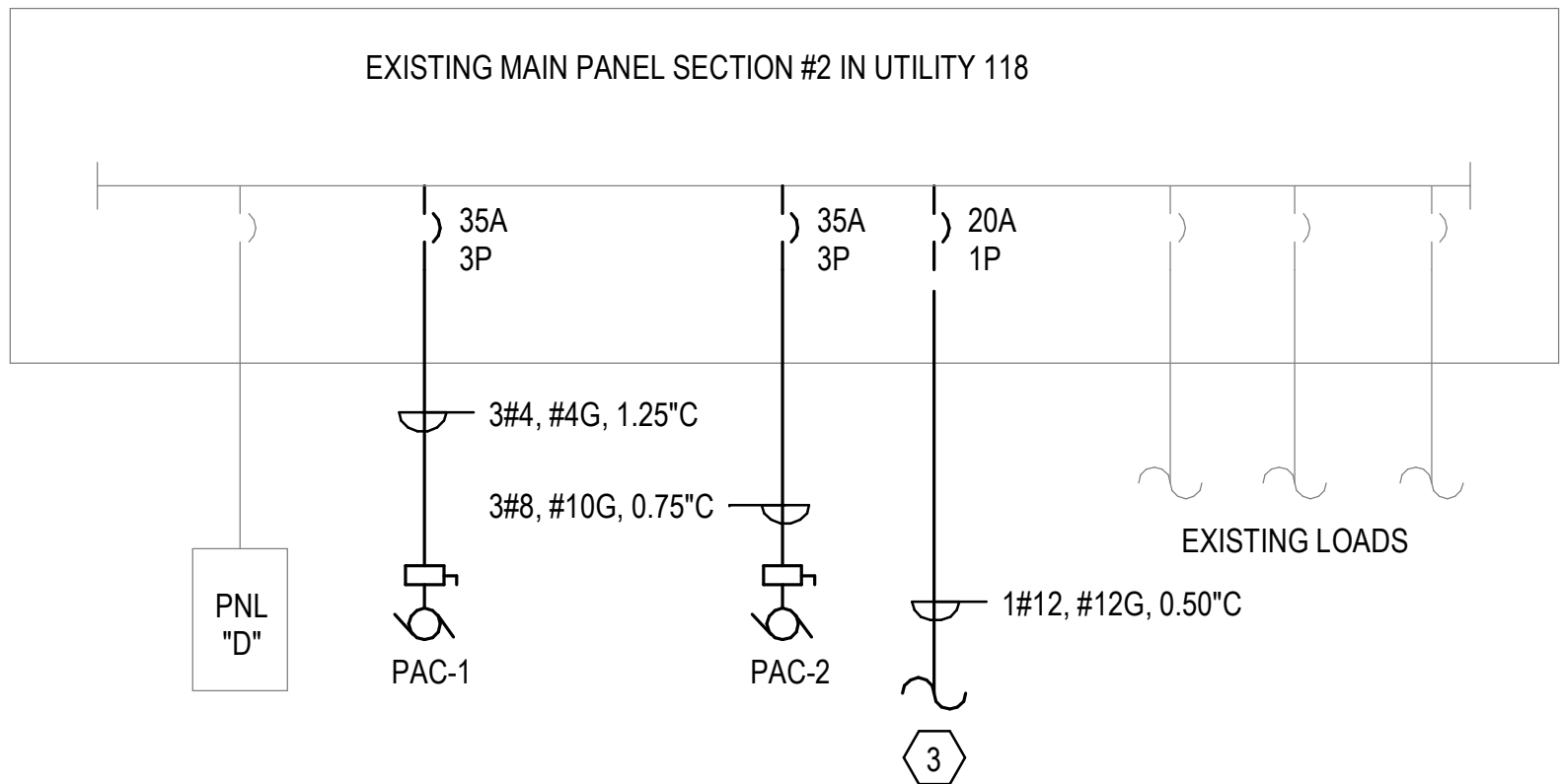
2 PARTIAL SINGLE - LINE DIAGRAM - UTILITY 118 N.T.S.
