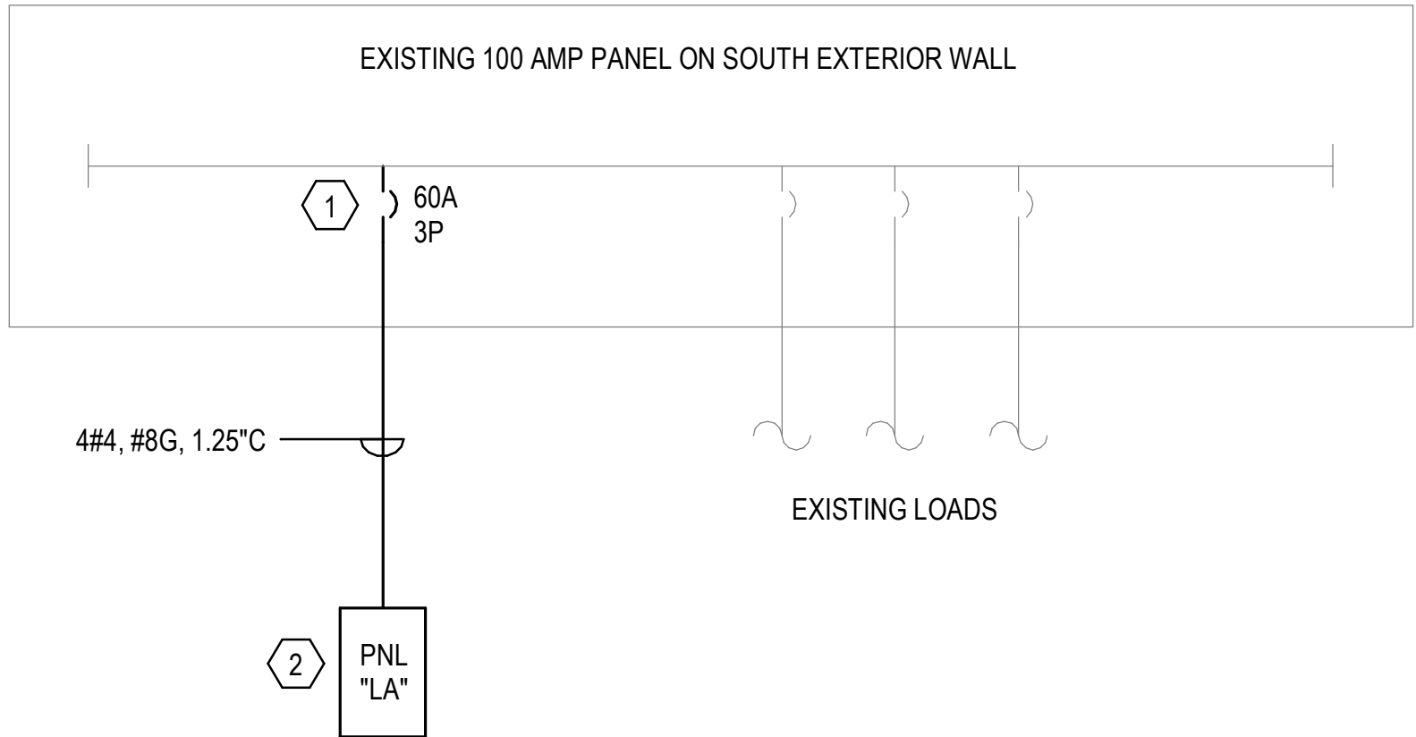
1 PARTIAL SINGLE - LINE DIAGRAM - NEW BREAK ROOM N.T.S.
