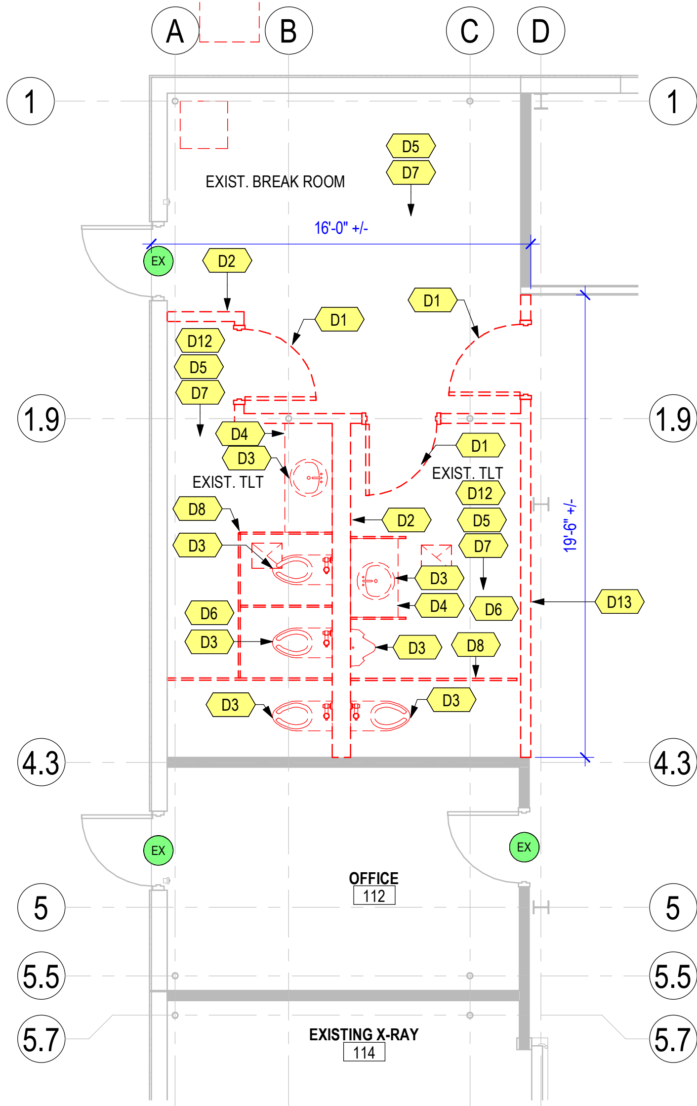
1 AREA C DEMOLITION PLAN
