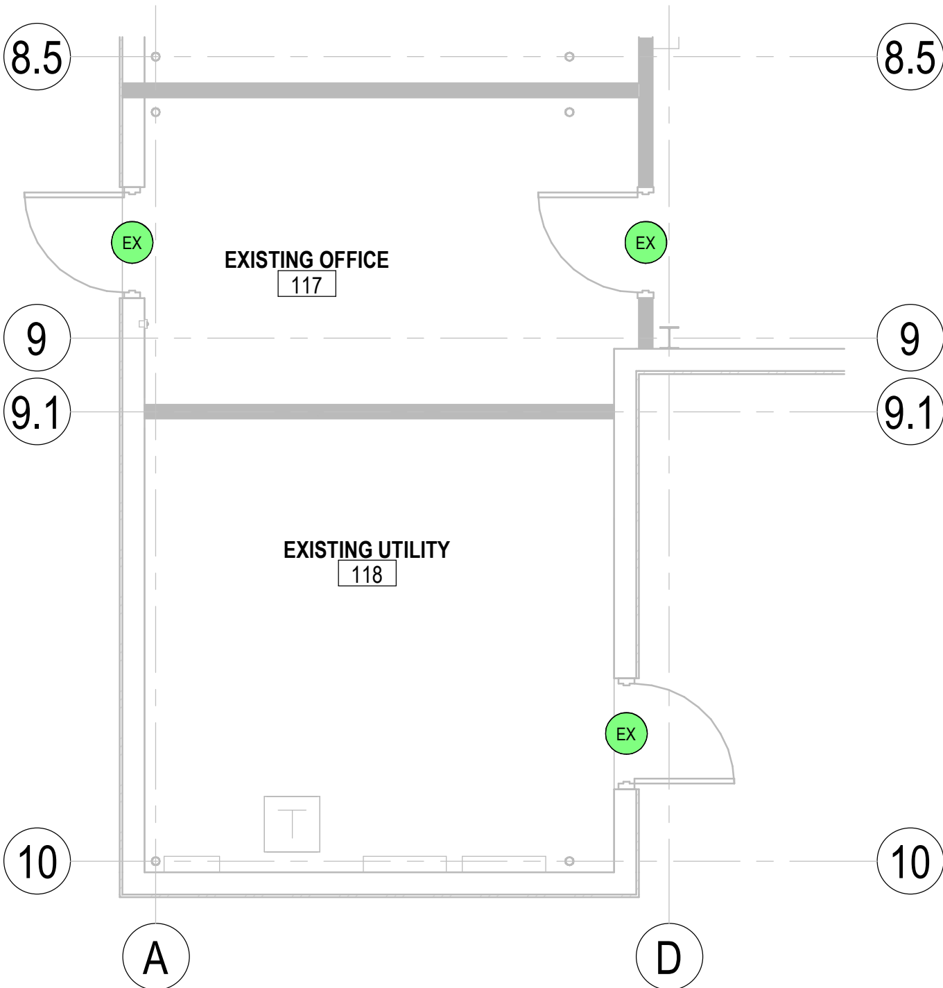
2 AREA D DEMOLITION PLAN
