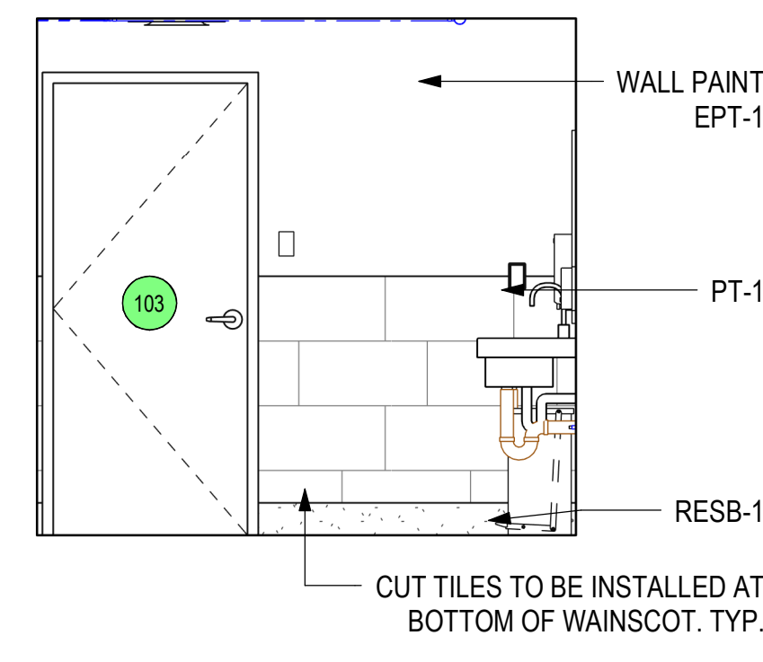
7 MN TLT 103 - NORTH 3/8" = 1'-0"
