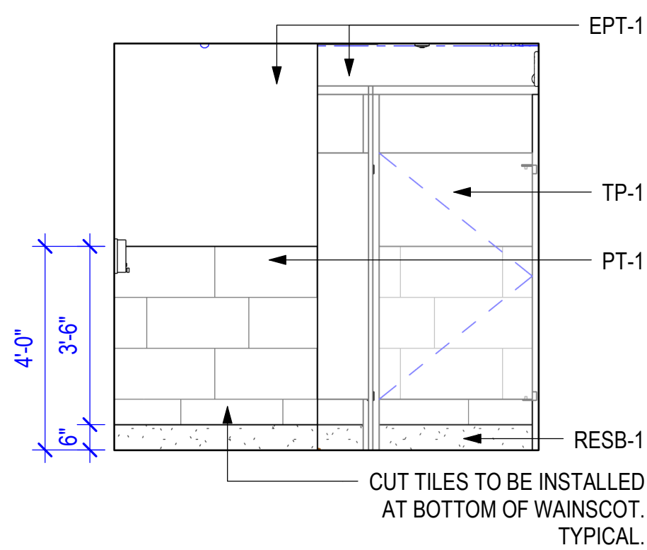
5 MN TLT 103 - SOUTH 3/8" = 1'-0"
