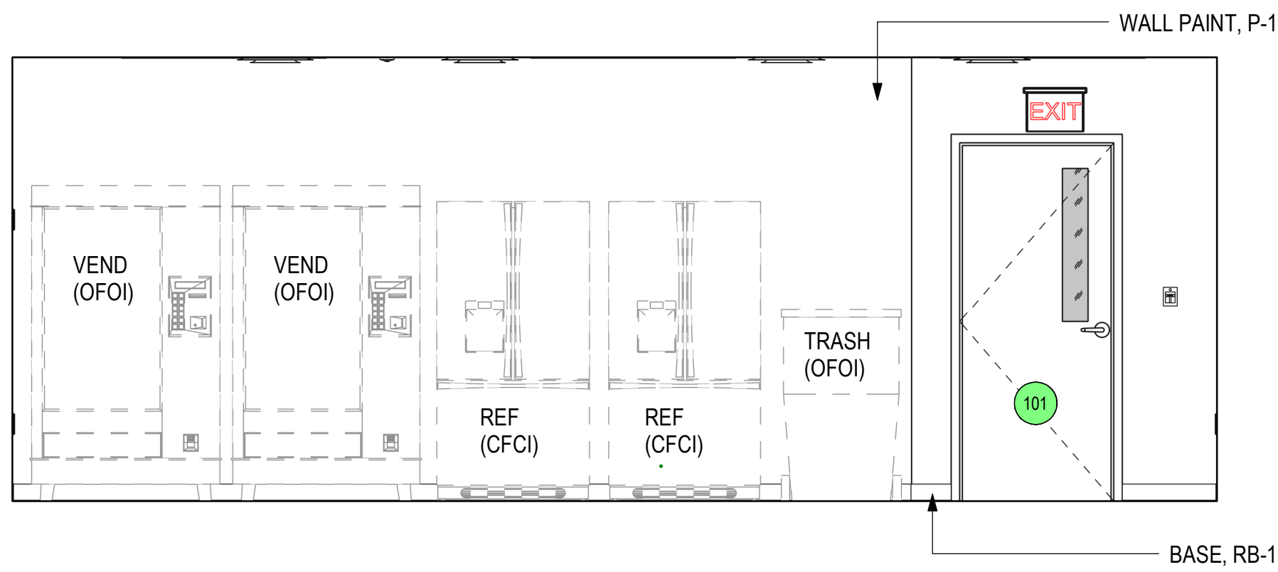
2 BREAK ROOM 101 - WEST 3/8" = 1'-0"
