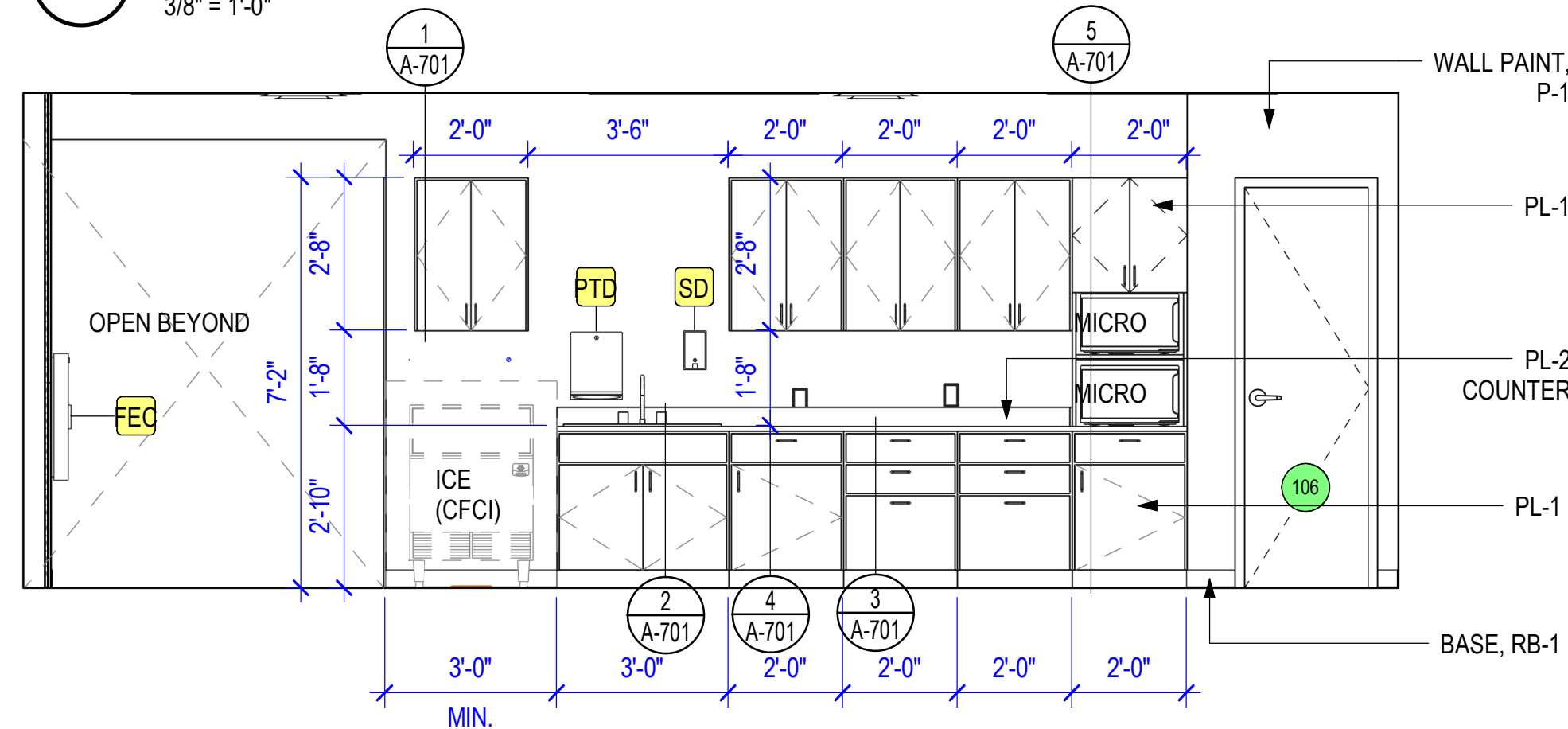
4 BREAK ROOM 101 - EAST 3/8" = 1'-0"
