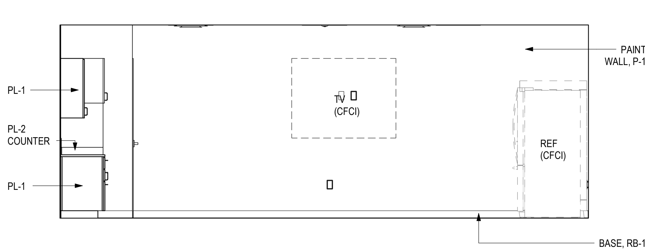
1 BREAK ROOM 101 - SOUTH 3/8" = 1'-0"
