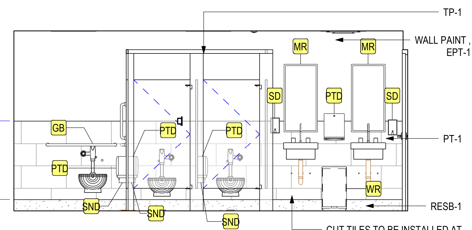
10 WM TLT 104 - WEST 3/8" = 1'-0"
