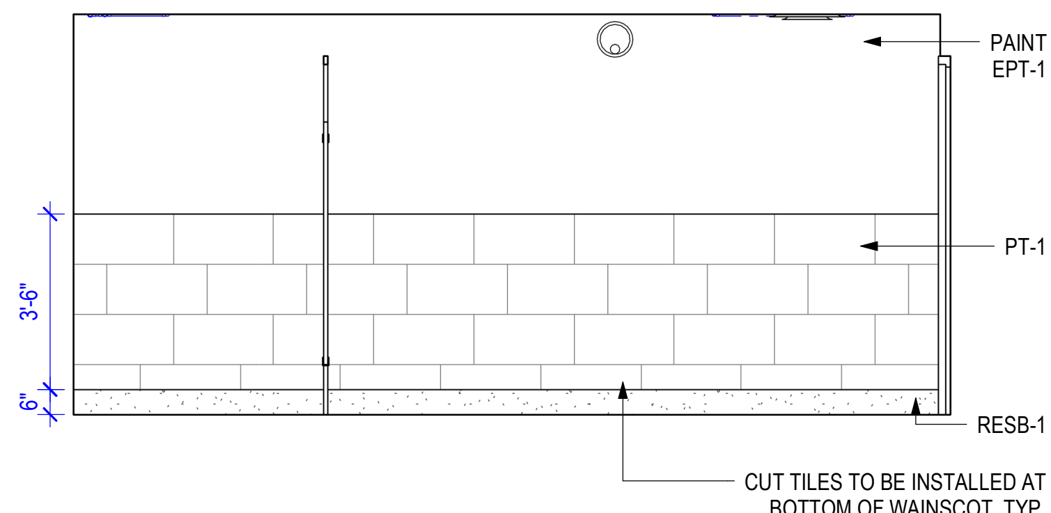
6 MN TLT 103 - WEST 3/8" = 1'-0"
