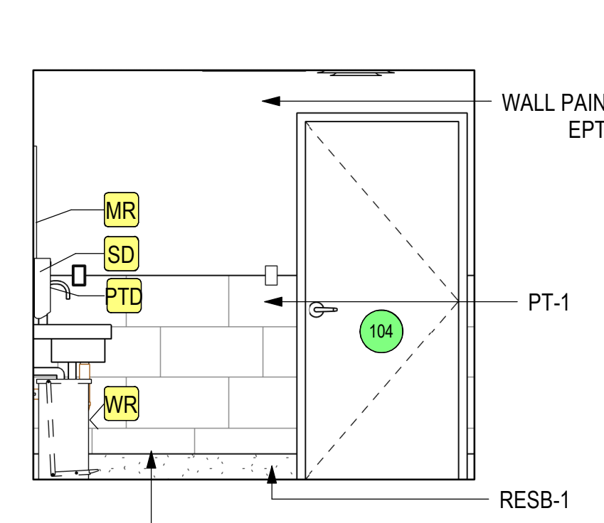
11 WM TLT 104 - NORTH 3/8" = 1'-0"
