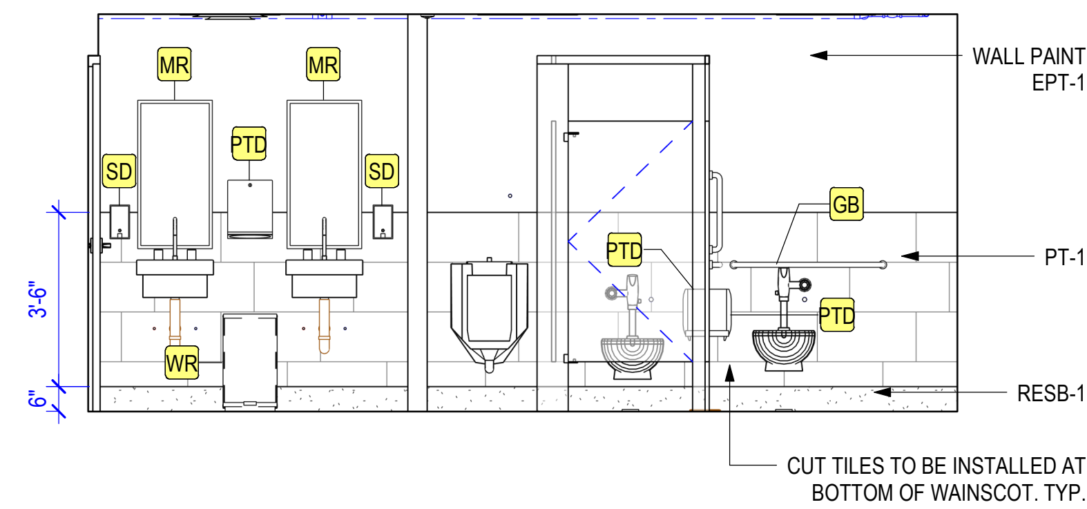
8 MN TLT 103 - EAST 3/8" = 1'-0"
