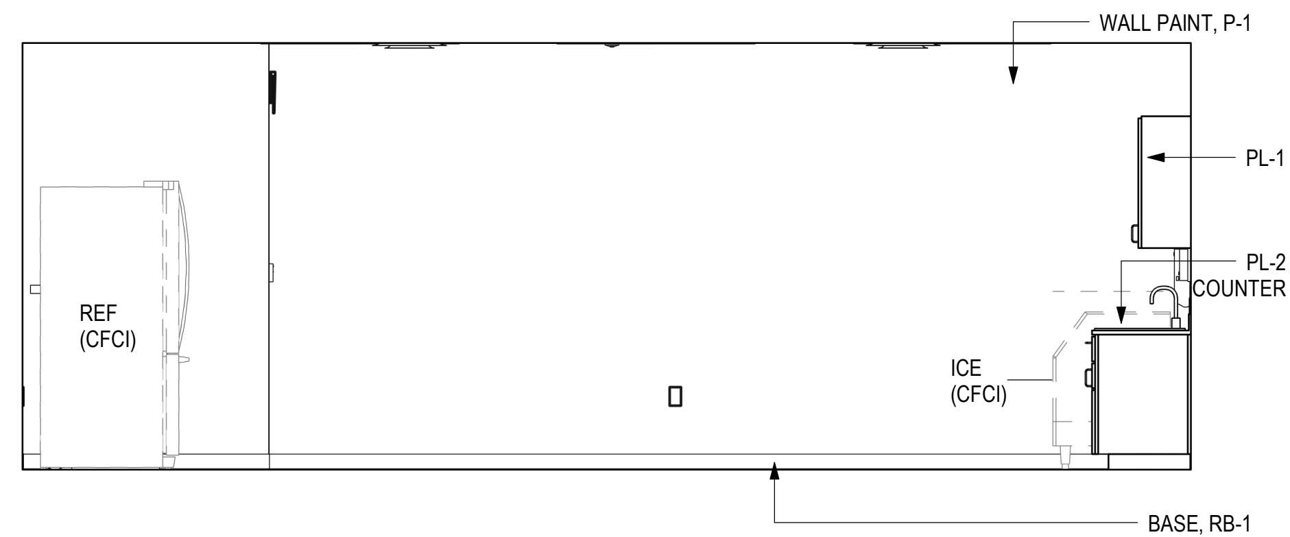
1 BREAK ROOM 101 - SOUTH 3/8" = 1'-0"
