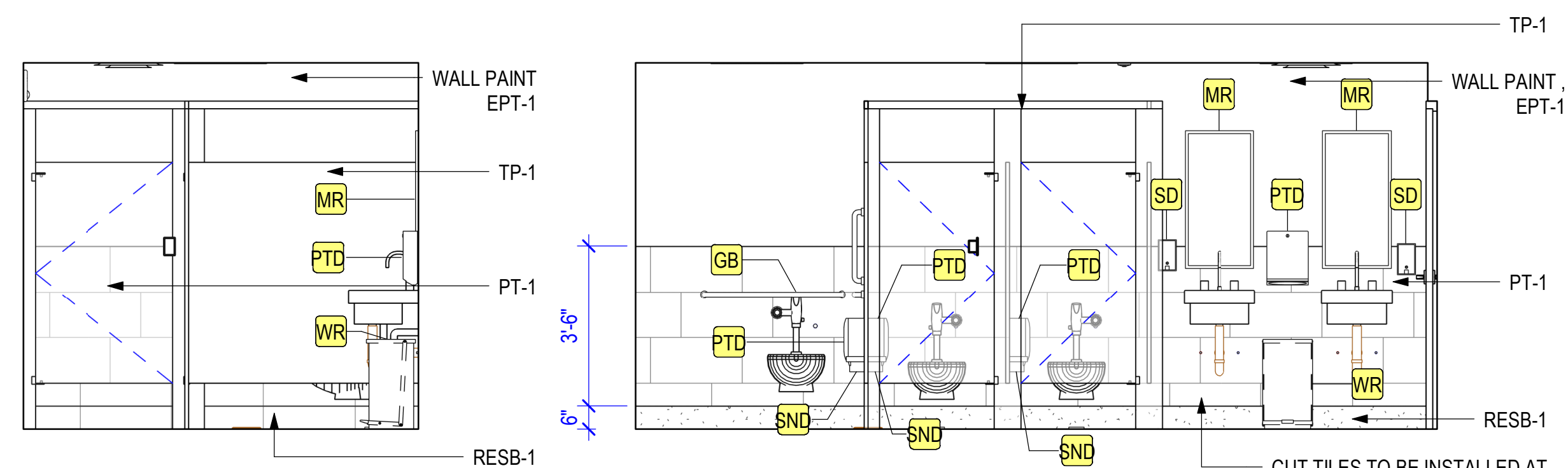
9 WM TLT 104 - SOUTH 3/8" = 1'-0"
