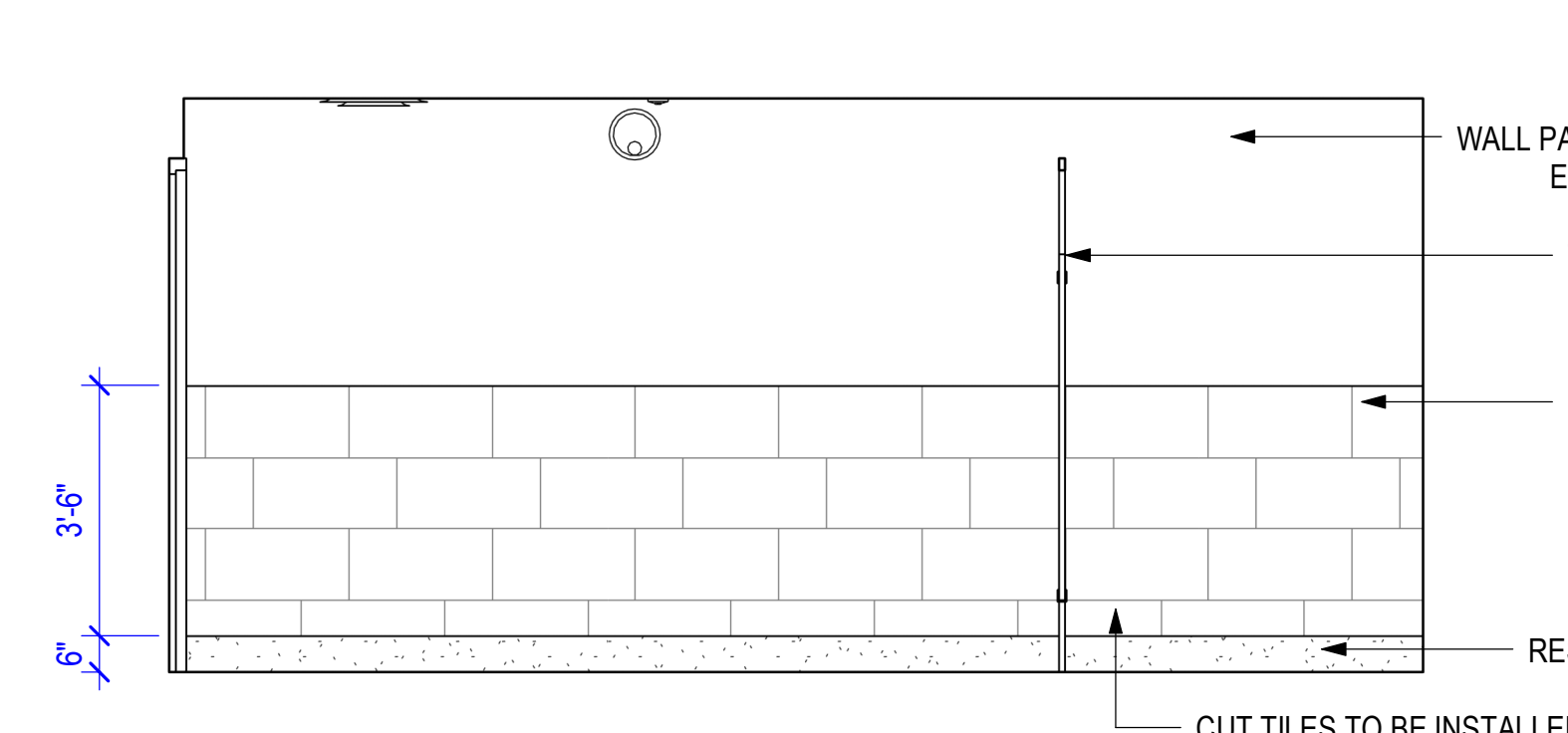
12 WM TLT - EAST 3/8" = 1'-0"
