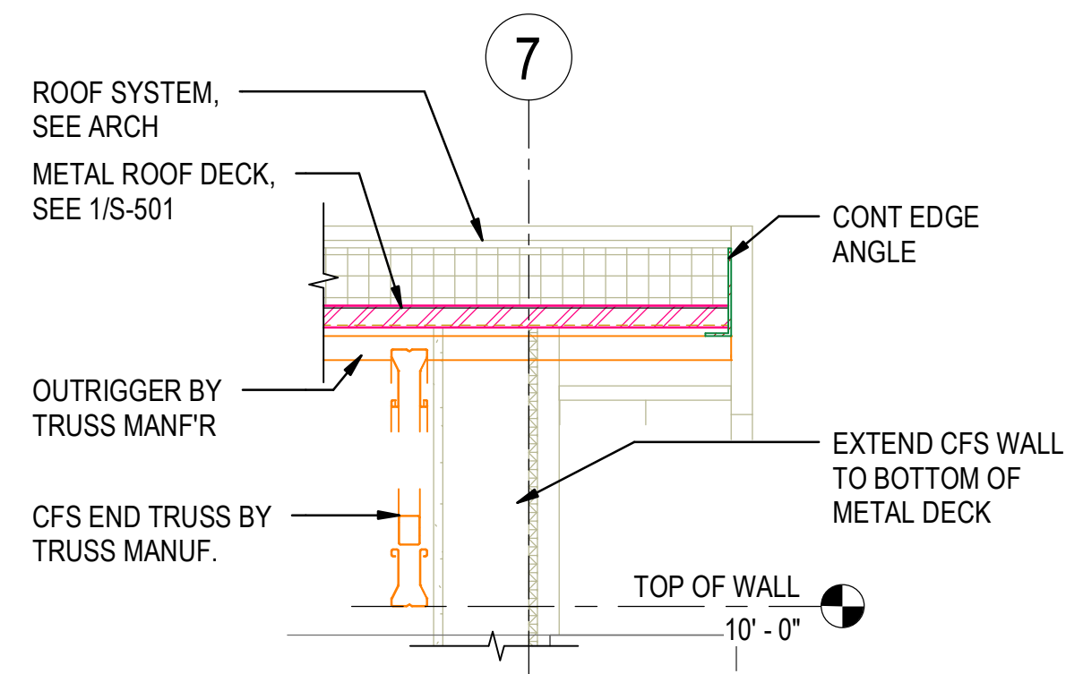
1 ENDWALL TRUSS TO LOAD BEARING WALL 1" = 1'-0"
