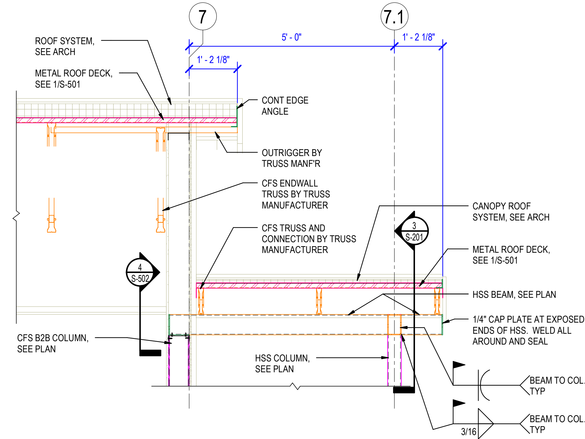
3 CANOPY FRAMING 3/4" = 1'-0"
