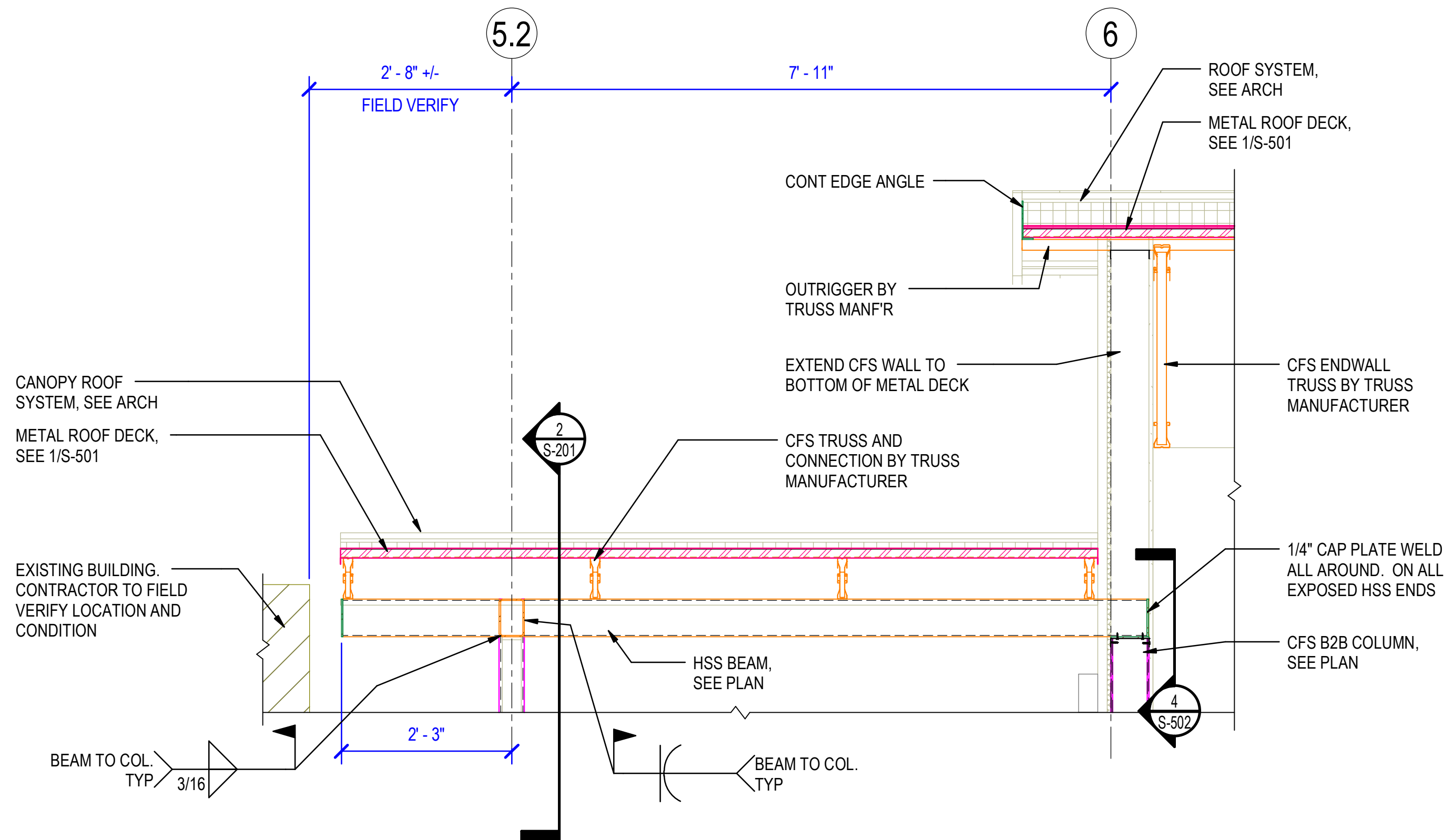
2 CANOPY FRAMING BETWEEN EXISTING BUILDING AND NEW BUILDING 3/4" = 1'-0"
