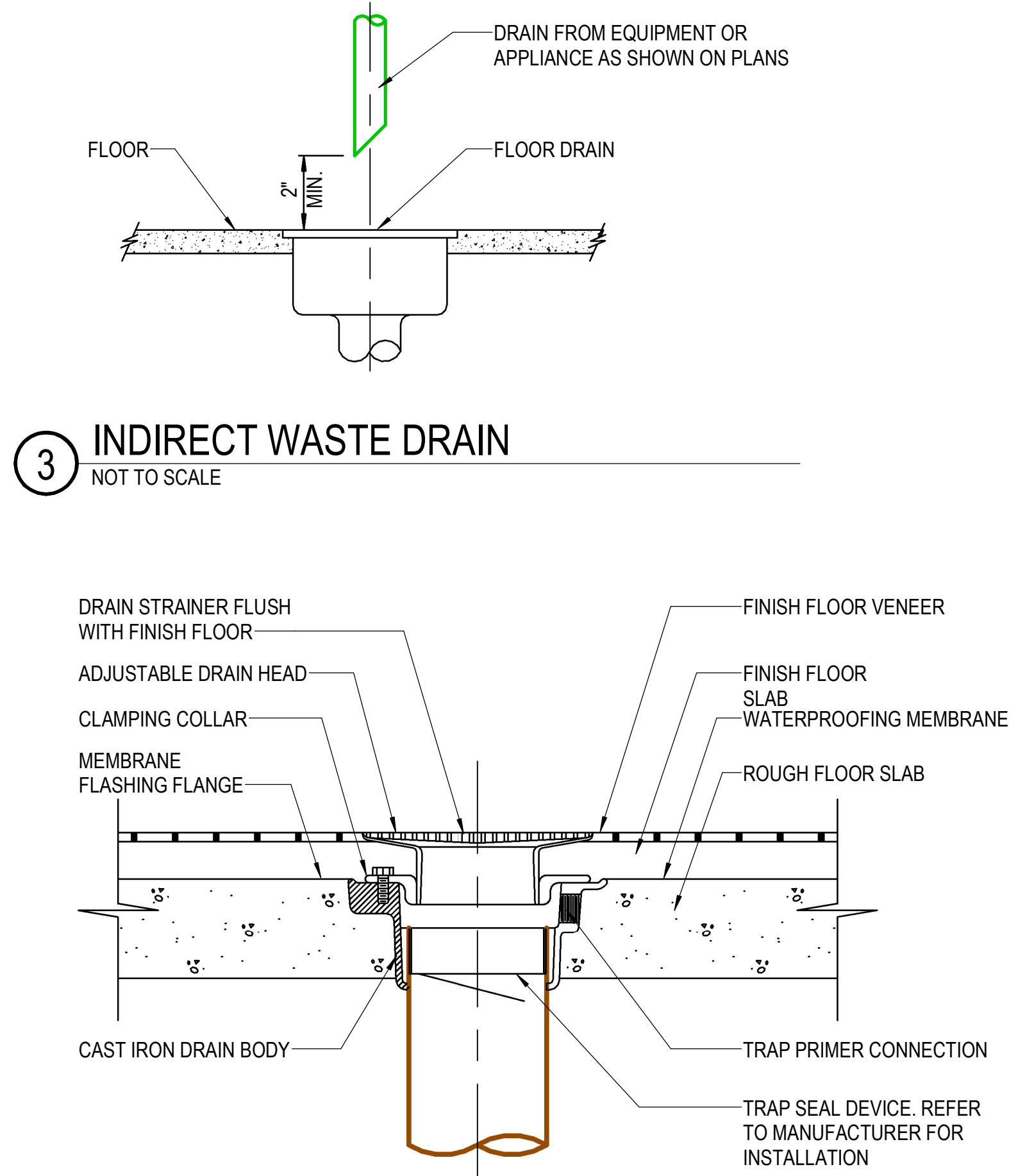
4 TRAP SEAL DEVICE INSTALLATION NOT TO SCALE
