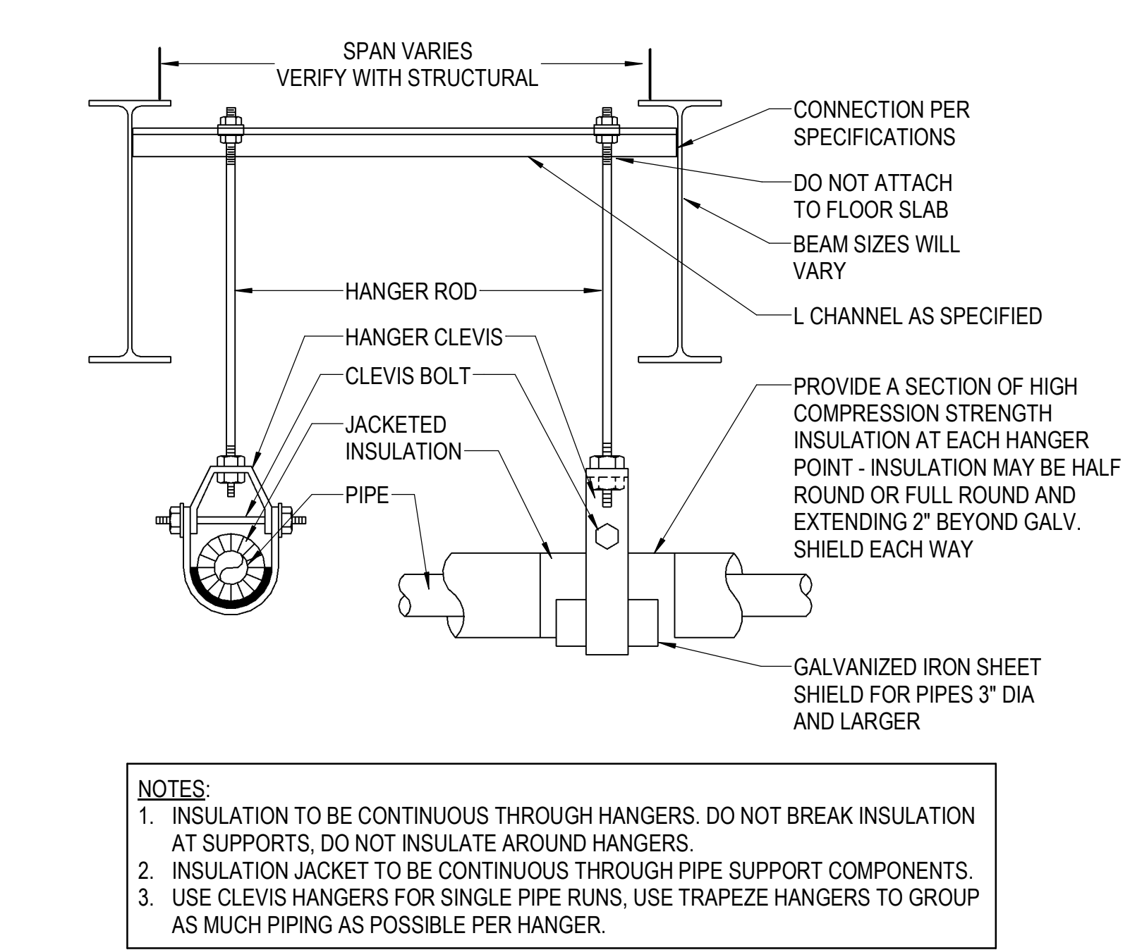
1 ADJUSTABLE CLEVIS HANGER NOT TO SCALE
