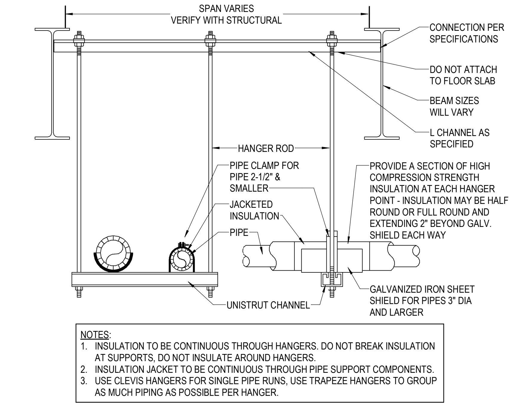
2 TRAPEZE PIPE HANGER NOT TO SCALE
