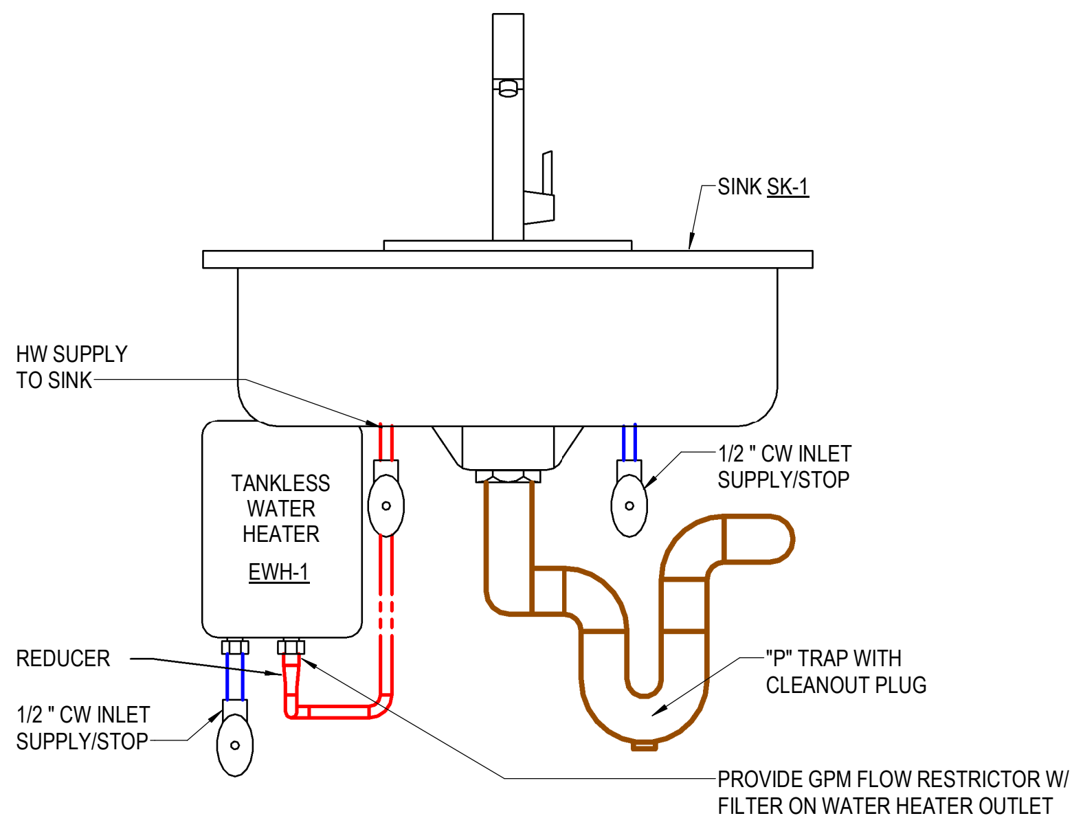
3 WATER HEATER INSTALLATION - EWH-1 NOT TO SCALE
