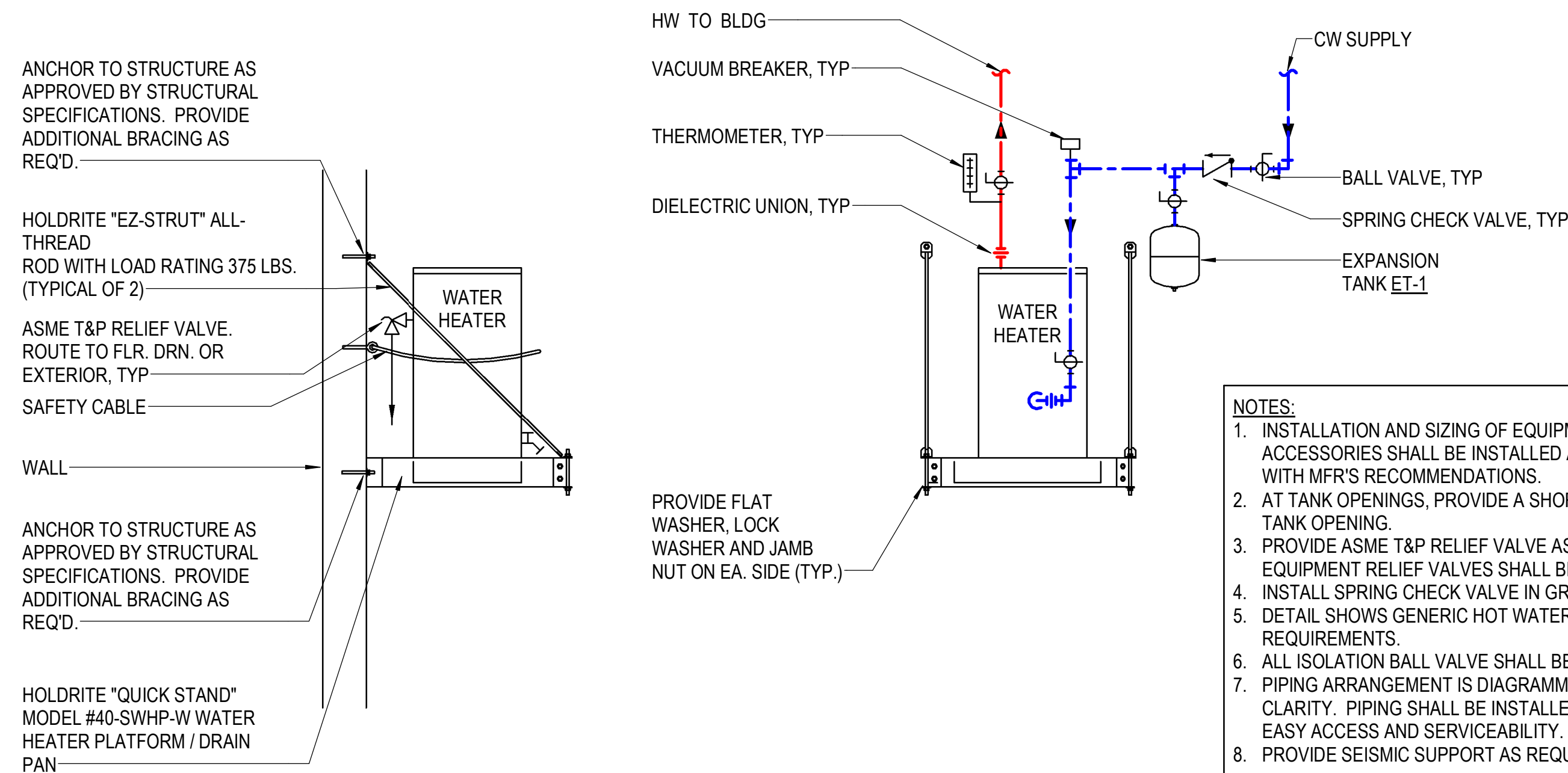
4 WATER HEATER INSTALLATION - EWH-2 NOT TO SCALE
