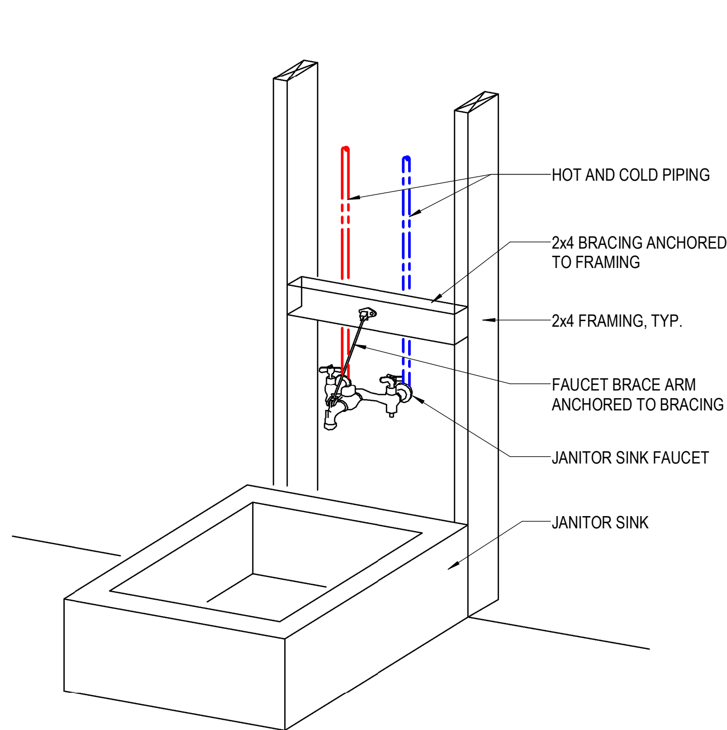
2 JANITOR SINK FAUCET BRACING NOT TO SCALE
