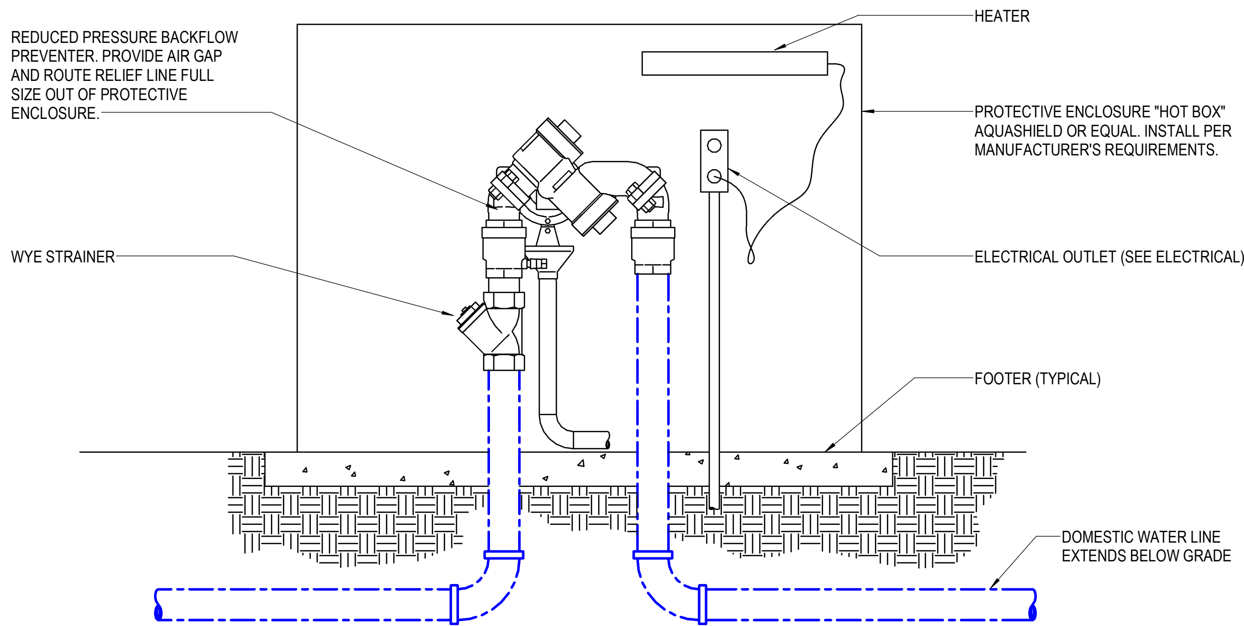
1 DOMESTIC WATER BUILDING SERVICE NOT TO SCALE
