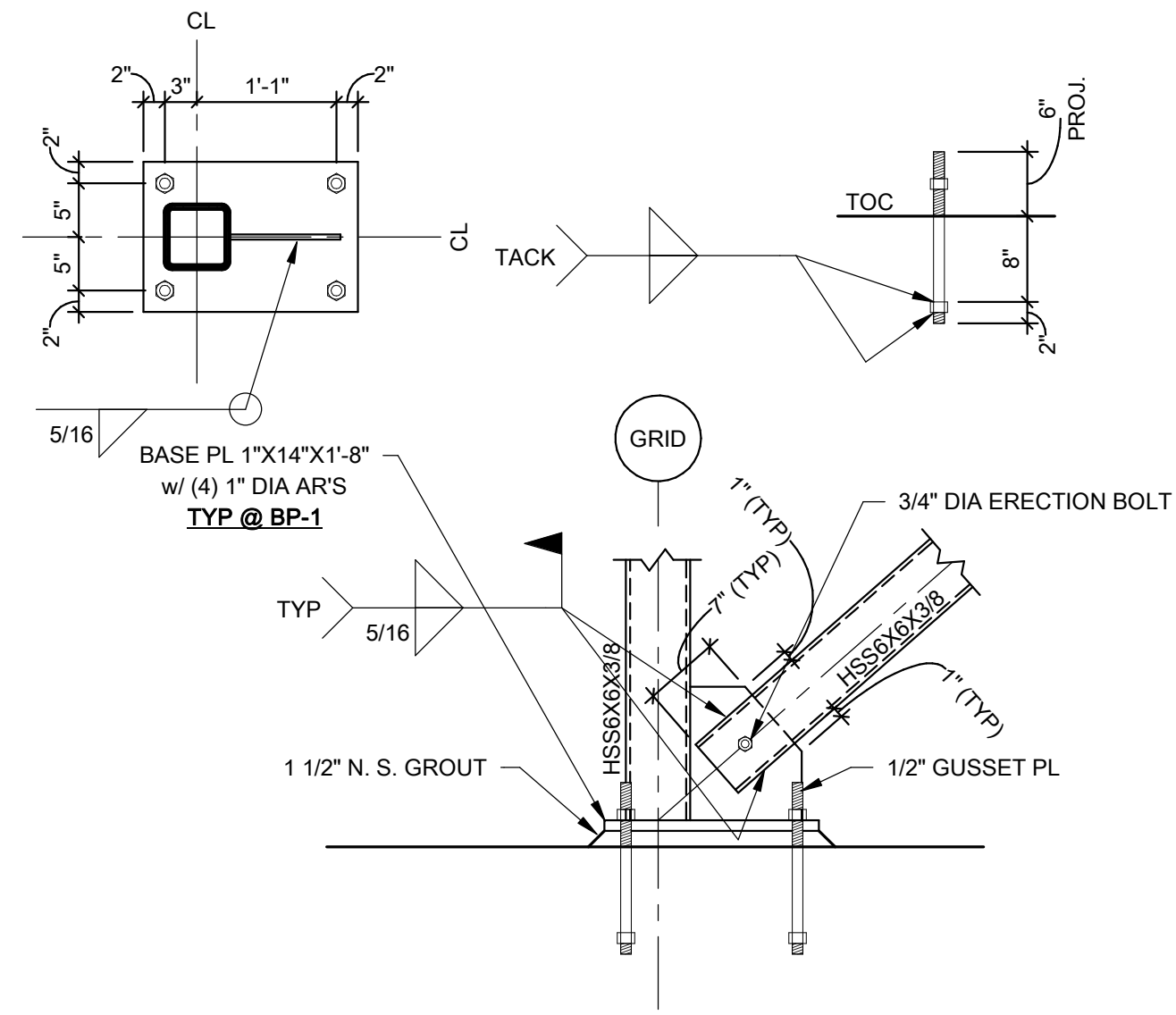
1 SECTION 3/4" = 1'-0"
