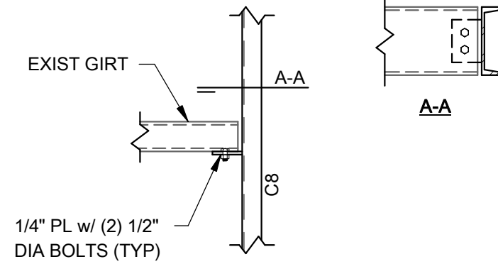
5 SECTION 3/4" = 1'-0"
