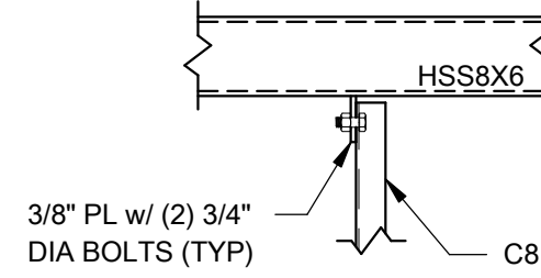
4 SECTION 3/4" = 1'-0"
