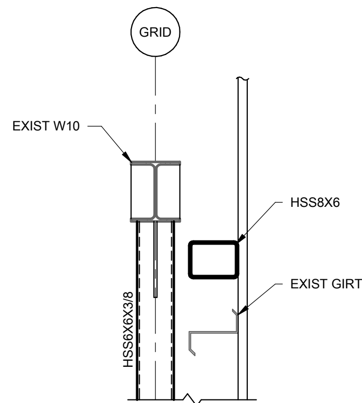
7 SECTION 3/4" = 1'-0"
