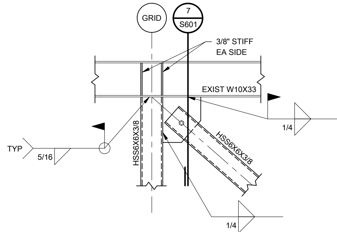
2 SECTION 3/4" = 1'-0"
