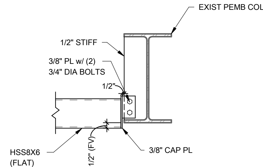
6 PLAN VIEW 3/4" = 1'-0"
