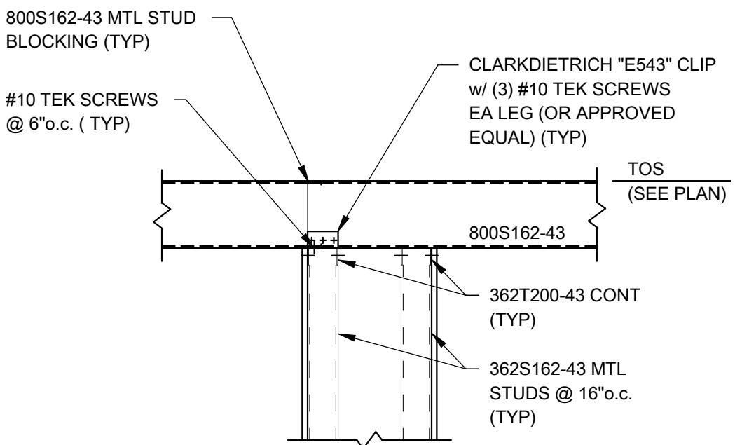
3 SECTION 3/4" = 1'-0"
