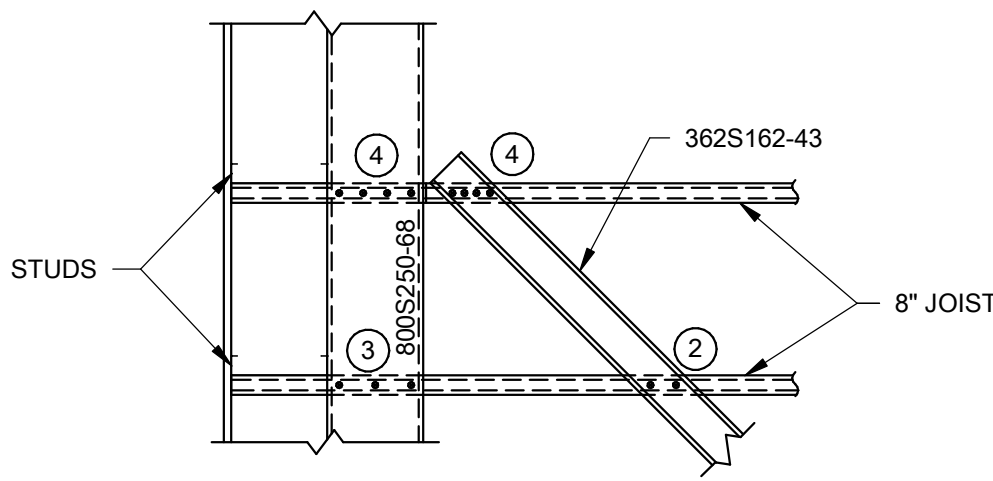
9 SECTION 3/4" = 1'-0"
