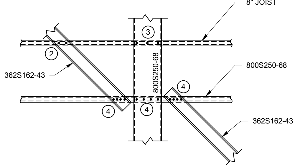
10 SECTION 3/4" = 1'-0"
