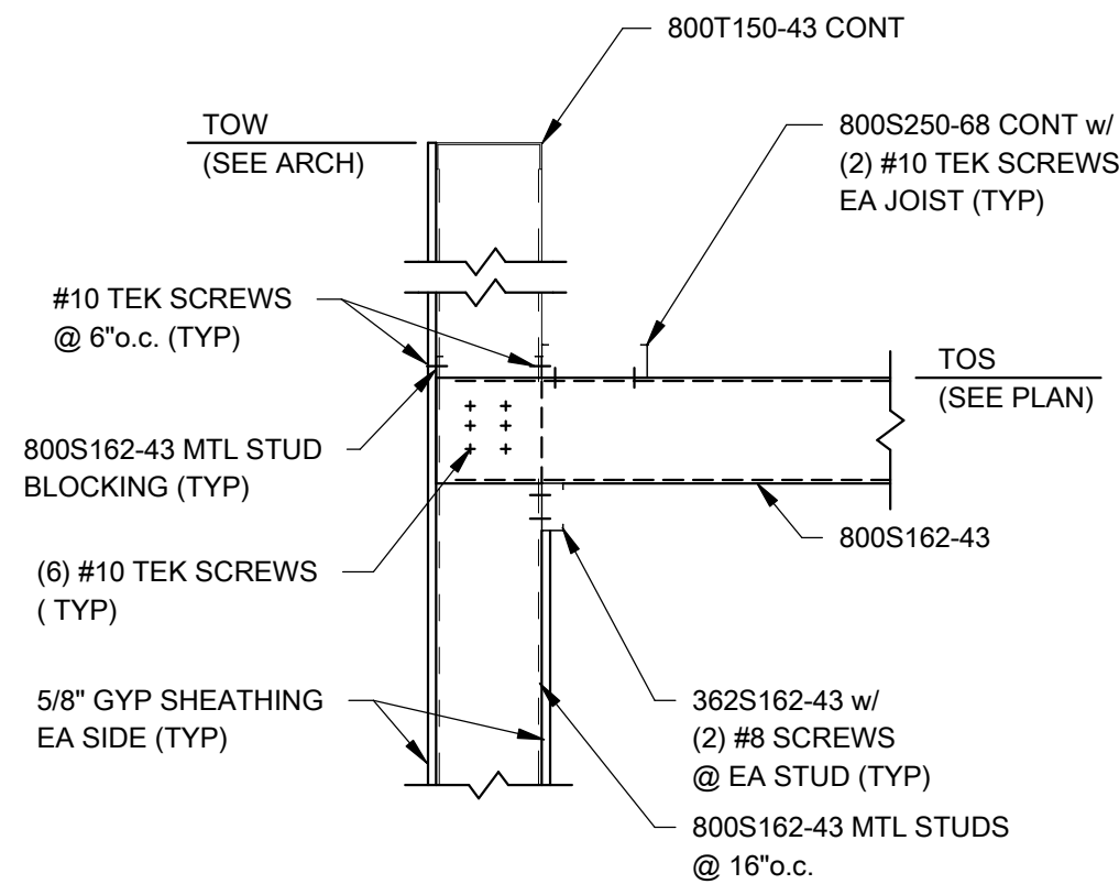
1 SECTION 3/4" = 1'-0"
