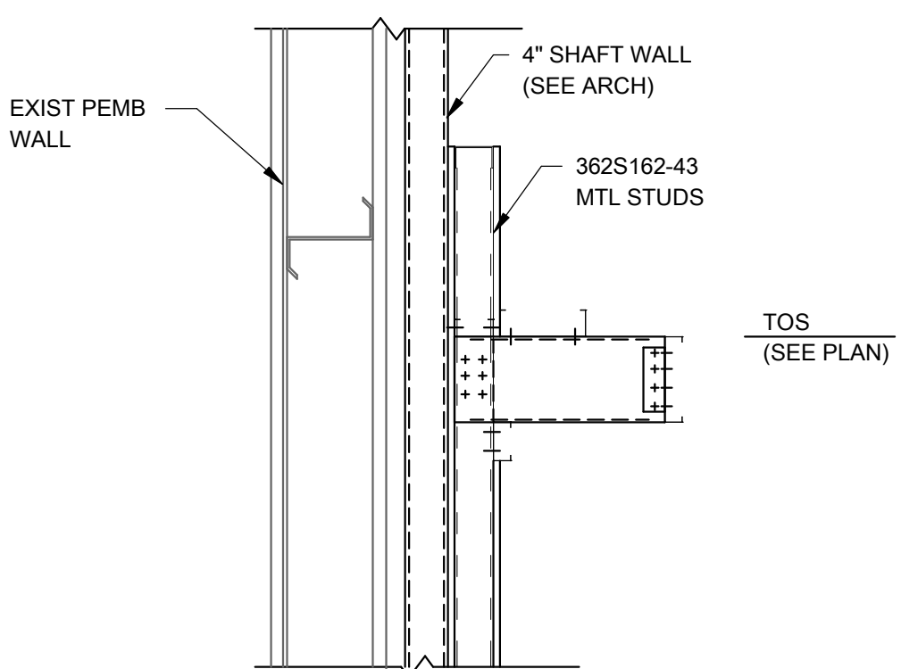
7 SECTION 3/4" = 1'-0"
