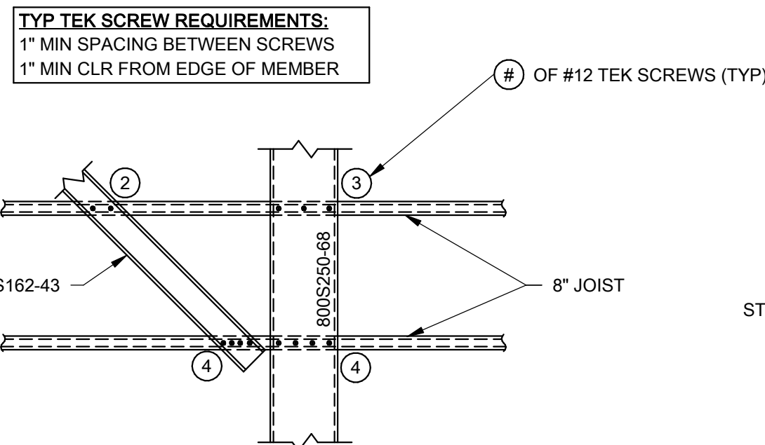
8 SECTION 3/4" = 1'-0"
