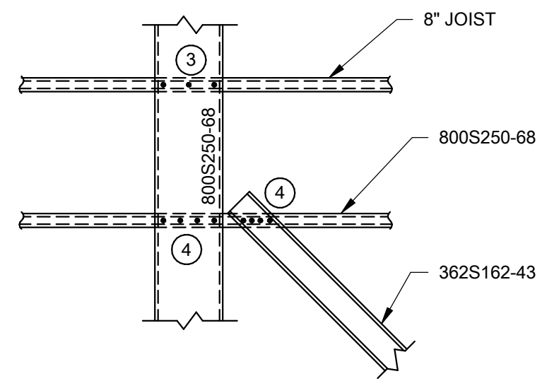
11 SECTION 3/4" = 1'-0"
