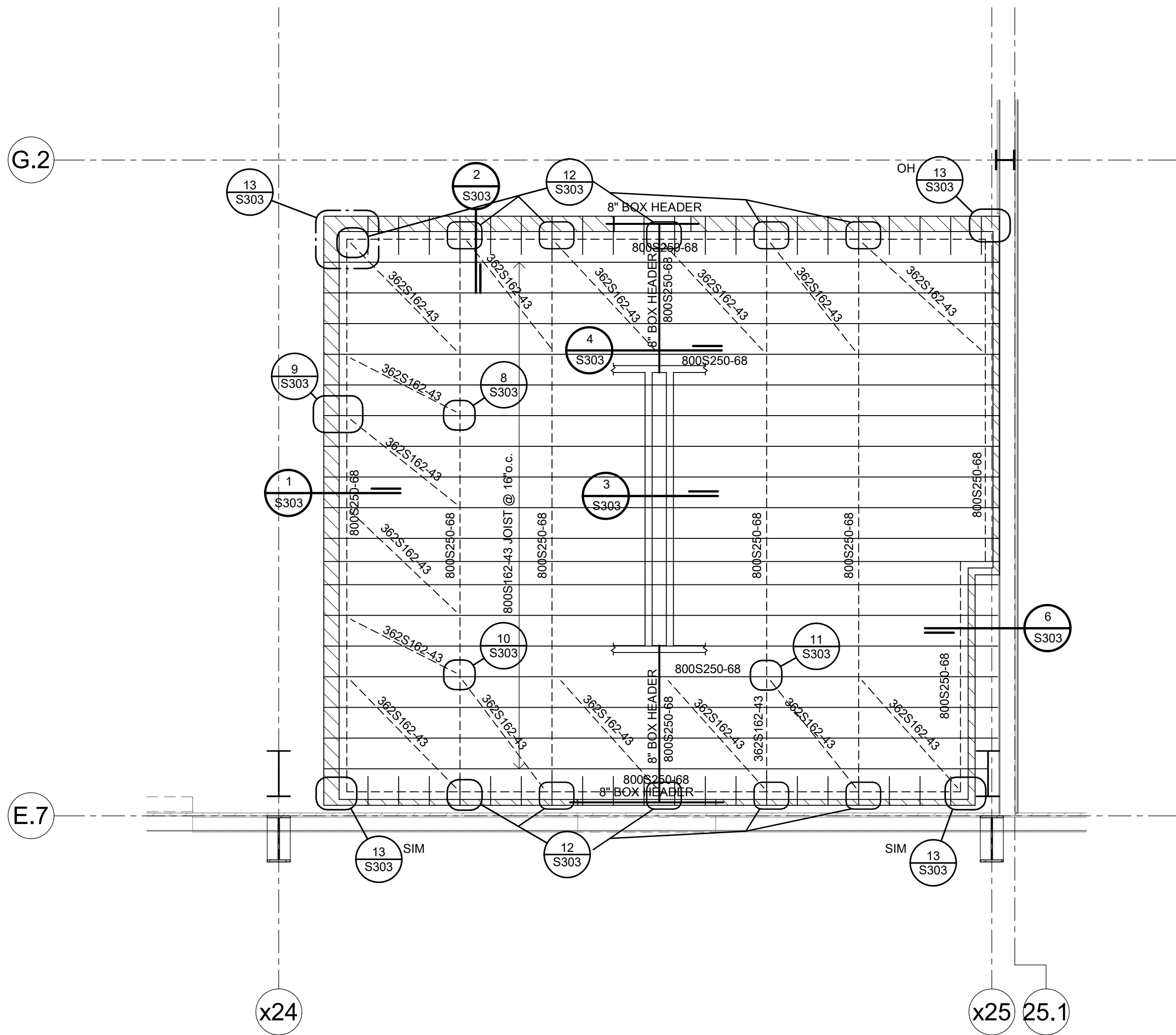
A BATHROOM FRAMING 1/4" = 1'-0"
