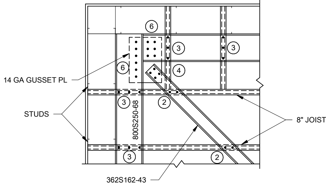
13 SECTION 3/4" = 1'-0"
