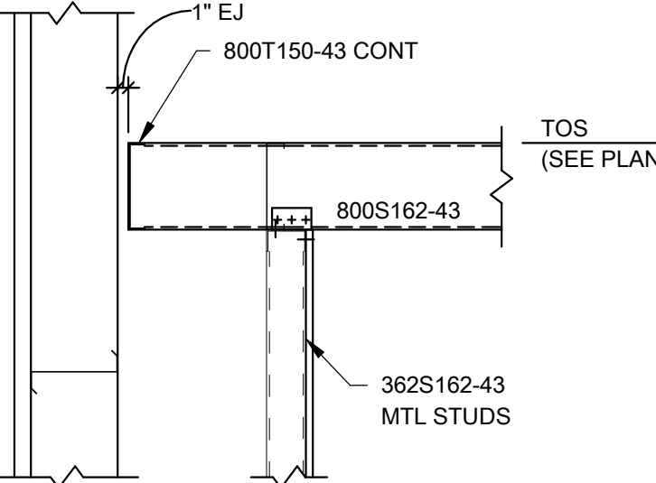
6 SECTION 3/4" = 1'-0"
