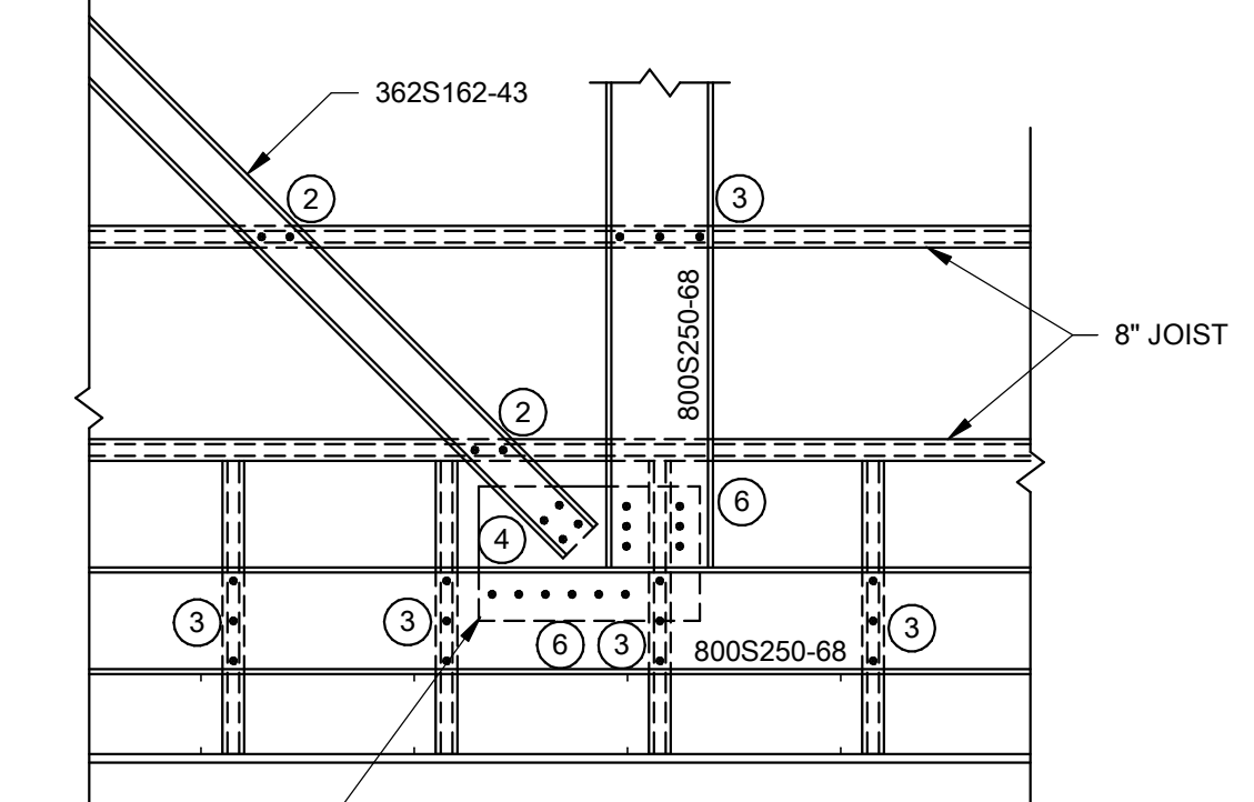
12 SECTION 3/4" = 1'-0"
