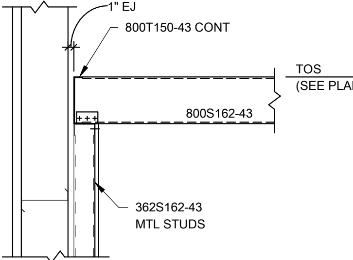
5 SECTION 3/4" = 1'-0"
