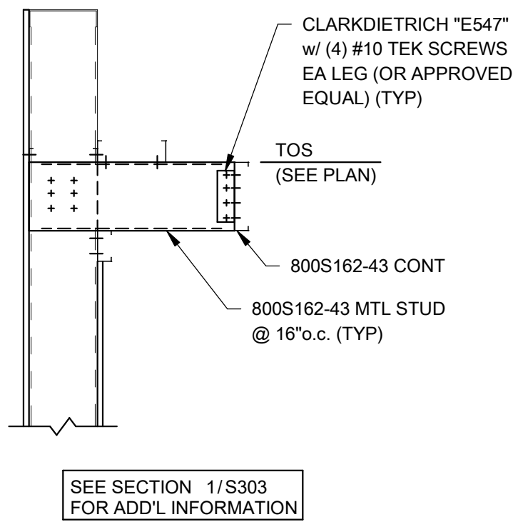
2 SECTION 3/4" = 1'-0"
