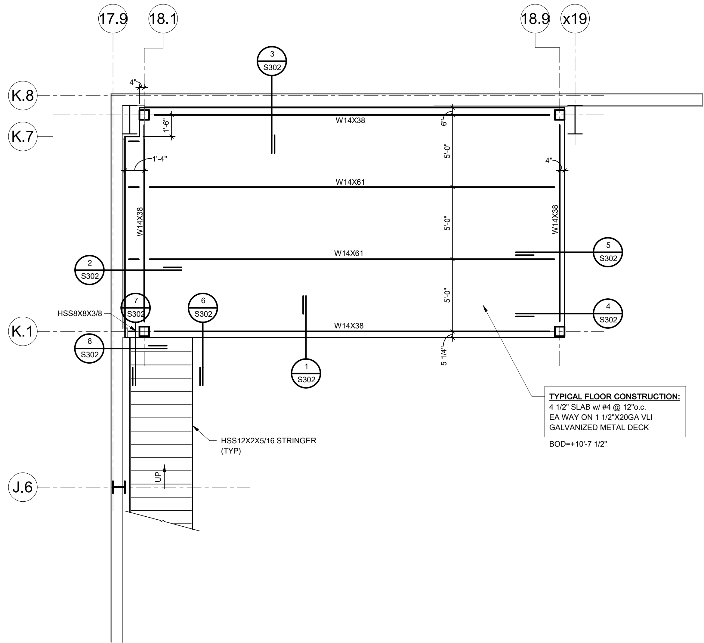
MEZZANINE FRAMING PLAN 1/4" = 1'-0"
