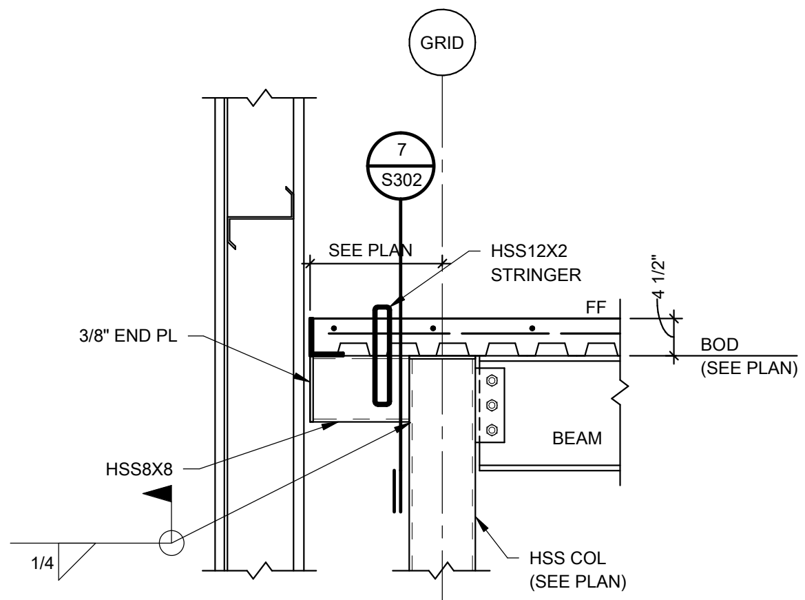
SECTION 8 3/4" = 1'-0"
