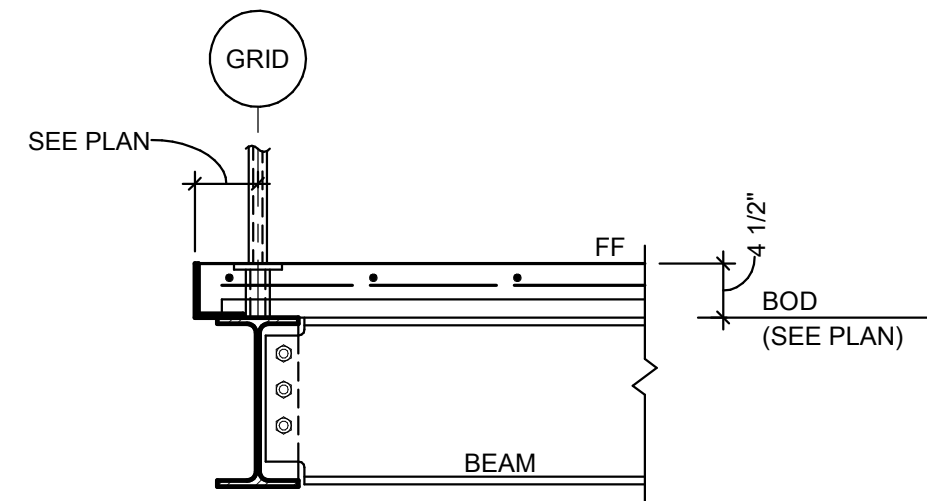
SECTION 5 3/4" = 1'-0"
