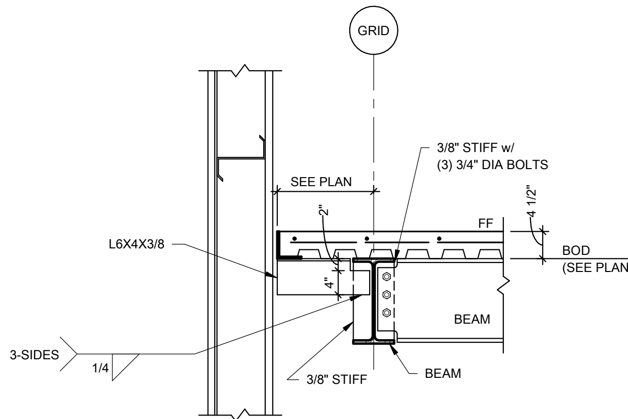
SECTION 2 3/4" = 1'-0"
