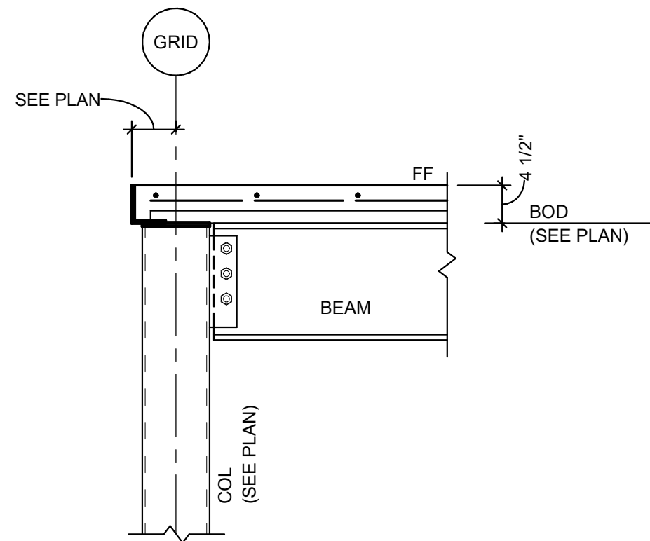
SECTION 4 3/4" = 1'-0"
