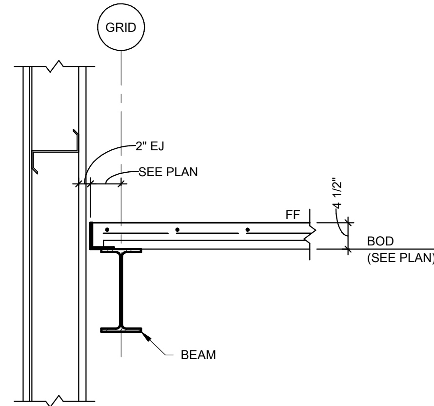
SECTION 1 3/4" = 1'-0"
