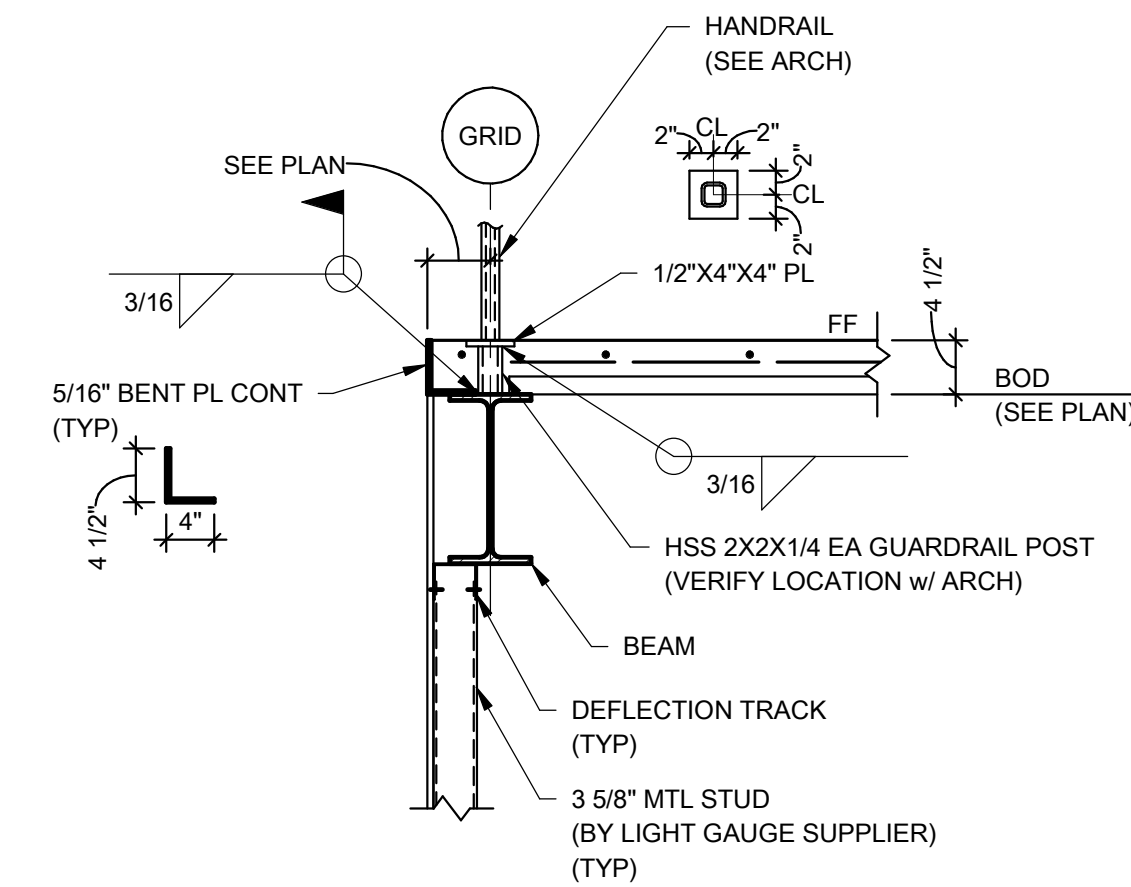
SECTION 1 3/4" = 1'-0"
