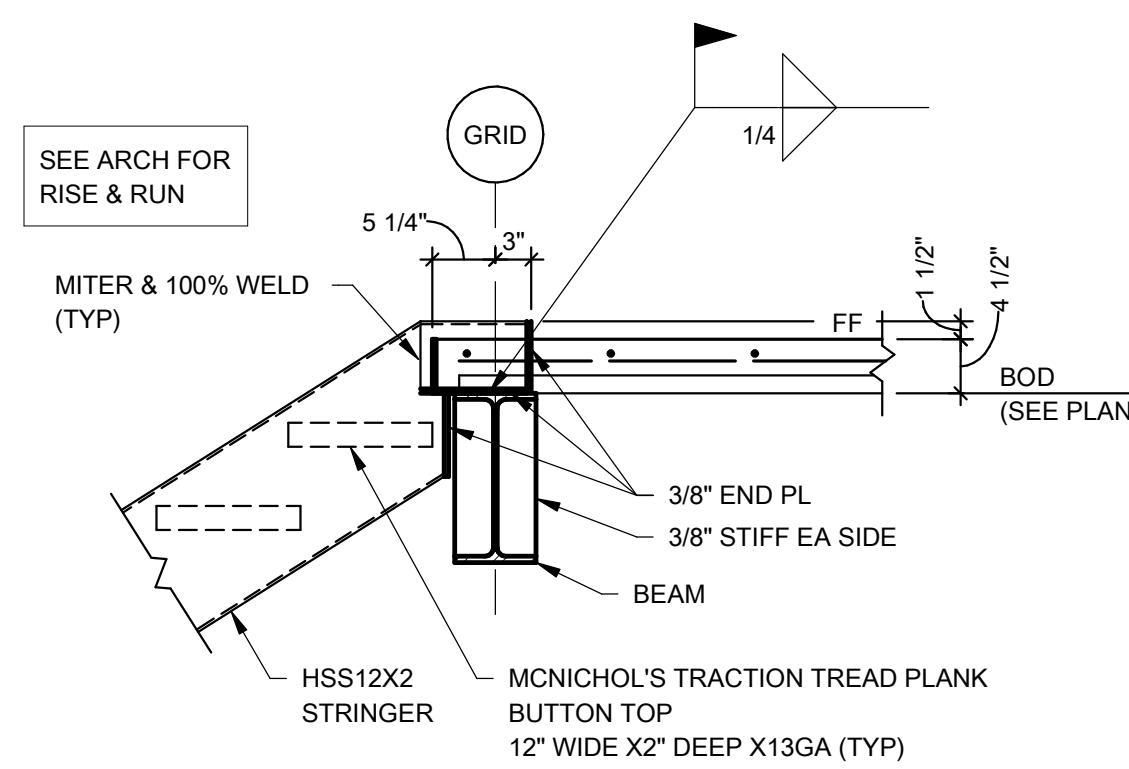
SECTION 6 3/4" = 1'-0"
