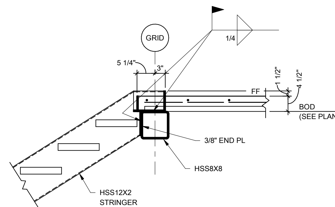
SECTION 7 3/4" = 1'-0"
