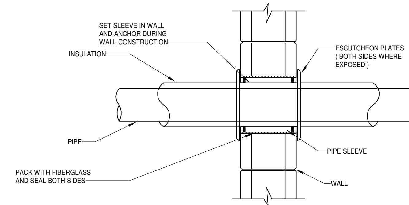
13 PIPE SLEEVE THRU INTERIOR WALL NOT TO SCALE:
