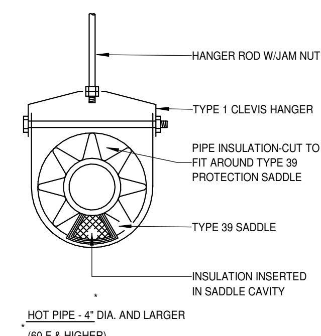
11 HANGER DETAILS: INSULATED PIPE DETAIL NOT TO SCALE:
