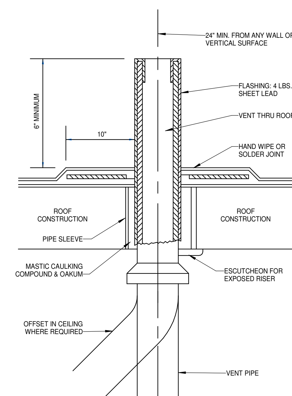
9 VENT THRU ROOF DETAIL NOT TO SCALE:
