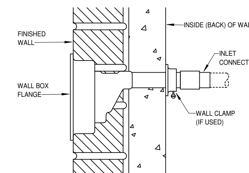
8 FREEZEPROOF WALL HYDRANT DETAIL NOT TO SCALE:
