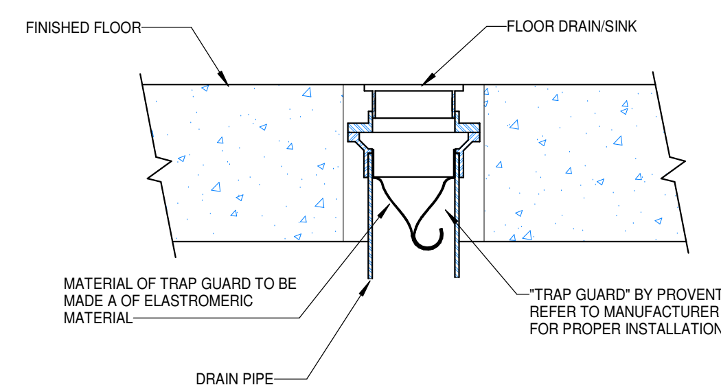
6 TRAP-GUARD DETAIL NOT TO SCALE:
