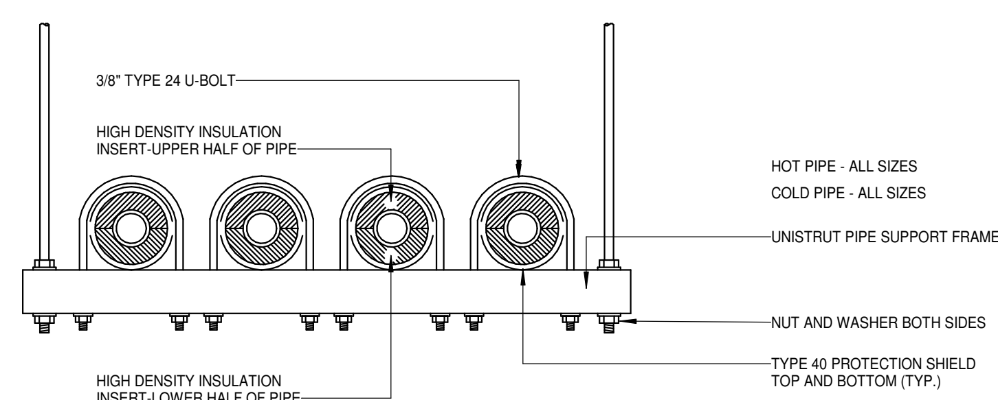
10 HORIZONTAL PIPE SUPPORT DETAIL NOT TO SCALE:
