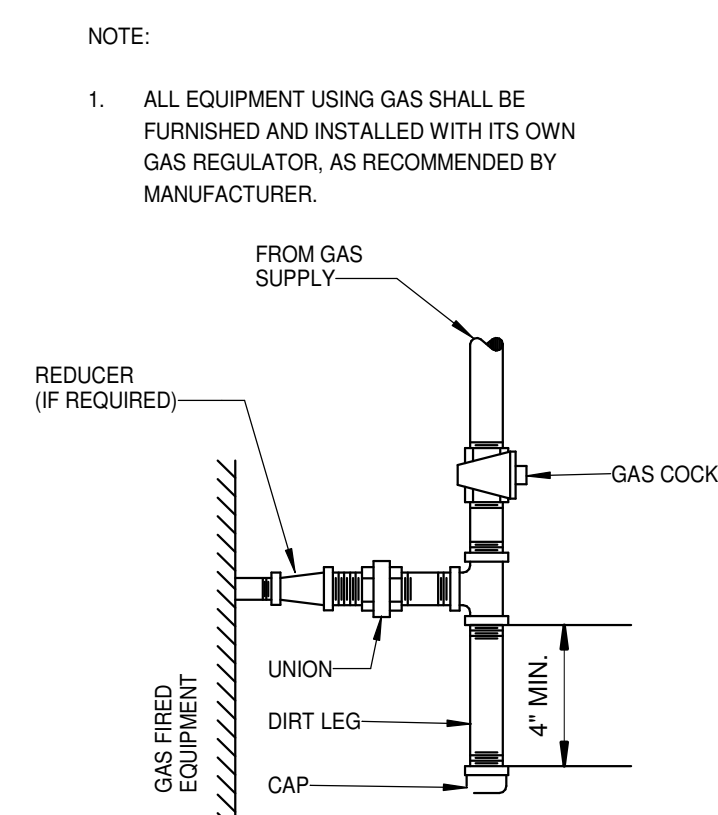
2 GAS CONNECTION DETAIL
