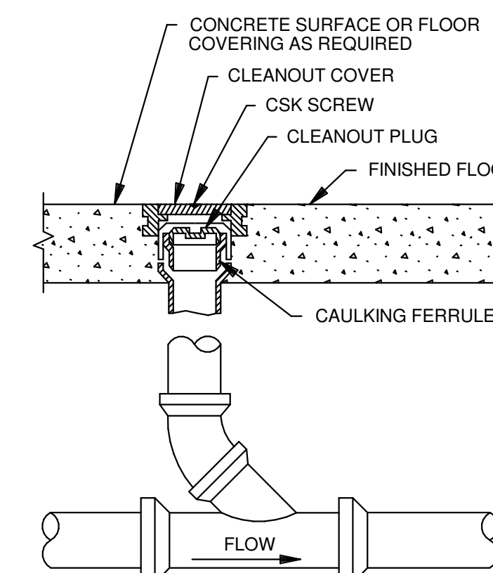
4 FLOOR CLEANOUT-FINISHED ROOMS NOT TO SCALE:
