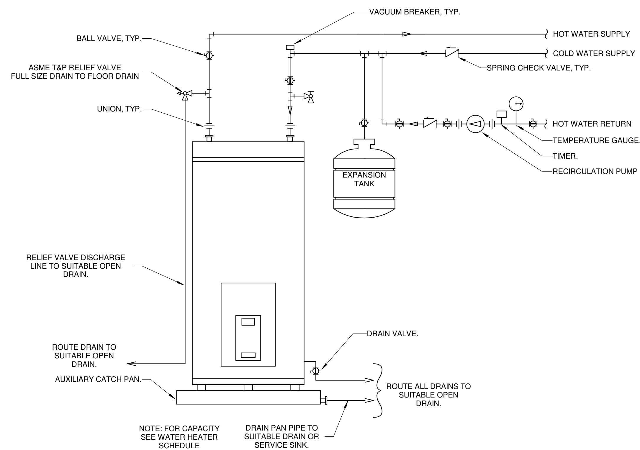
1 ELECTRIC WATER HEATER DETAIL
