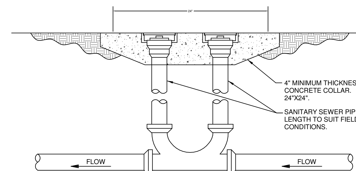
3 DOUBLE CLEANOUT TO GRADE NOT TO SCALE:
