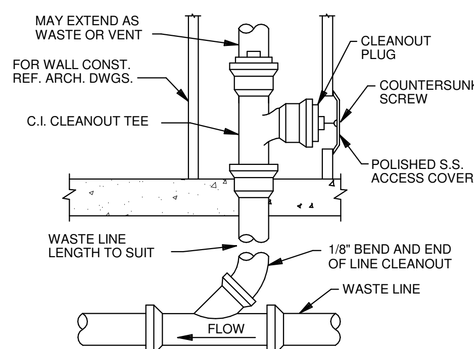
5 WALL CLEANOUT-FINISHED ROOMS NOT TO SCALE:
