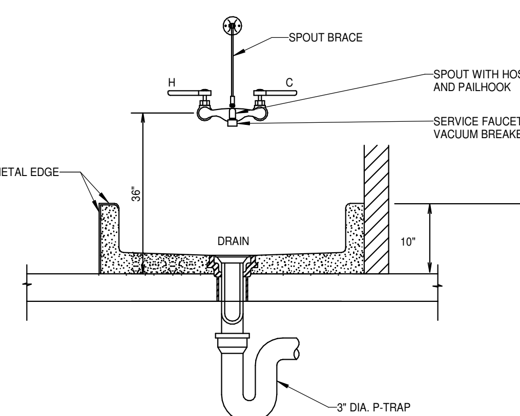
7 SERVICE SINK DETAIL NOT TO SCALE:
