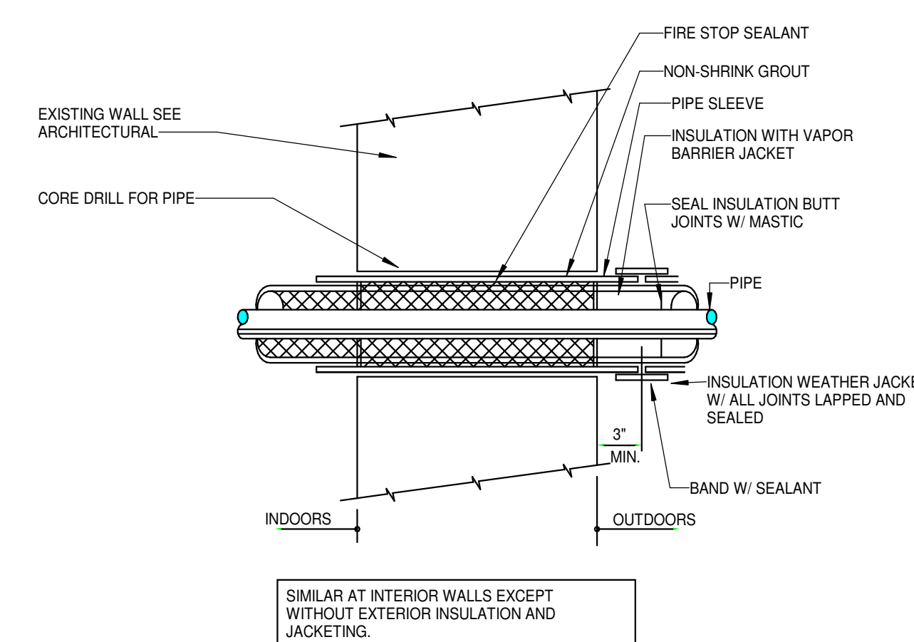
12 PIPE PENETRATION AT WALL NOT TO SCALE:
