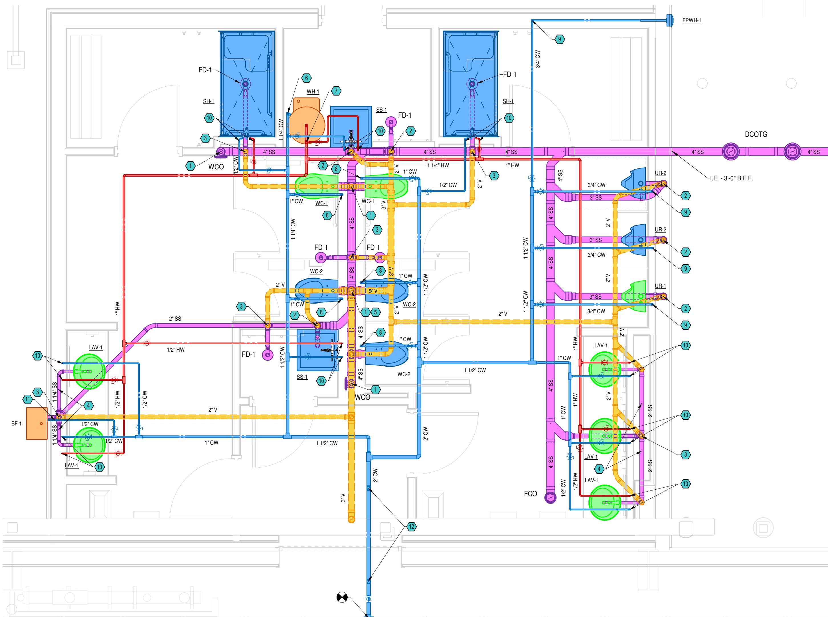
2 ENLARGED WAREHOUSE ADDITION PLUMBING PLAN 3/8" = 1'-0"
