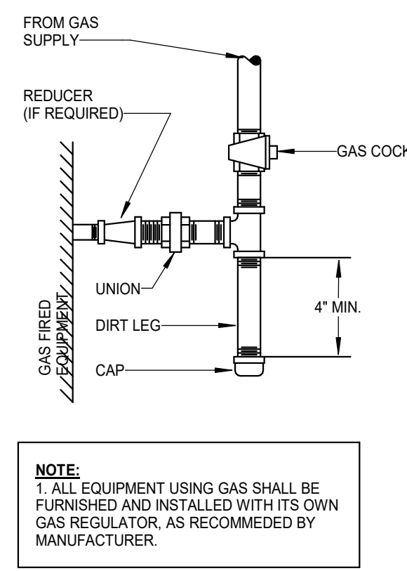
6 GAS CONNECTION DETAIL NOT TO SCALE:
