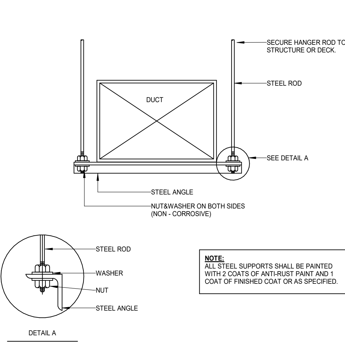
4 DUCT HANGER DETAIL NOT TO SCALE:
