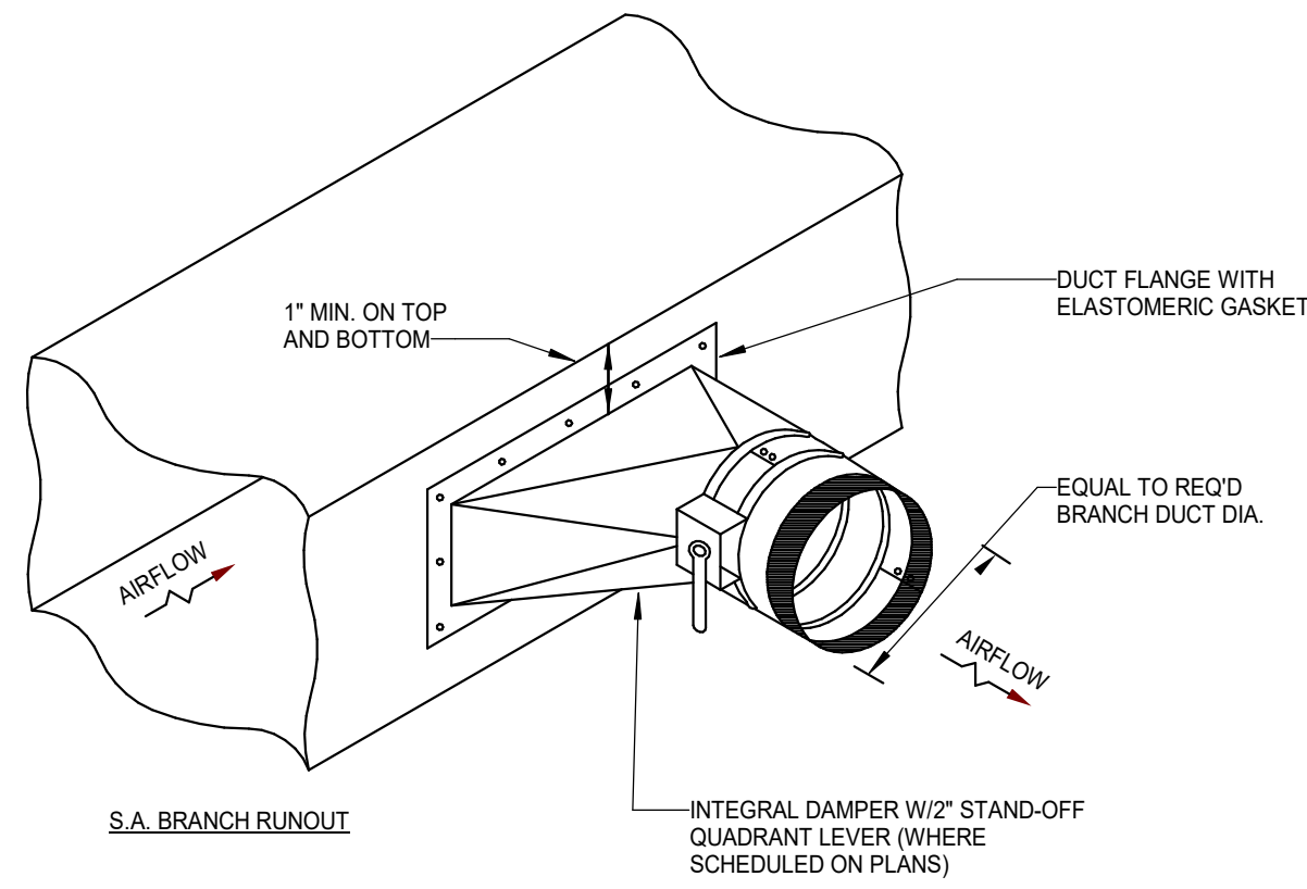
2 BRANCH DUCT TAKE-OFF (W/ DAMPER) DETAIL NOT TO SCALE:
