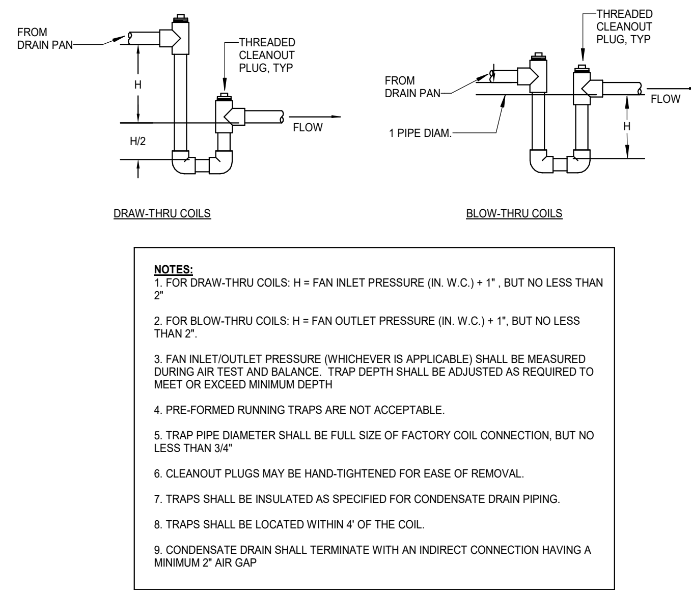
5 COIL CONDENSATE TRAP DETAIL NOT TO SCALE:
