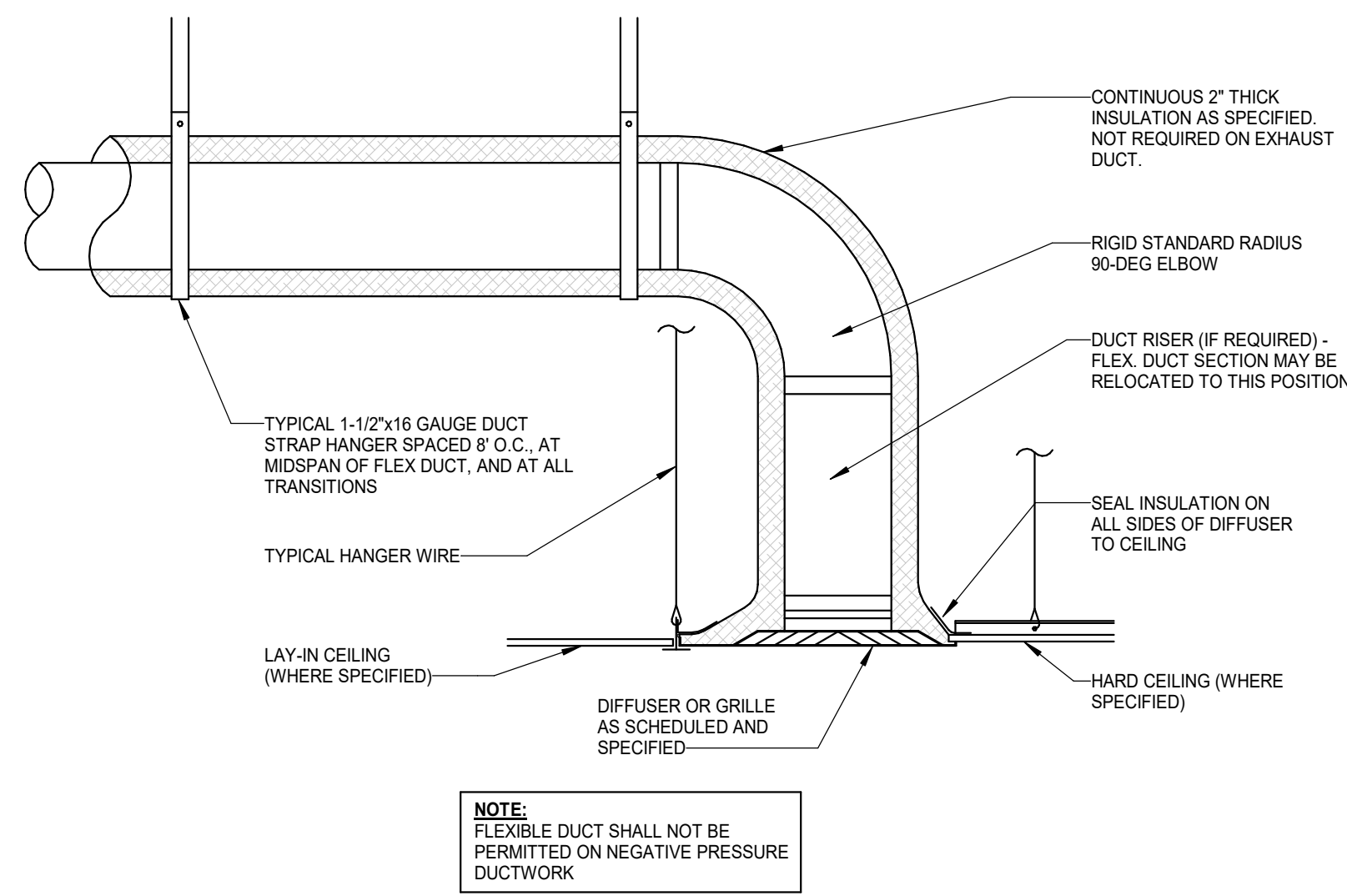
1 AIR DEVICE INSULATION (W/ FLEX DUCT) DETAIL NOT TO SCALE:
