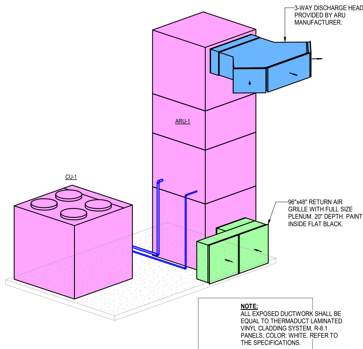
8 AIR ROTATION UNIT - ISOMETRIC NOT TO SCALE:
