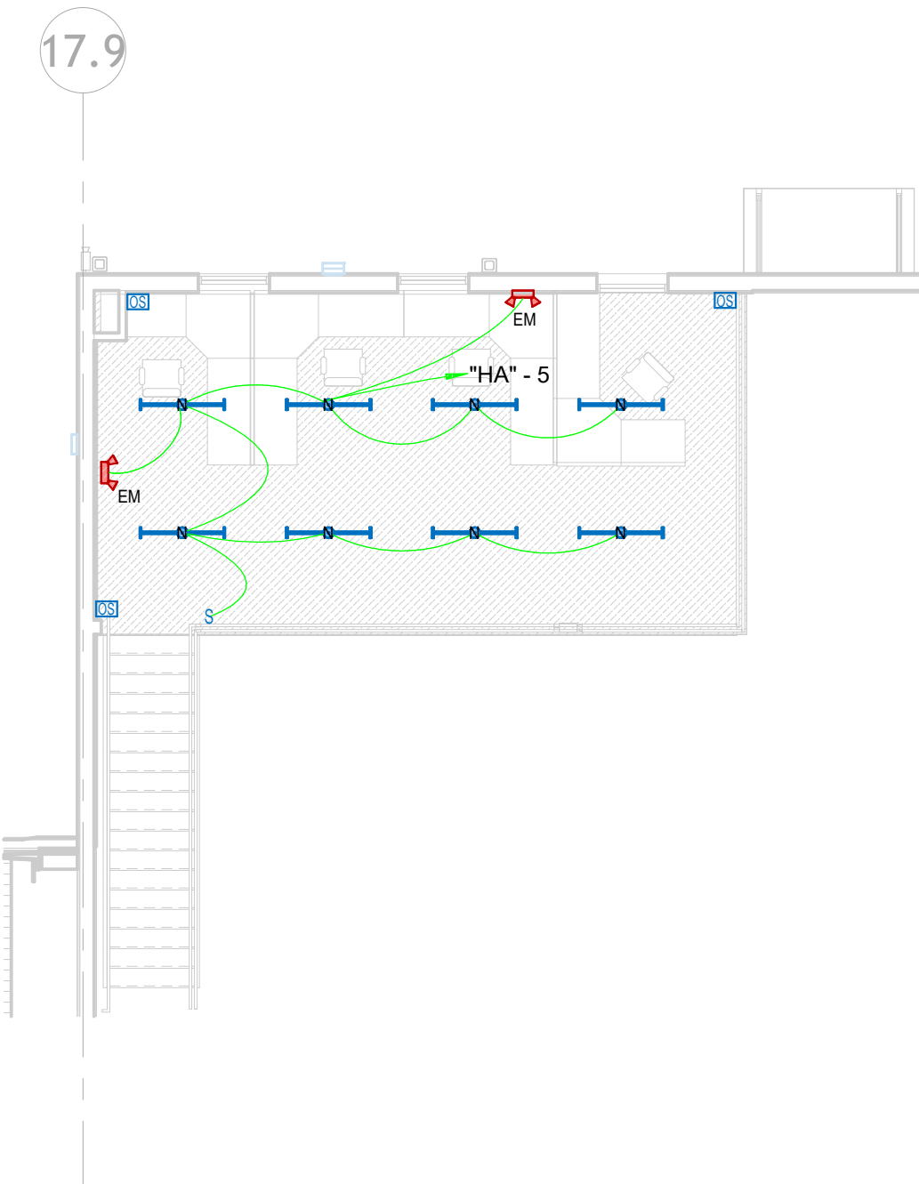
2 WAREHOUSE MEZZ LIGHTING PLAN 1/8" = 1'-0"
