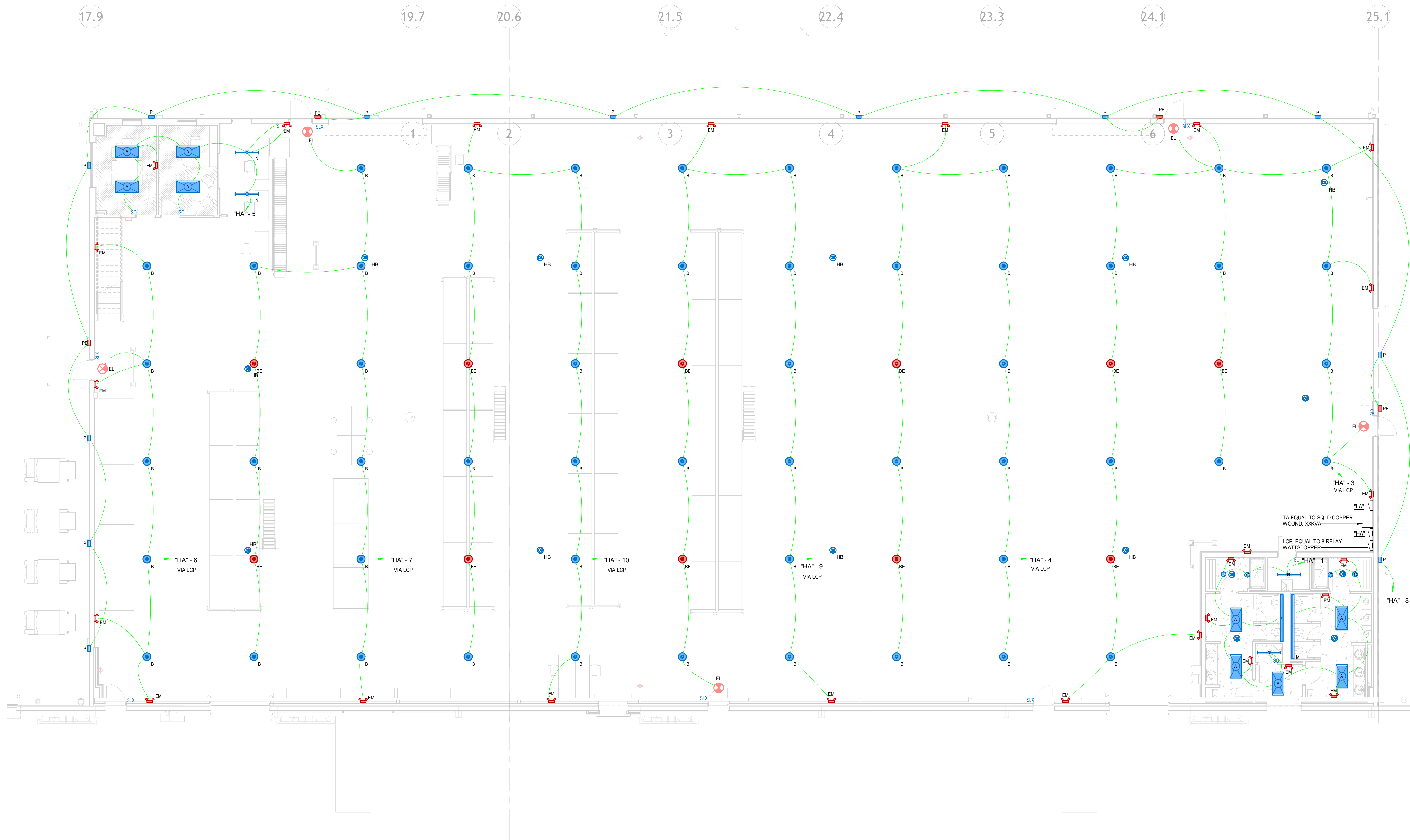
1 WAREHOUSE ADDITION LIGHTING PLAN 1/8" = 1'-0"
