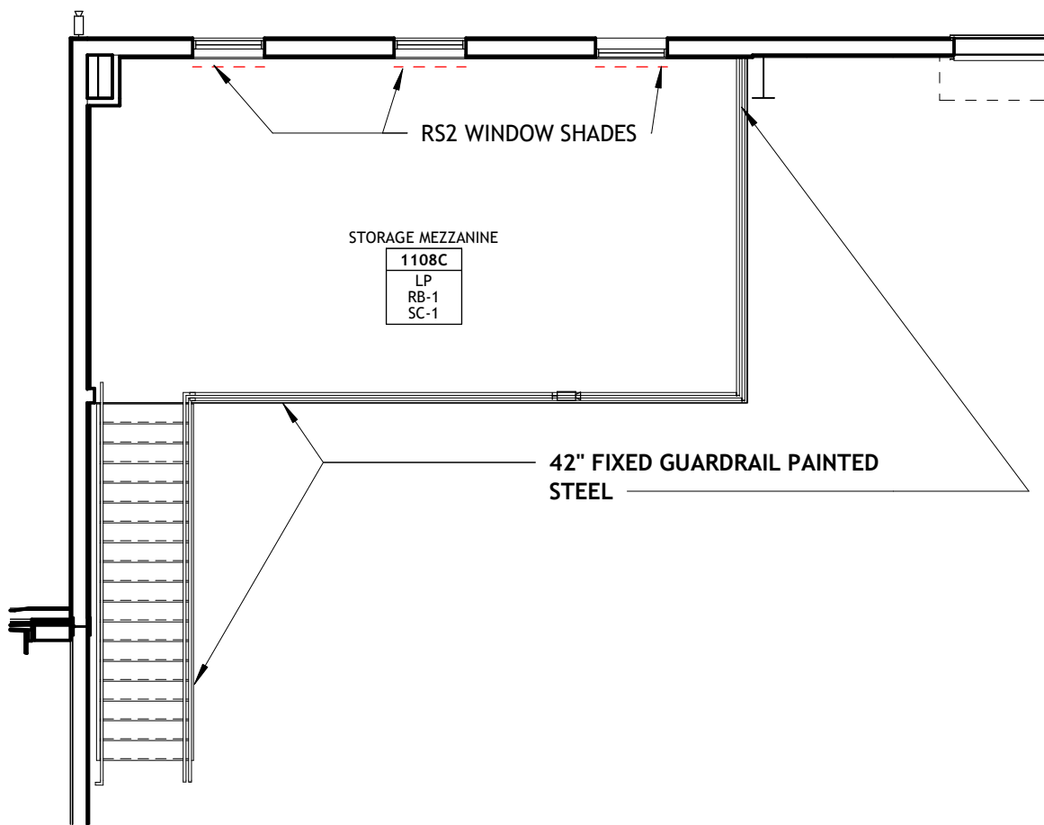
2 | WAREHOUSE MEZZANINE FLOOR PLAN Copy 1
