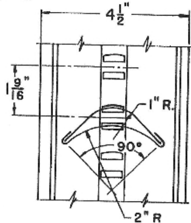
DETAIL 2 RUNNER
