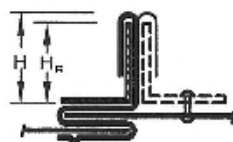
STANDING S (ANGLE REINFORCED) T-14
