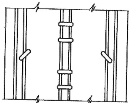
ALTERNATE DETAIL 5 LARGE DOUBLE VANE RUNNER
