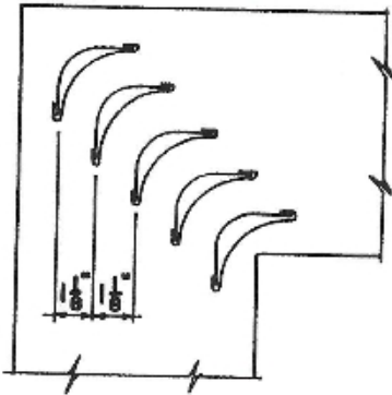
DETAIL 3 SMALL DOUBLE VANE
