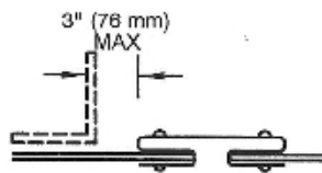
T-8 DOUBLE "S" SLIP (T-8a REINFORCED)
