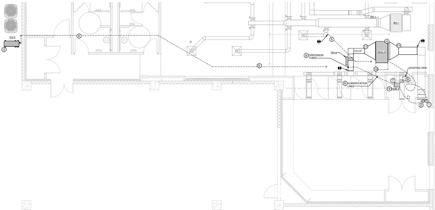
② FIRST FLOOR PLAN - HVAC 1/4" = 1'-0"
