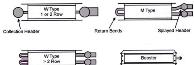
Figure 1: Coil Types
