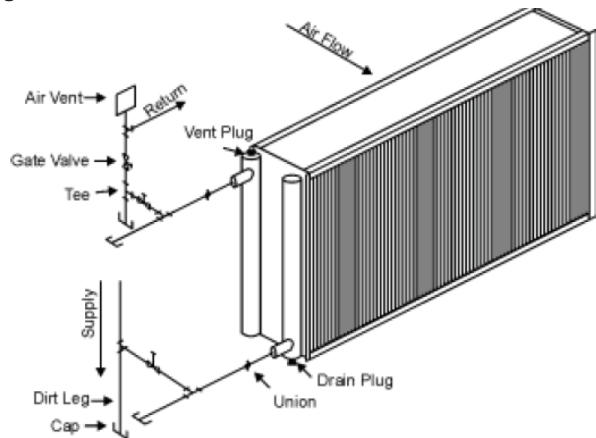
Figure 4: Horizontal Air Flow
