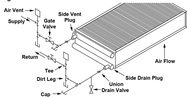
Figure 5: Vertical Air Flow
