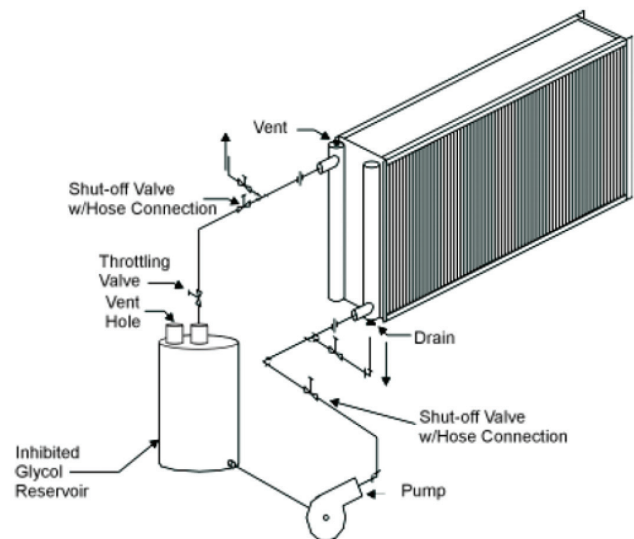
Figure 8: Flushing System
