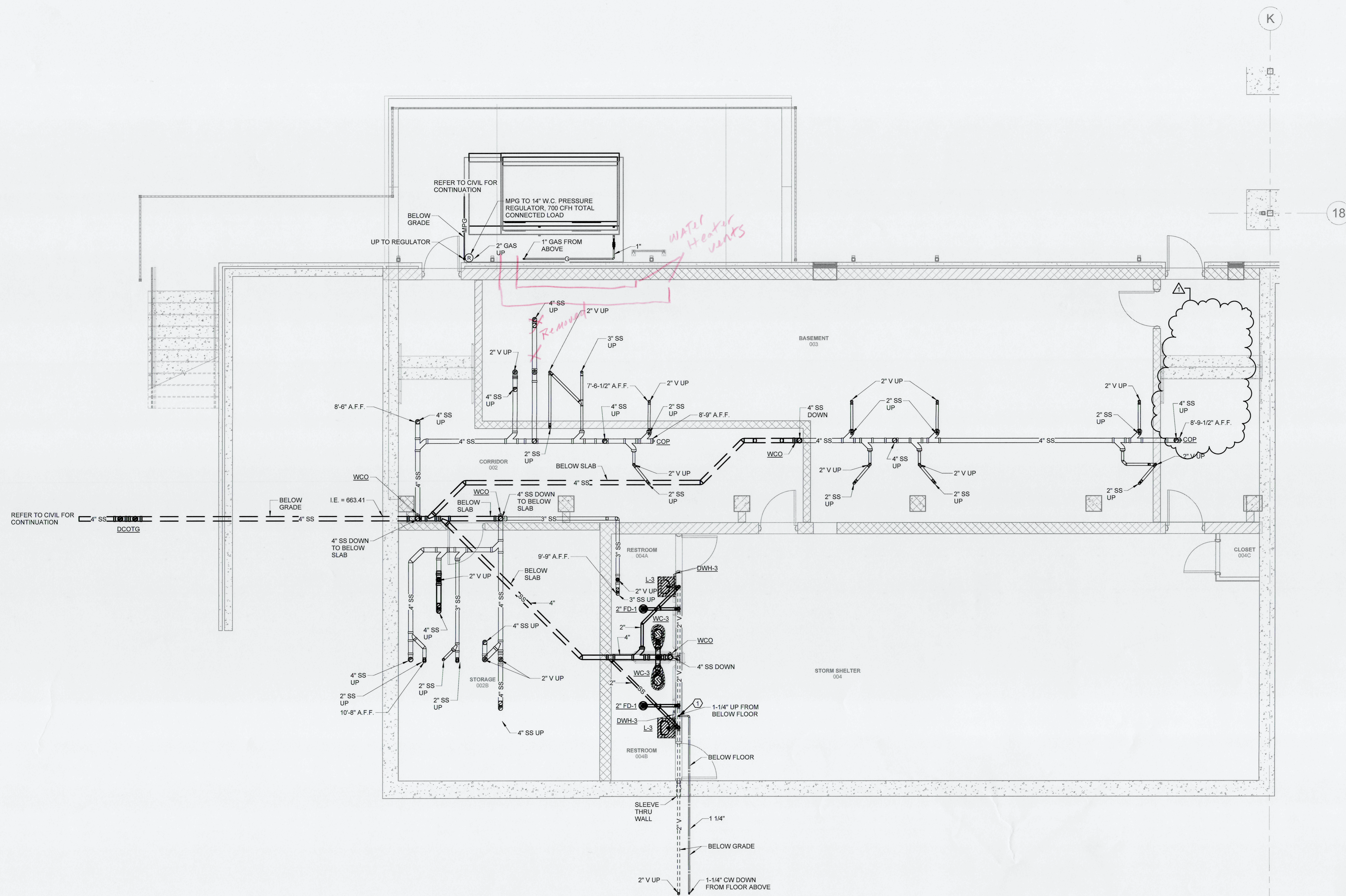
① BASEMENT - PLUMBING - BUILDING #6 1/4" = 1'-0"
