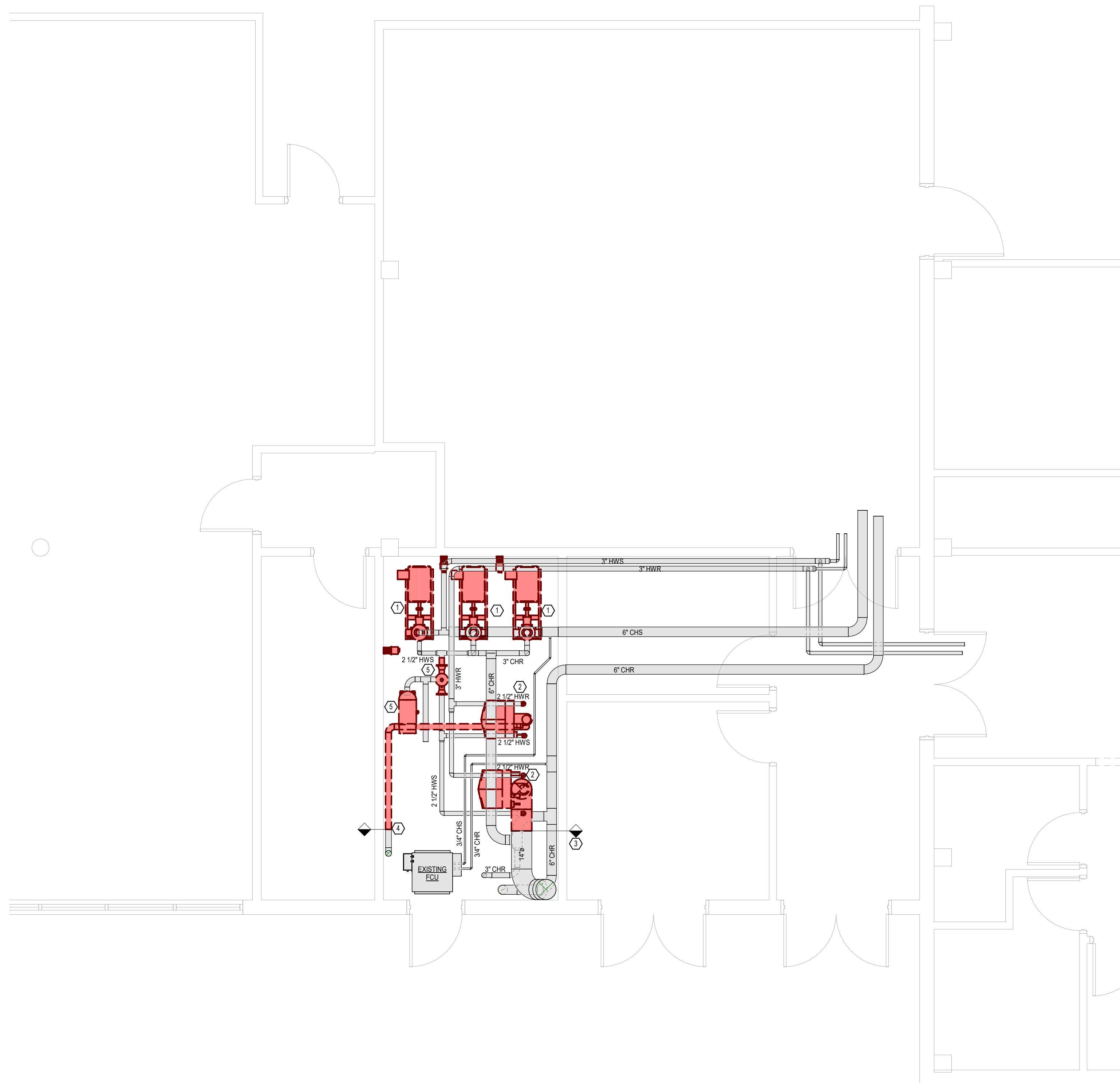
1 FIRST FLOOR DEMOLITION PLAN - MECHANICAL 1/4" = 1'-0"
