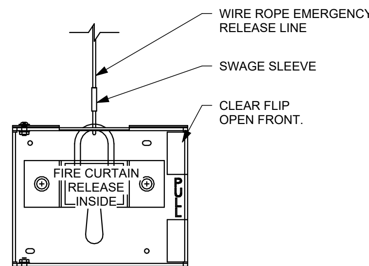
9 DETAIL - FIRE CURTAIN PULL BOX
