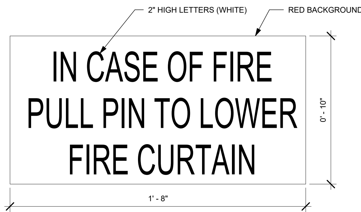
5 DETAIL - FIRE CURTAIN SIGNAGE
