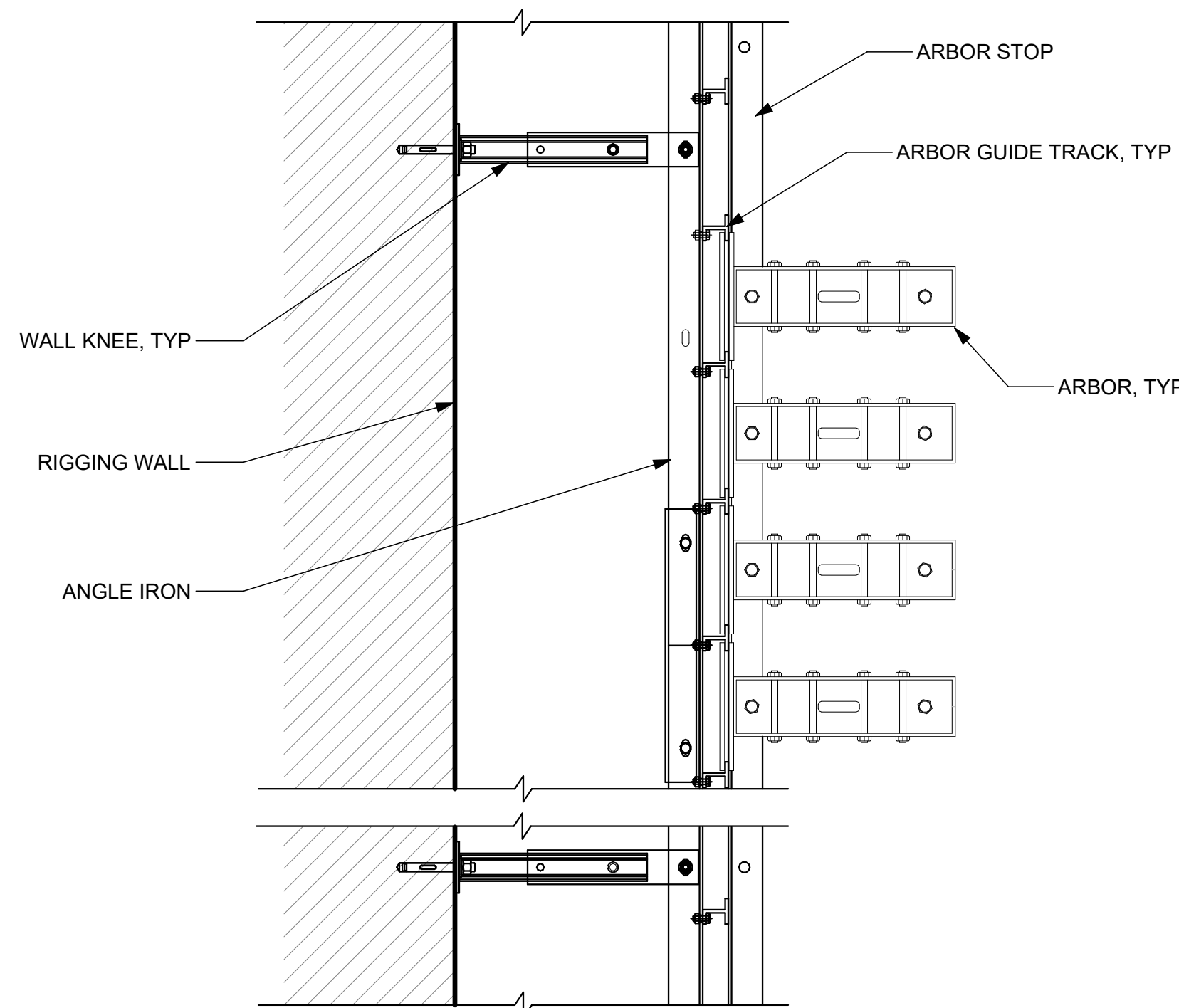
10 PLAN DETAIL - RIGGING WALL 1 1/2" = 1'-0"
