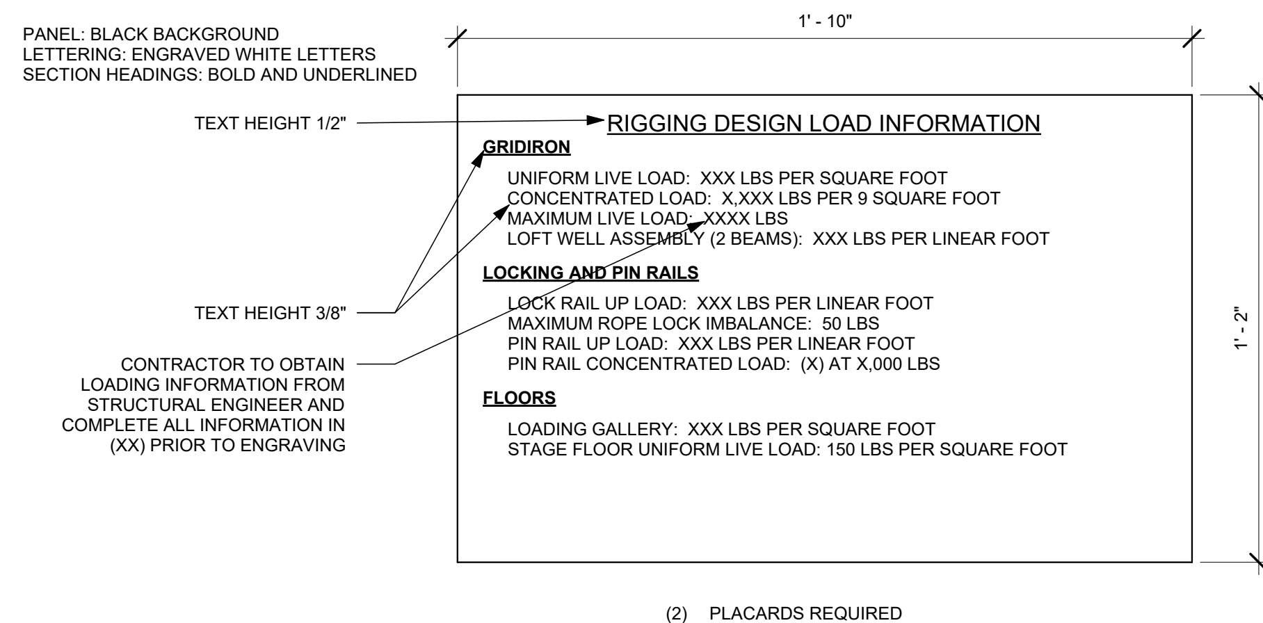
2 DETAIL - RIGGING DESIGN LOAD SIGNAGE
