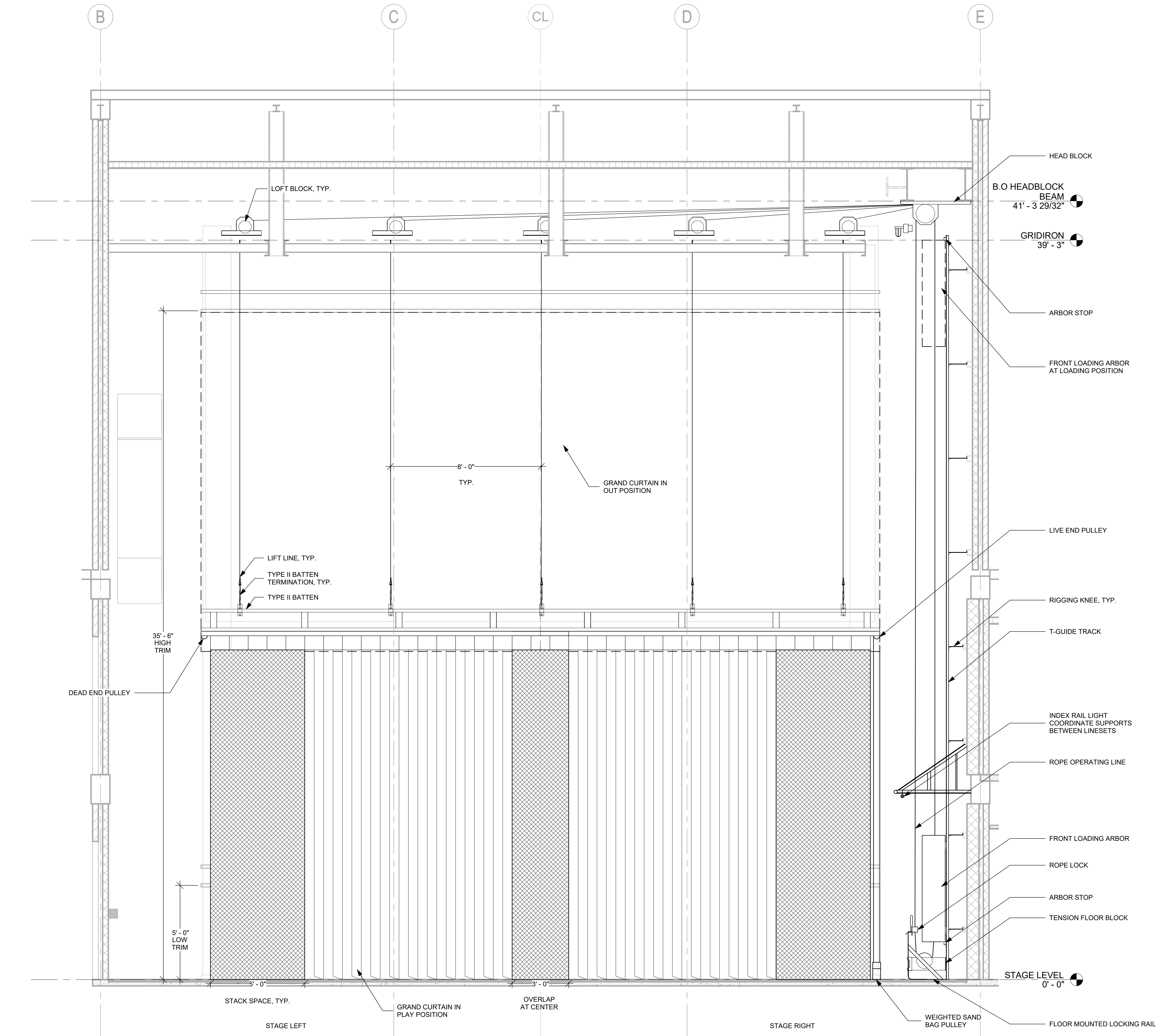
1 ELEVATION - GRAND CURTAIN 3/8" = 1'-0"
