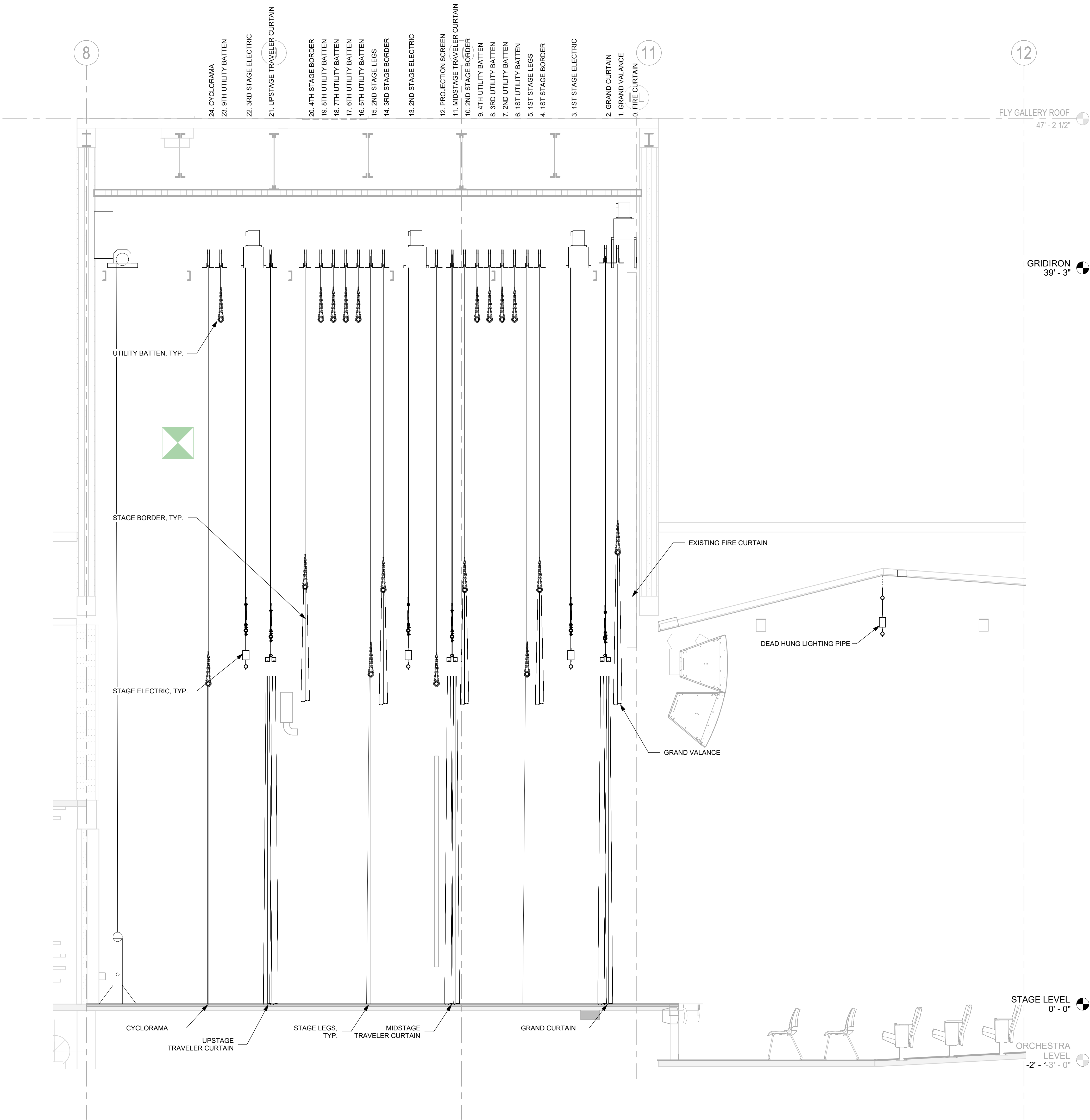
1 SECTION - THEATE RIGGING, CENTERLINE SECTION 3/8" = 1'-0"
