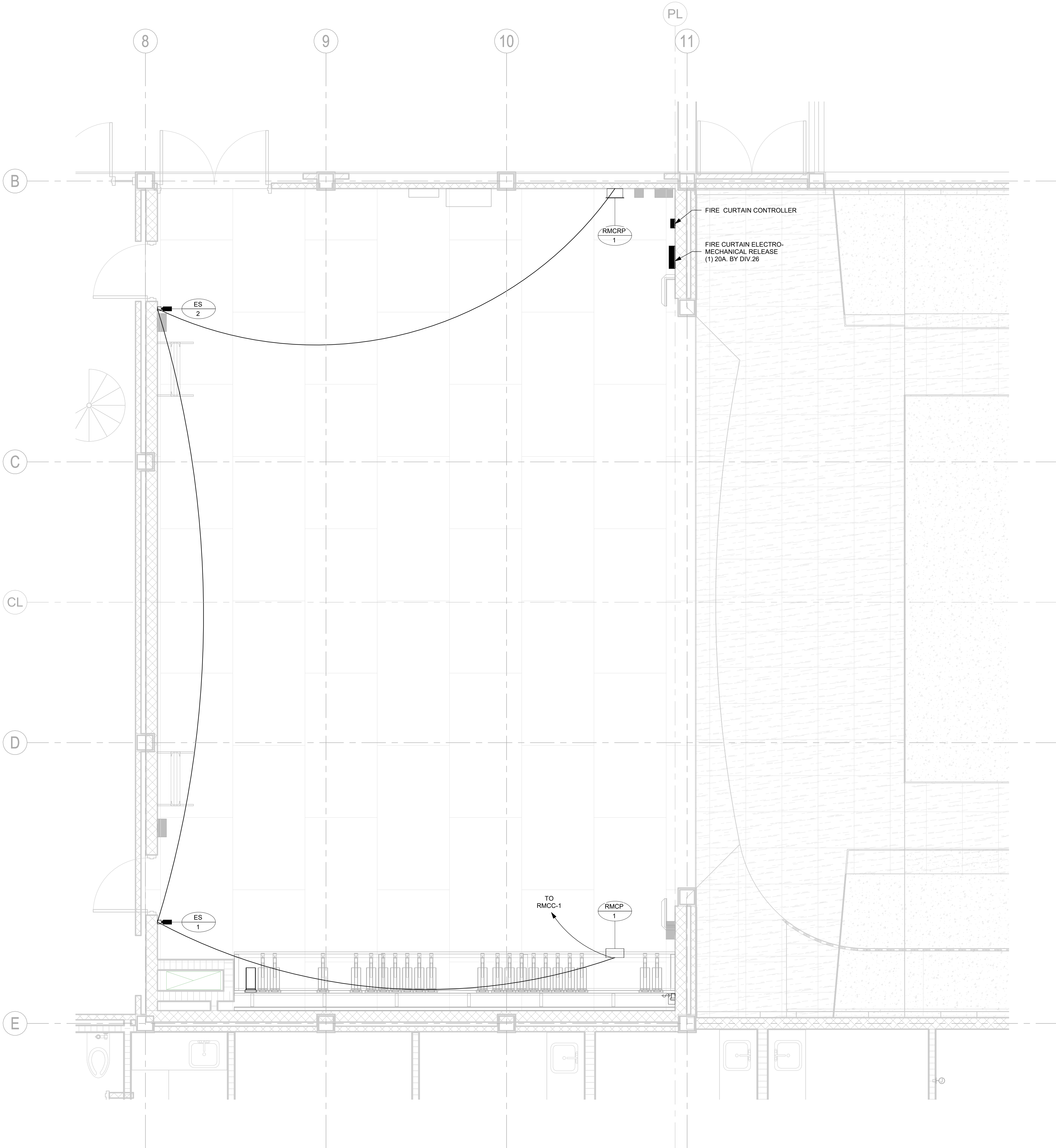
1 PLAN - RIGGING POWER AND PANEL, STAGE LEVEL 3/8" = 1'-0"
