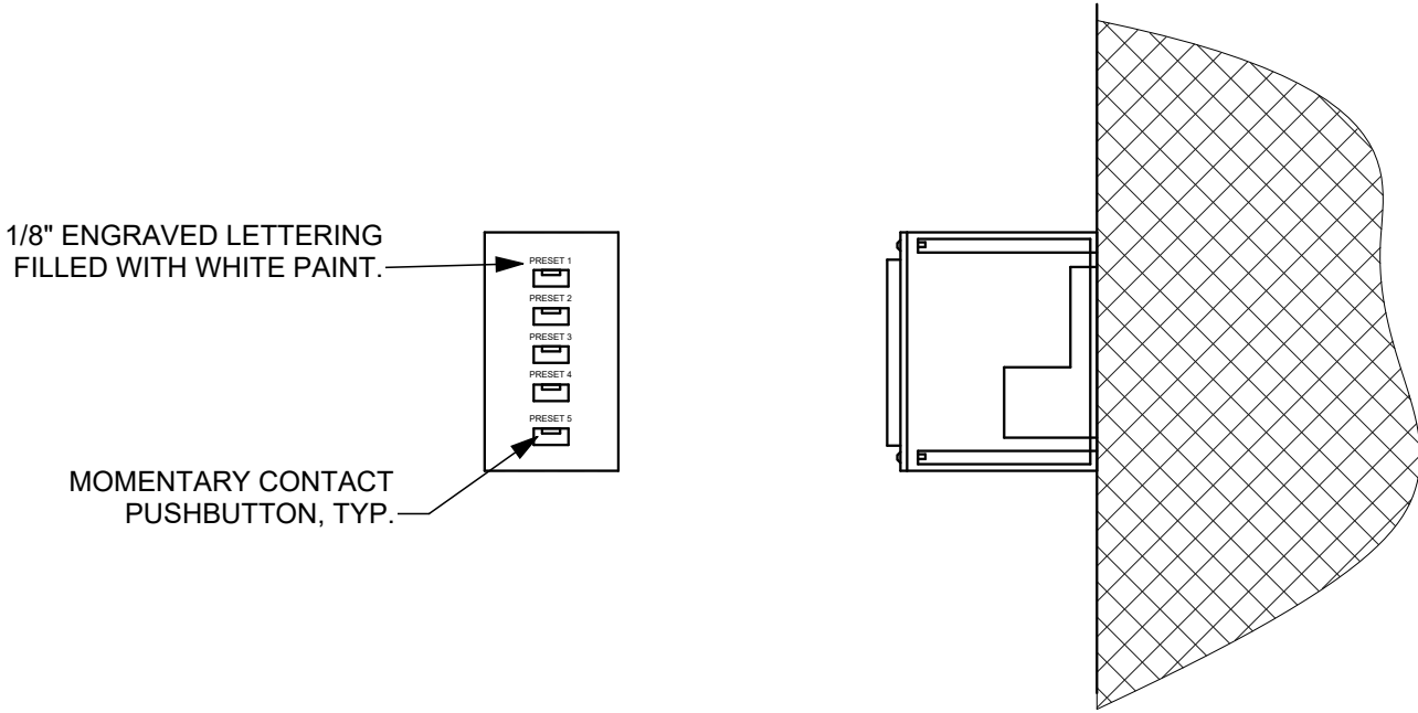
3 DETAIL - EP-5 - SURFACE 3" = 1'-0"
