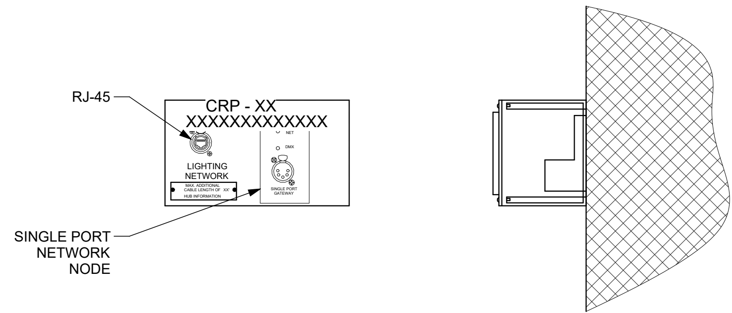
7 DETAIL - CRP - 1 NETWORK - 1 PORT NODE - SURFACE 3" = 1'-0"
