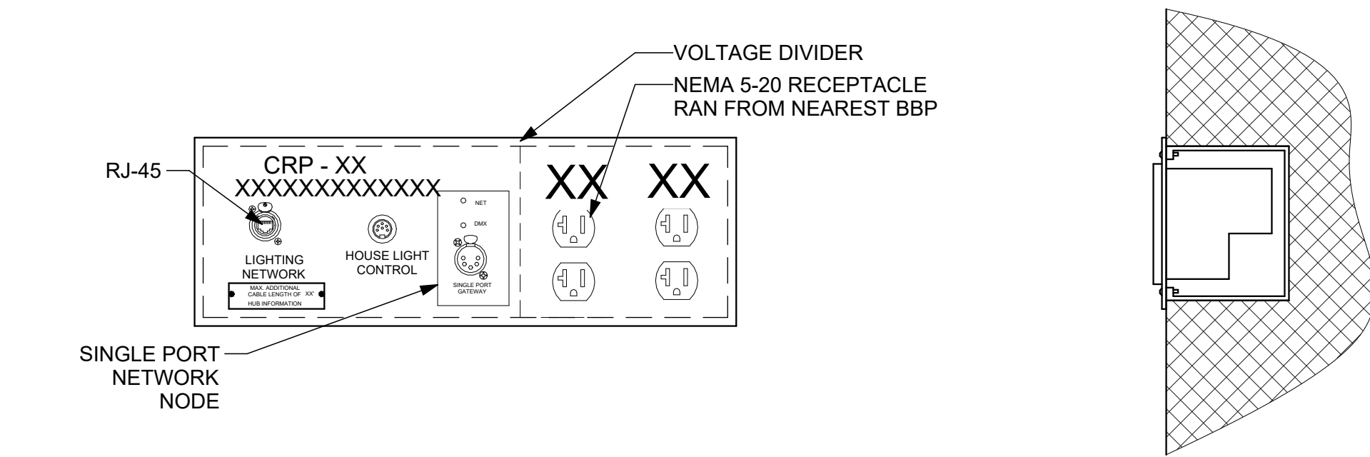
8 DETAIL - CRP -1 NETWORK - 1 AUX - 1 PORT NODE - CONV POWER- FLUSH 3" = 1'-0"
