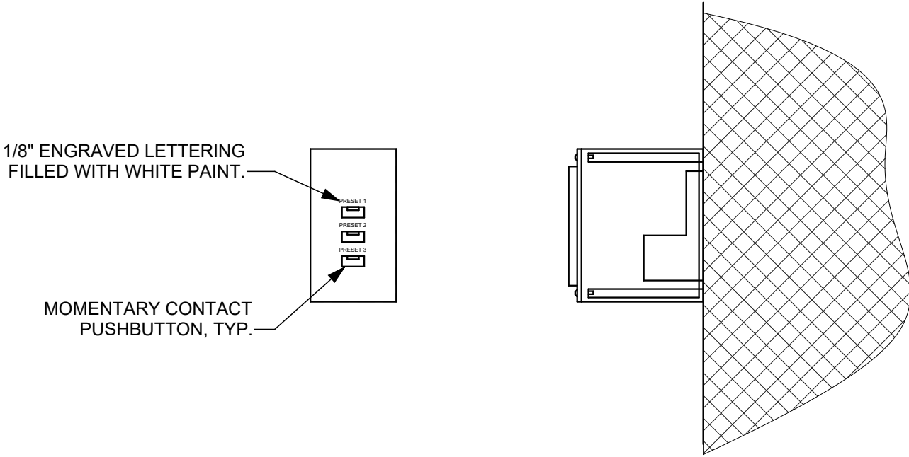
2 DETAIL - EP-3 - SURFACE 3" = 1'-0"
