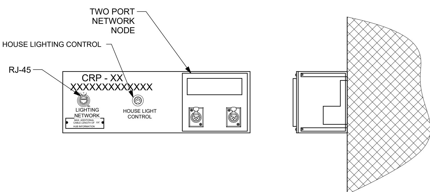
5 DETAIL - CRP - 1 NETWORK - 1 AUX - 2 PORT NODE- SURFACE 3" = 1'-0"
