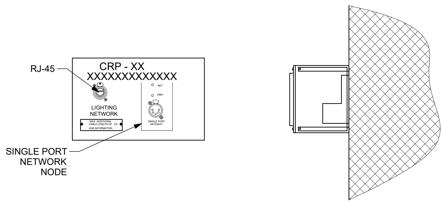
1 DETAIL - CRP - 1 PORT NODE - 1 NETWORK - SURFACE 3" = 1'-0"
