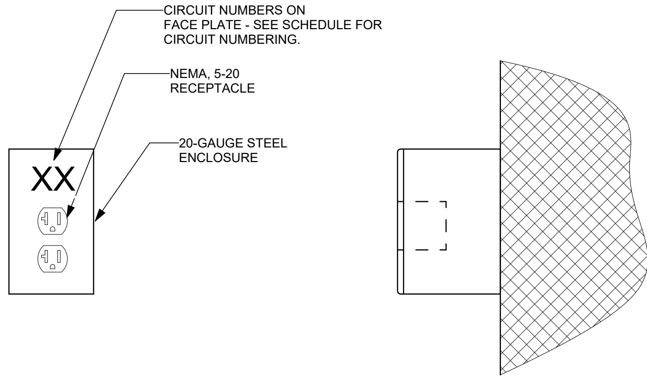
6 DETAIL - PB - 1 CIRC - SURFACE 3" = 1'-0"
