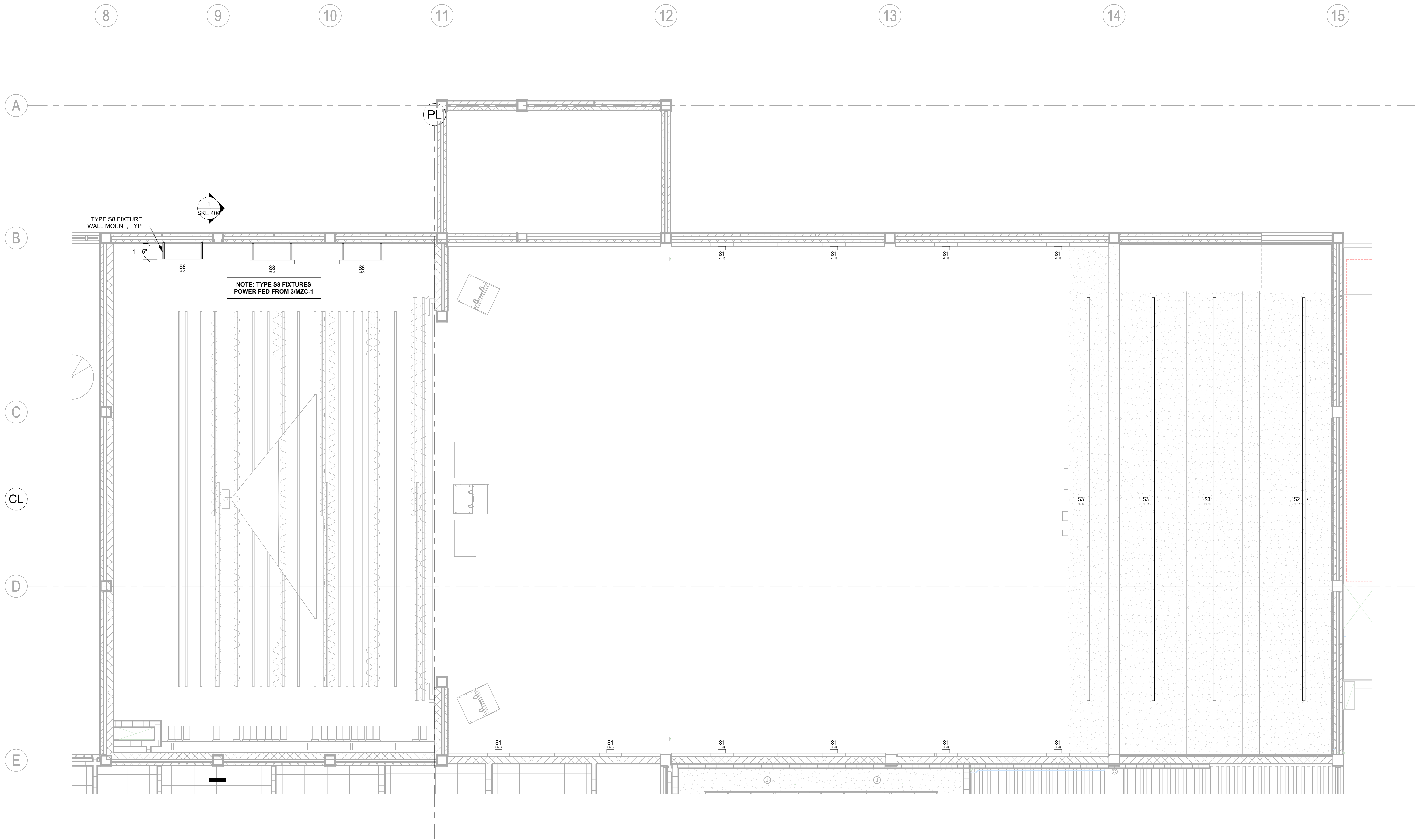
1 LIGHTING CEILING PLAN - STAGE LEVEL SCALE: 1/4" = 1'-0"
