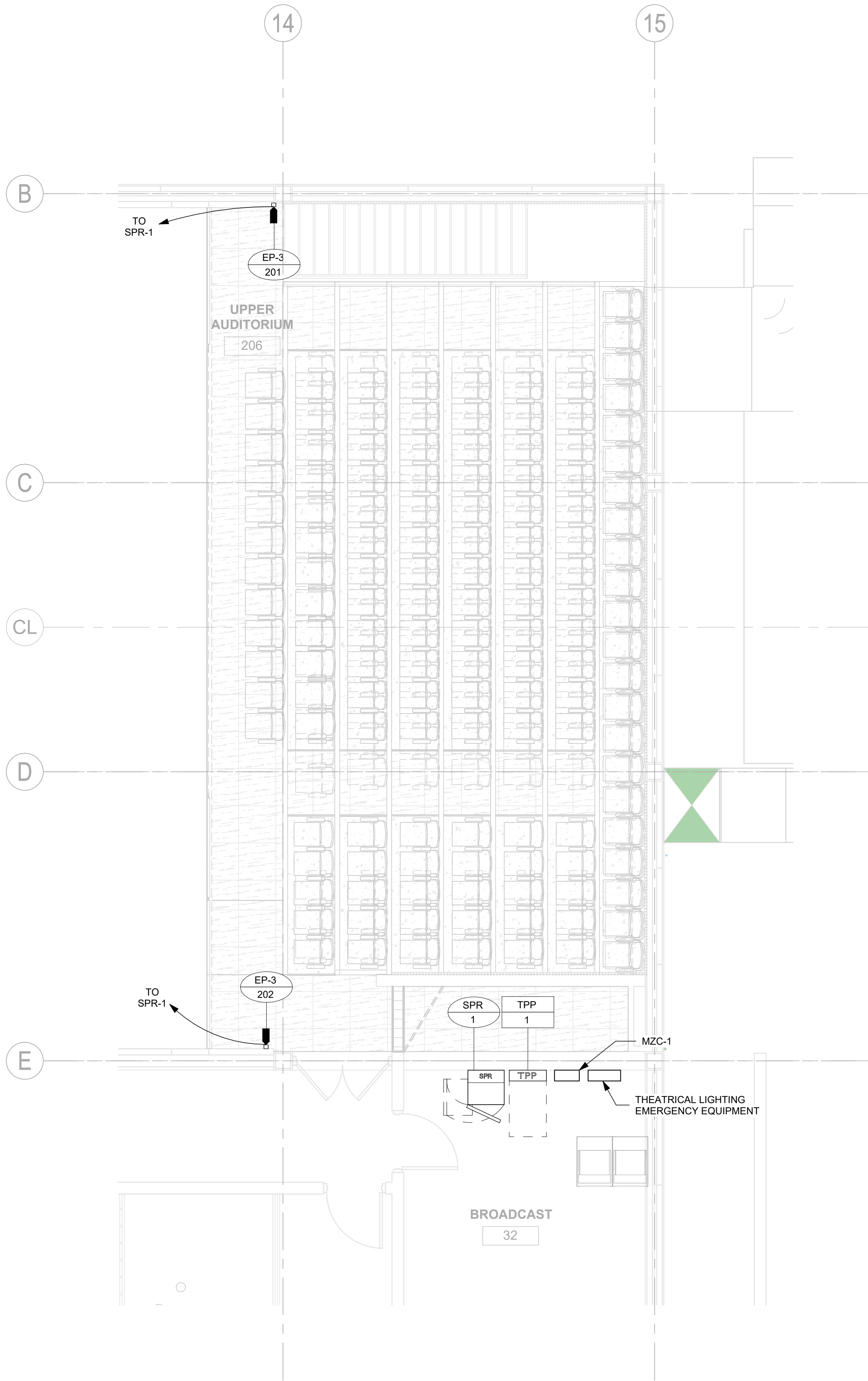
1 PLAN - POWER AND PANEL, BALCONY LEVEL SCALE: 1/4" = 1'-0"
