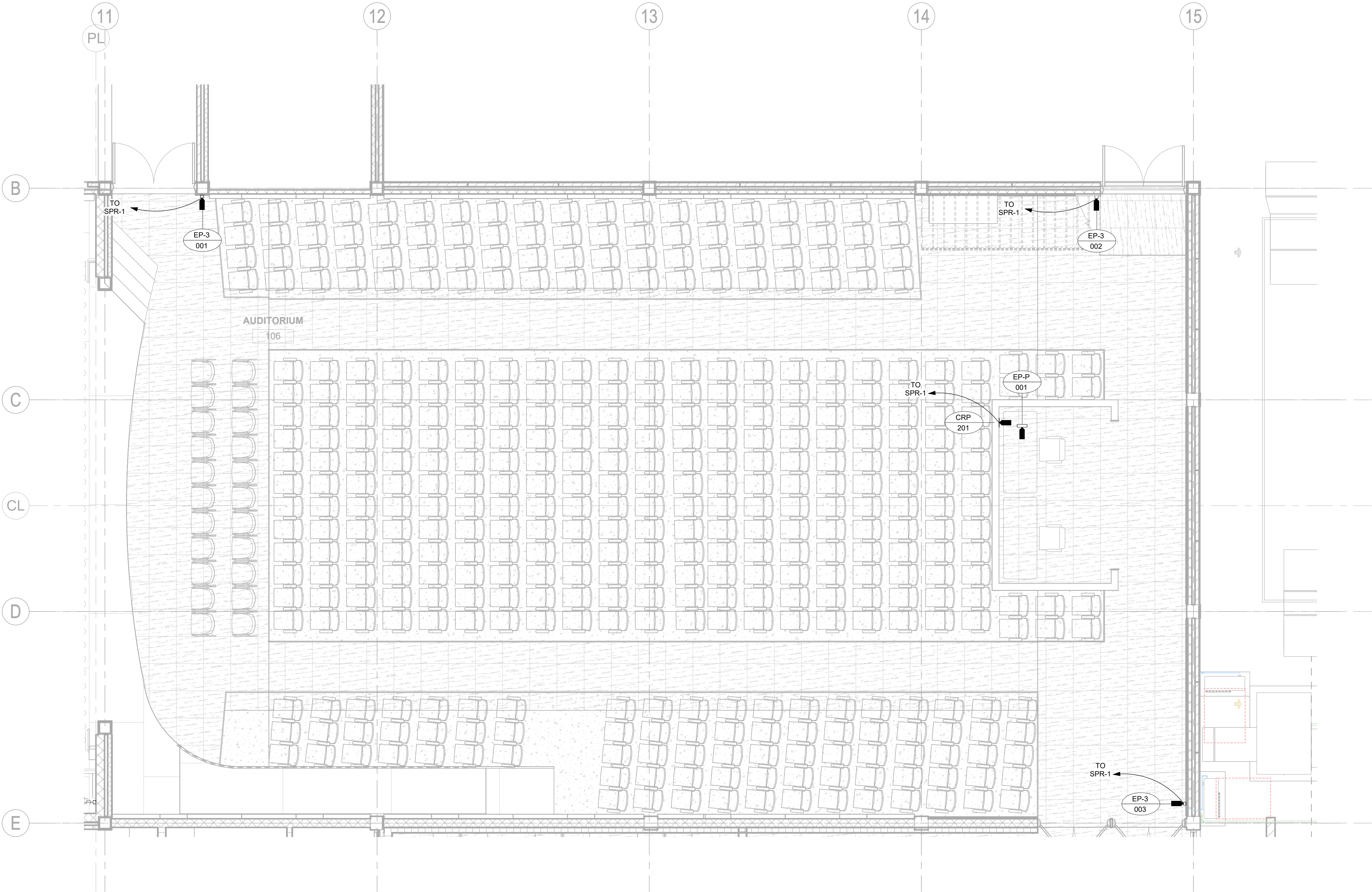
1 PLAN - ORCHESTRA LEVEL, POWER AND PANEL SCALE: 1/4" = 1'-0"
