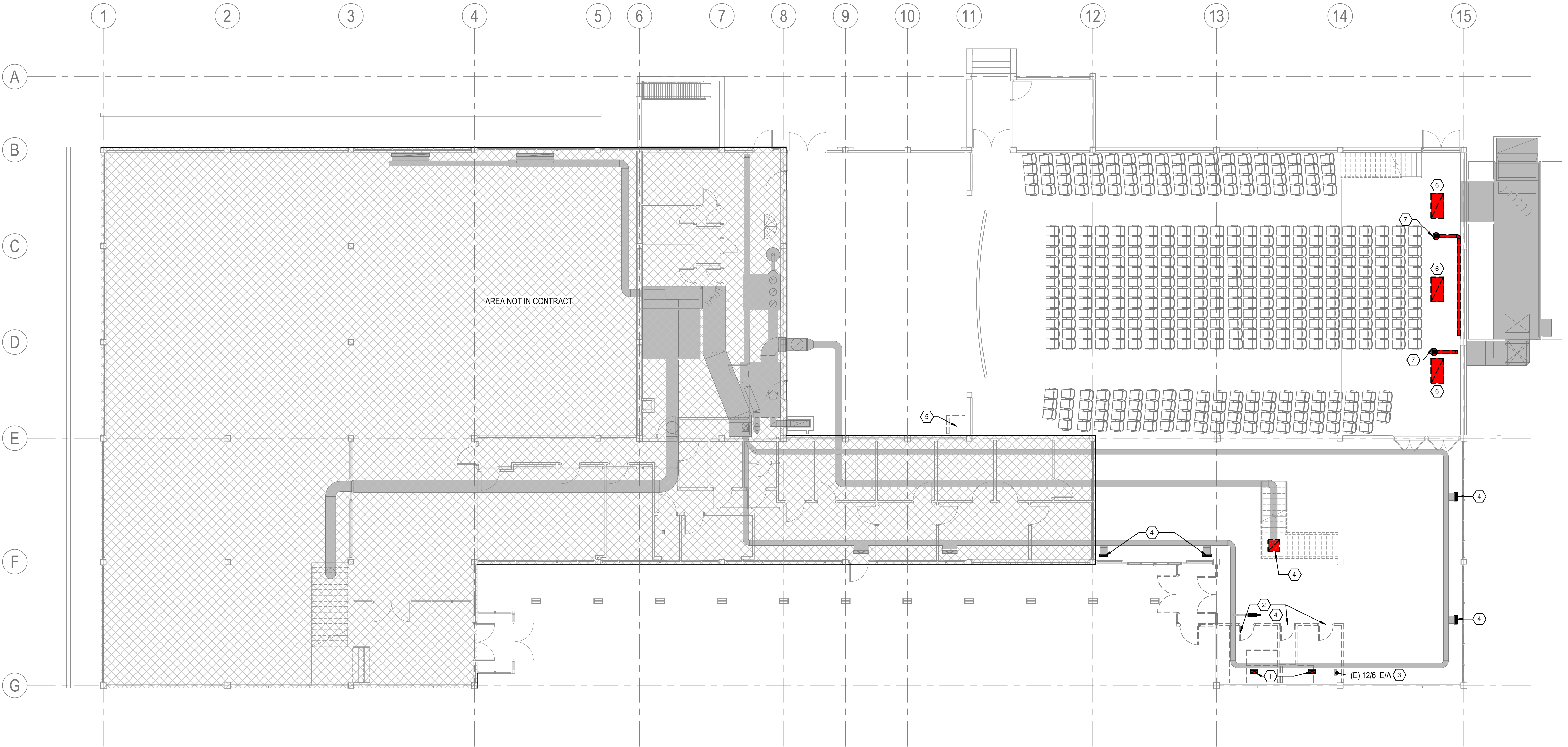
1 FIRST FLOOR DEMOLITION PLAN 1/8" = 1'-0" 0 4 8 16
