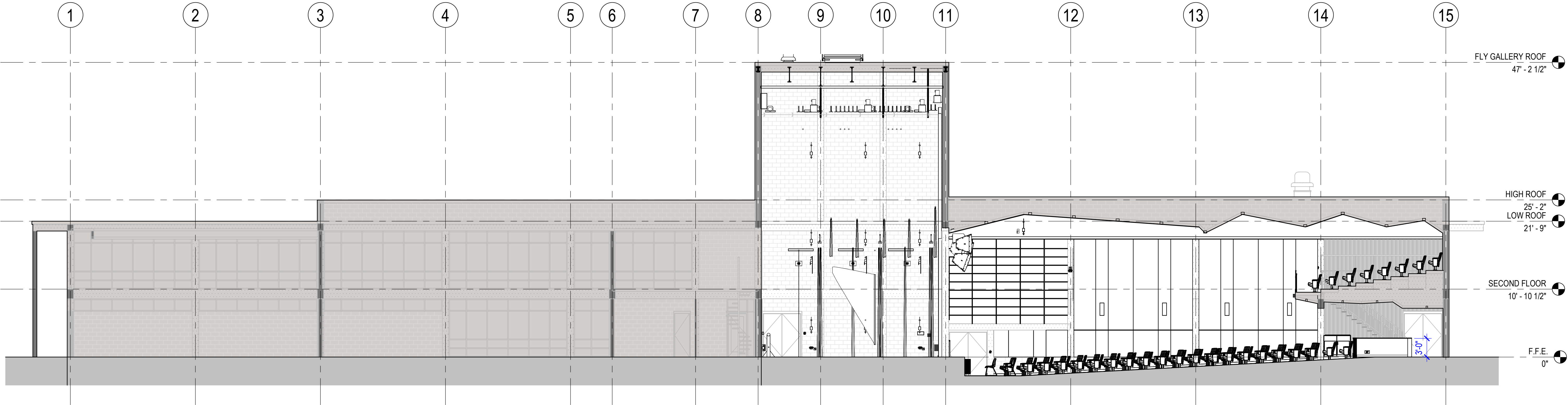
2 BUILDING SECTION 1/8" = 1'-0"
