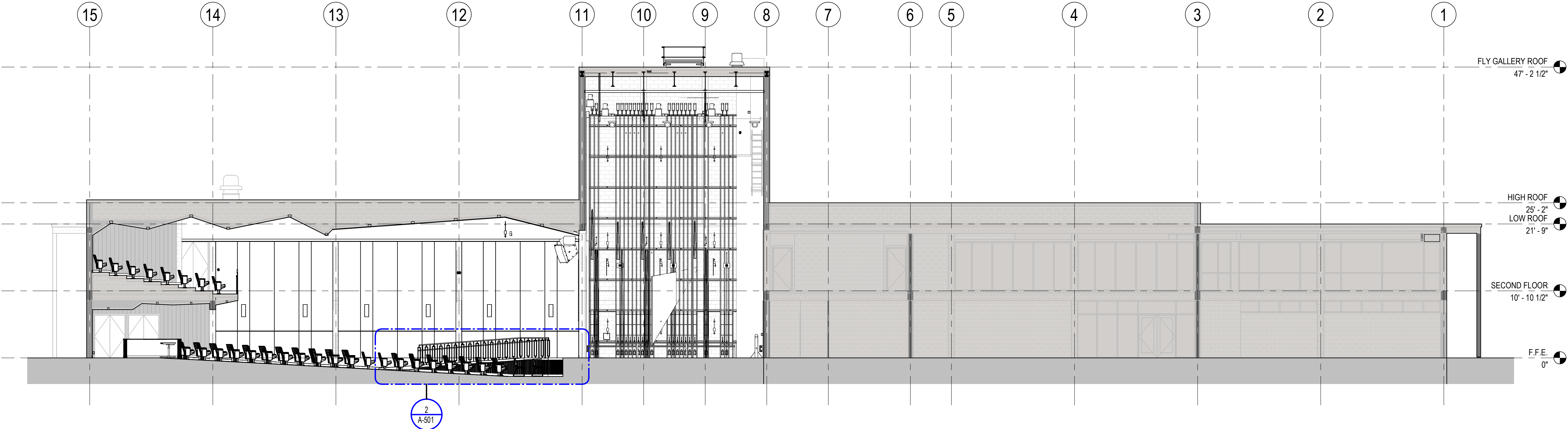
1 BUILDING SECTION 1/8" = 1'-0"
