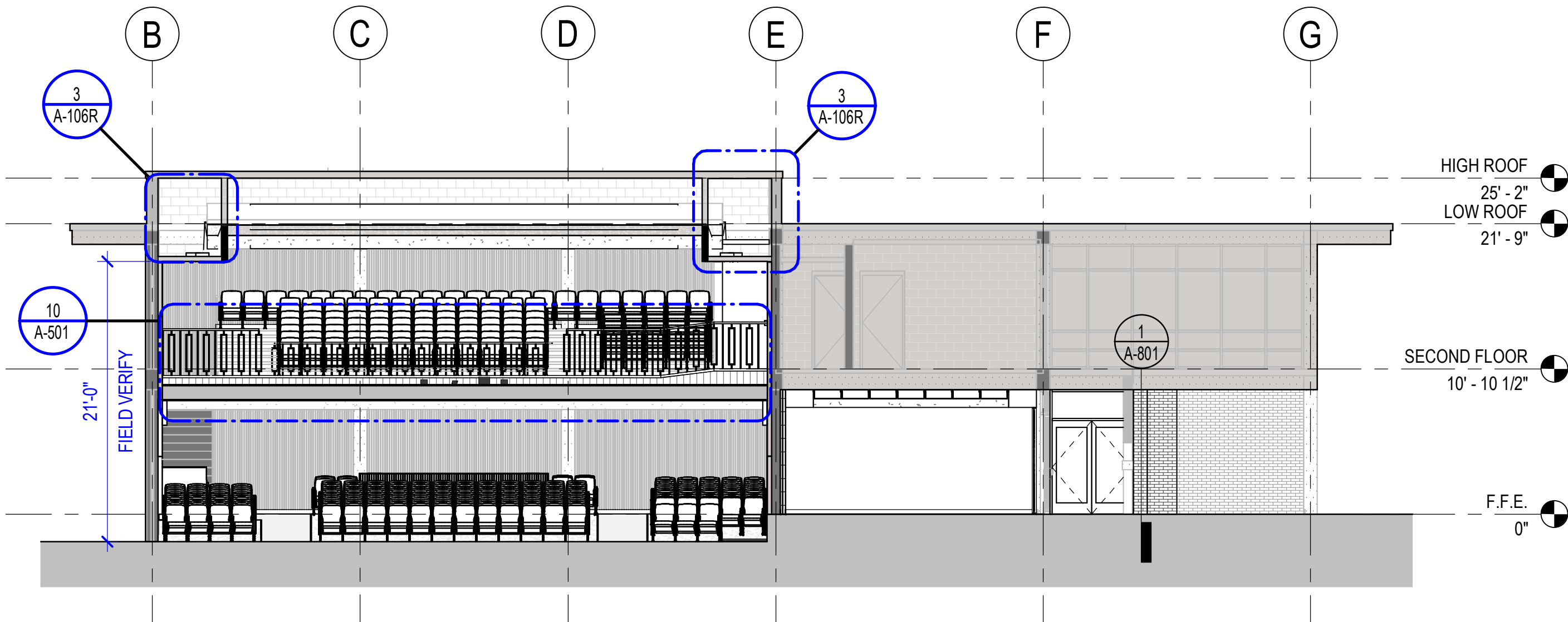
3 BUILDING SECTION 1/8" = 1'-0"
