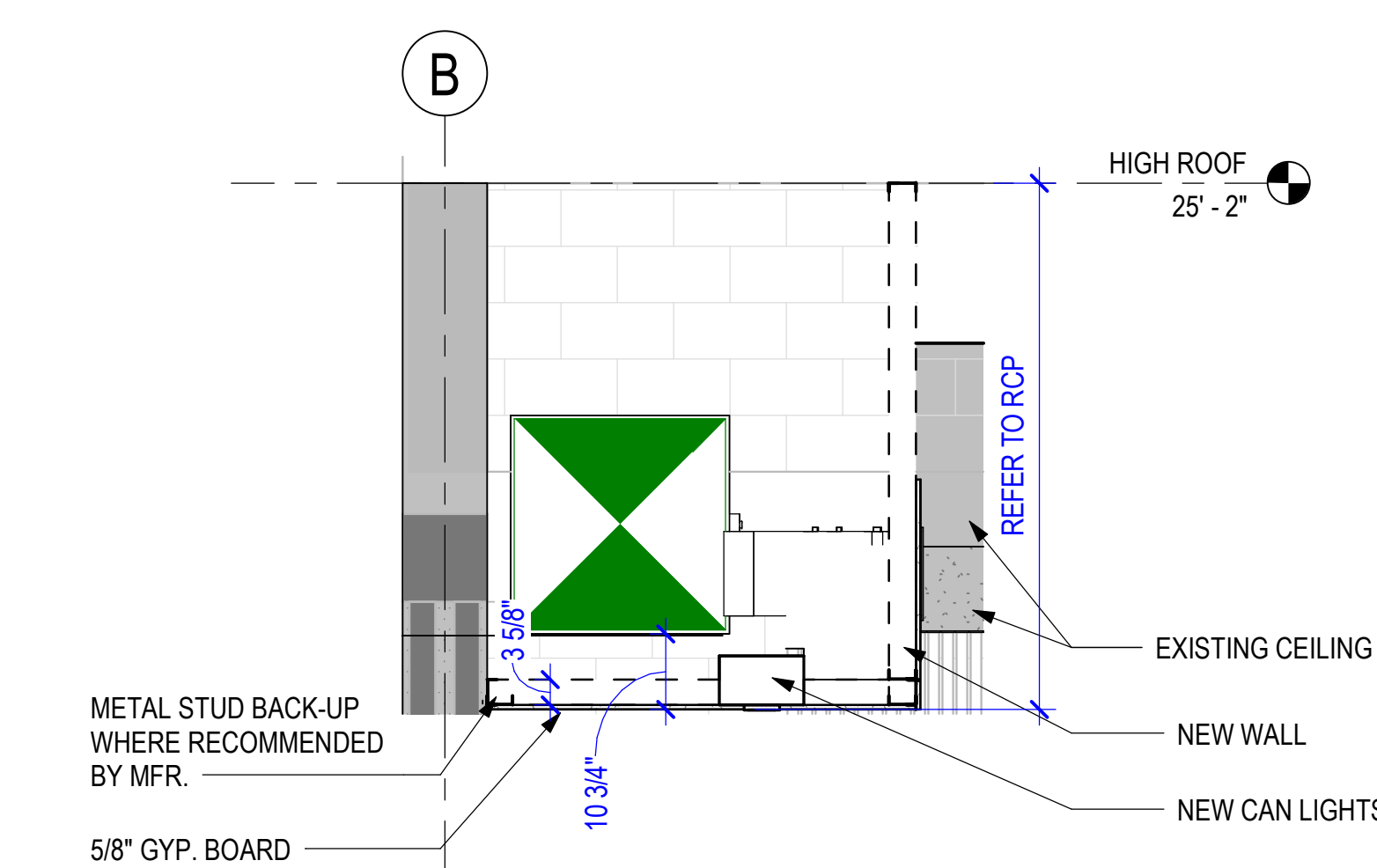
3 FURR OUT - AUDITORIUM CEILING 1/2" = 1'-0"
