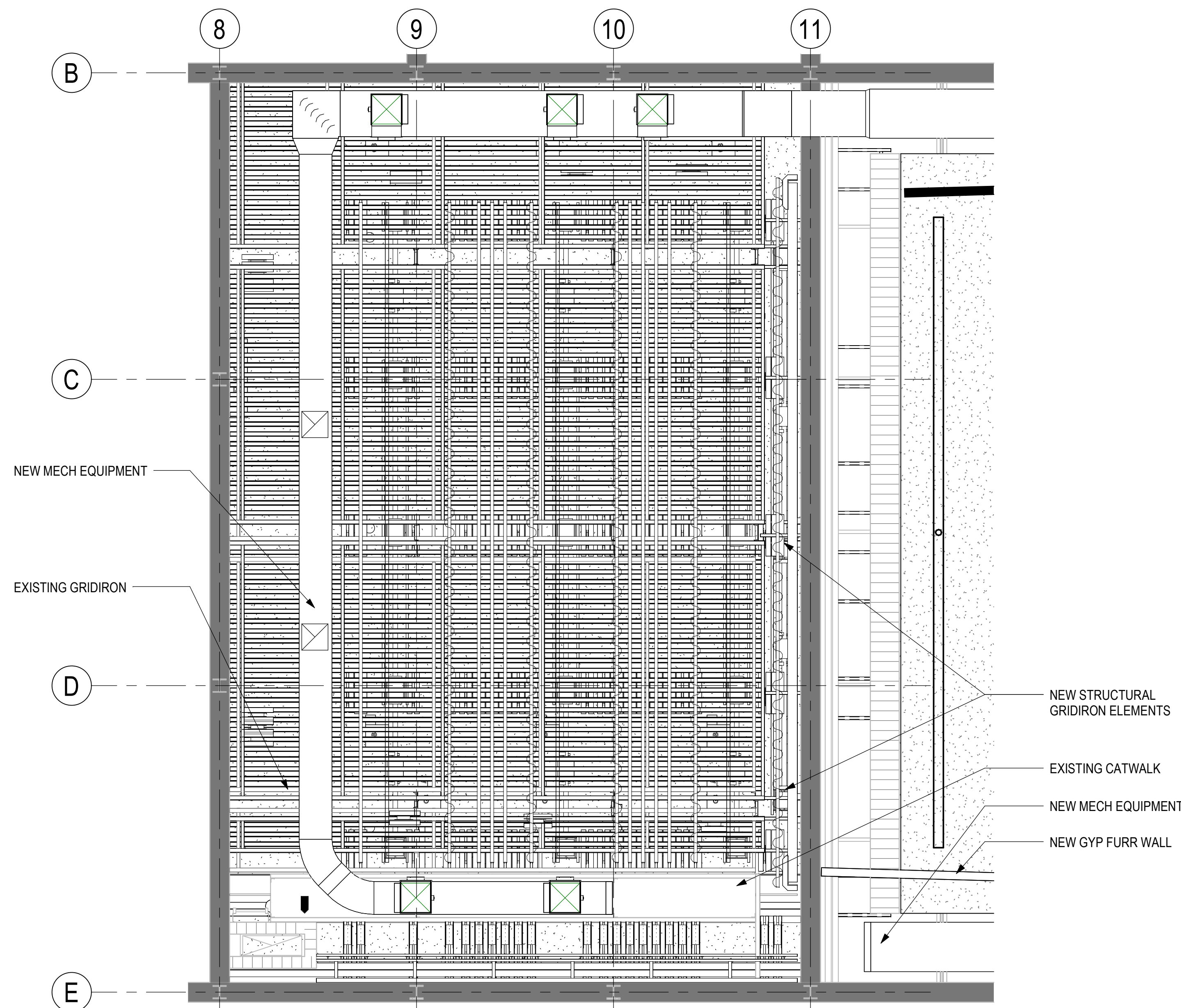
2 REFLECTED CEILING PLAN - STAGE 1/4" = 1'-0"
