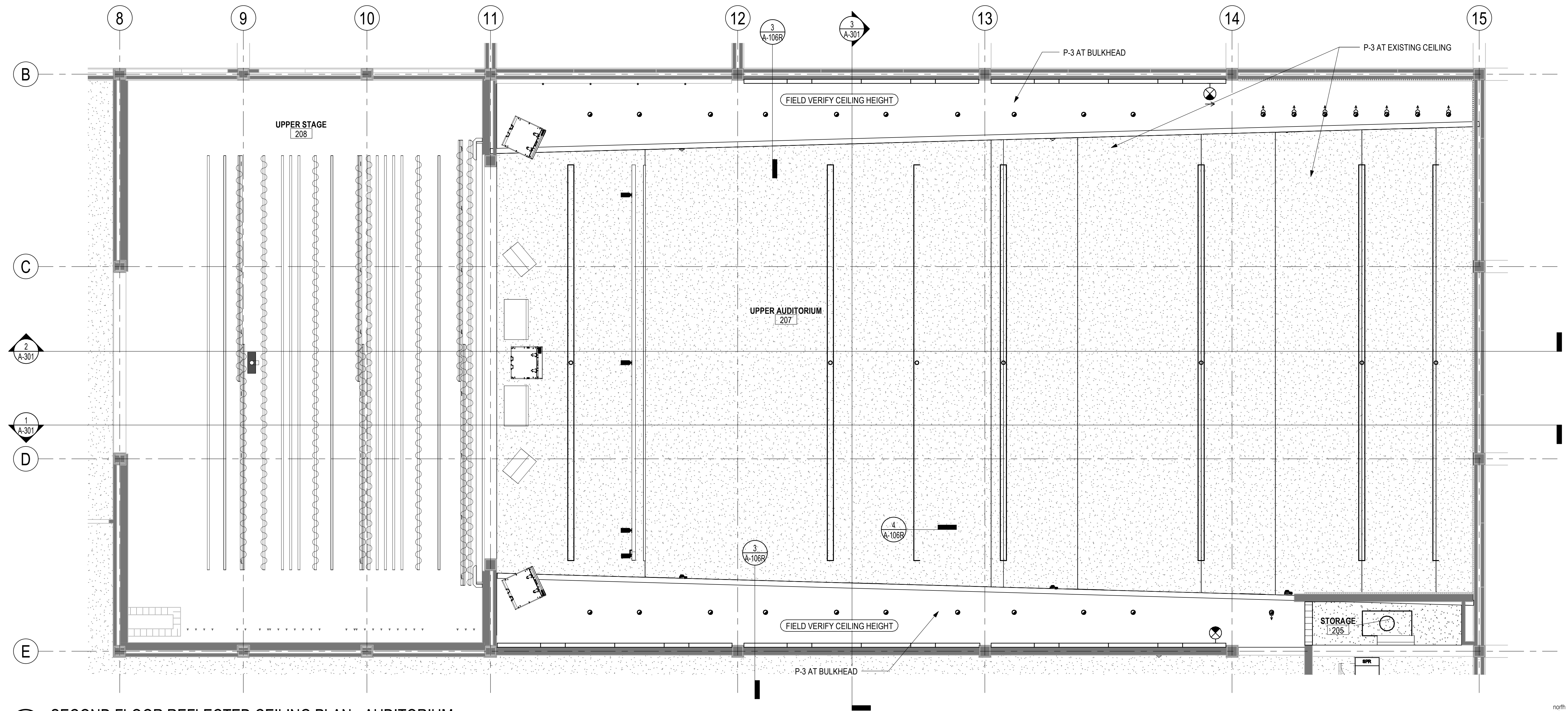
1 SECOND FLOOR REFLECTED CEILING PLAN - AUDITORIUM 1/4" = 1'-0"
