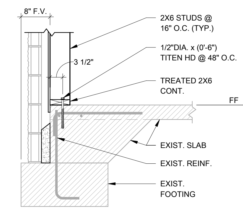
1 SECTION 3/4" = 1'-0"
