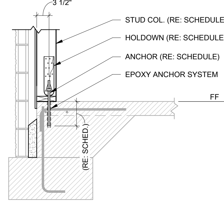
2 SECTION 3/4" = 1'-0"
