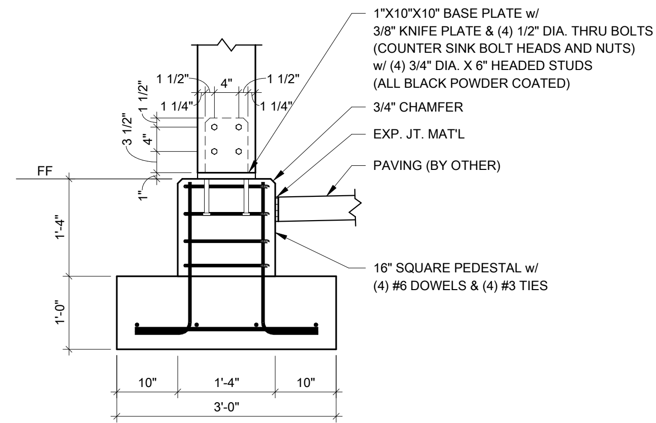
6 SECTION 3/4" = 1'-0"
