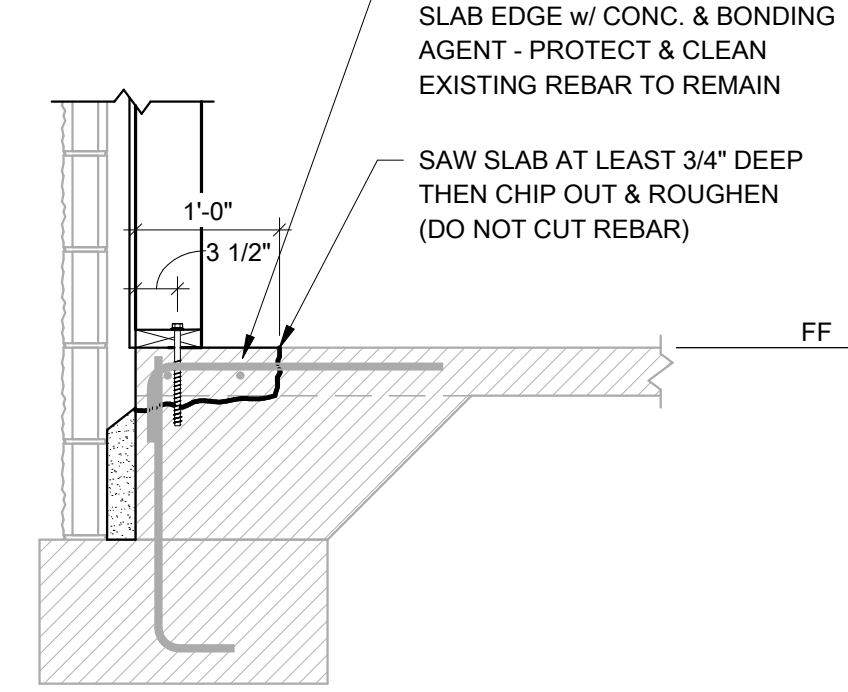
3 SECTION 3/4" = 1'-0"
