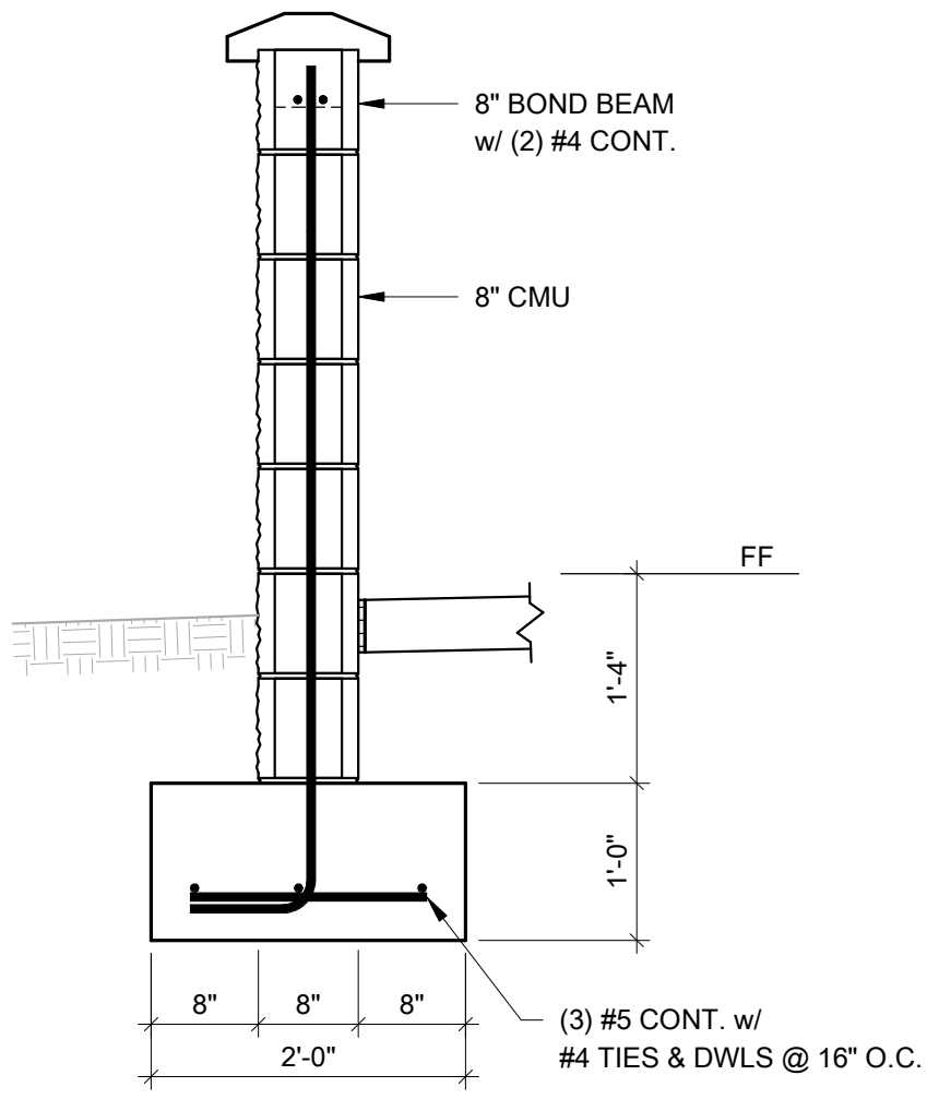
7 SECTION 3/4" = 1'-0"
