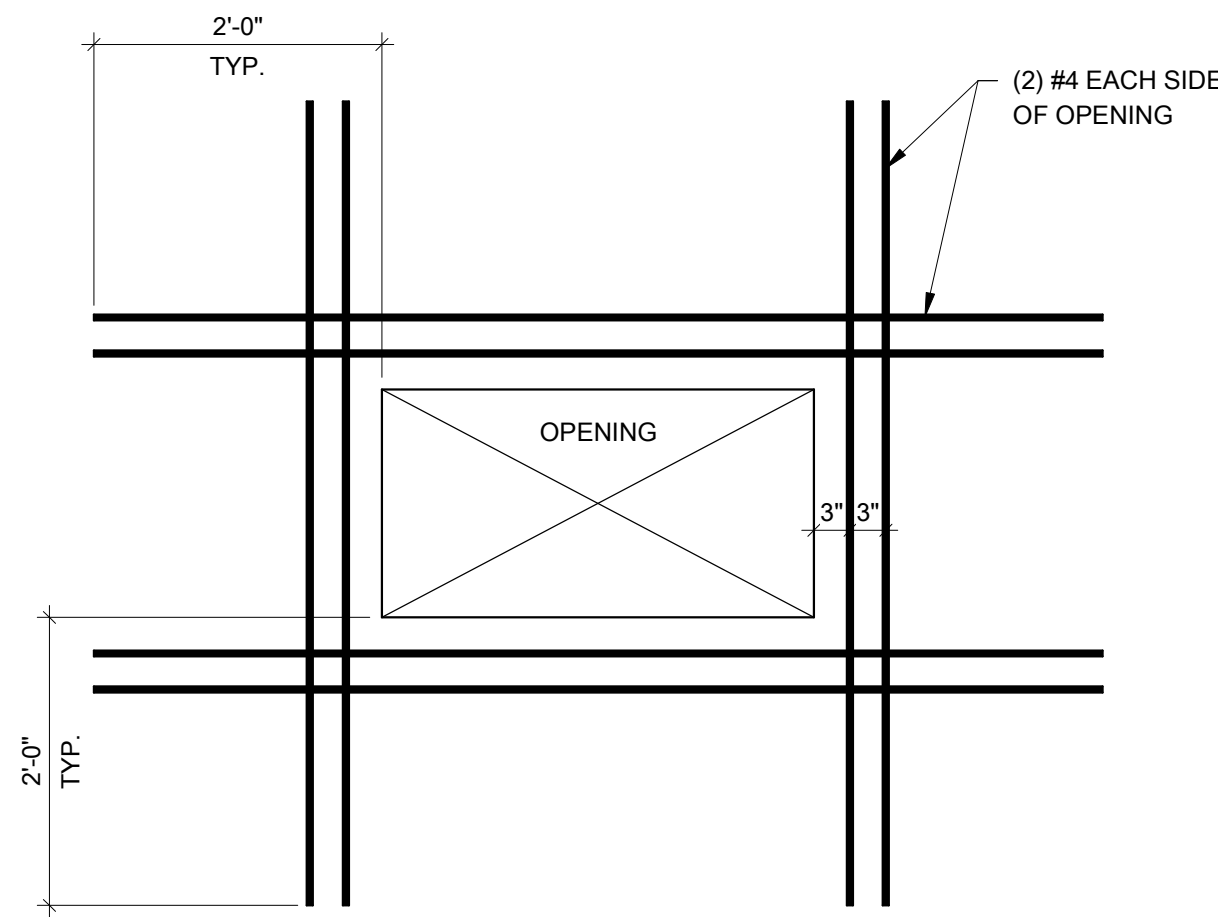
5 TYP. REINF. @ SLAB OPENINGS & PIPE PENETRATIONS 3/4" = 1'-0"
