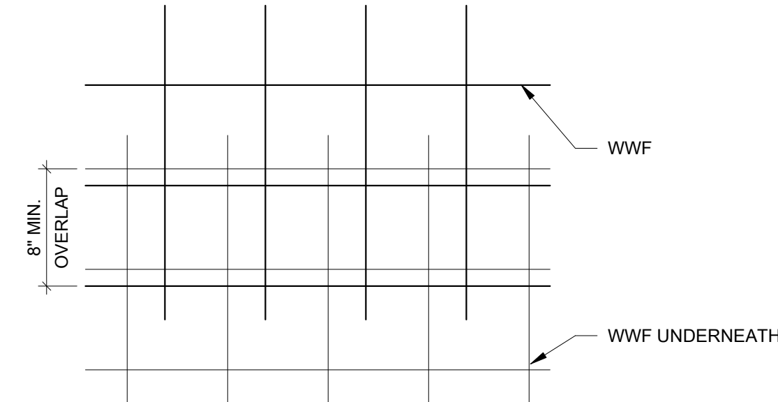
4 TYP. WWF OVERLAP 1 1/2" = 1'-0"
