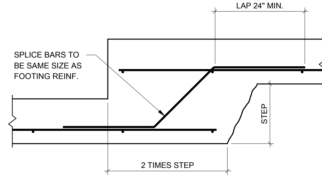
3 TYPICAL CONT. FOOTING STEP DETAIL 3/4" = 1'-0"
