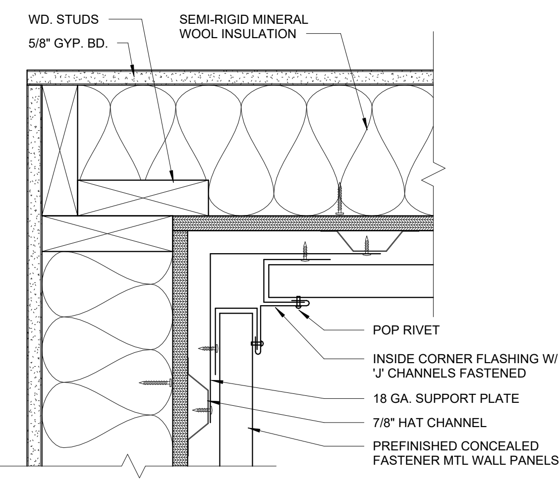
1 ENLARGED DETAIL - MP-2 INSIDE CORNER 3" = 1'-0"
