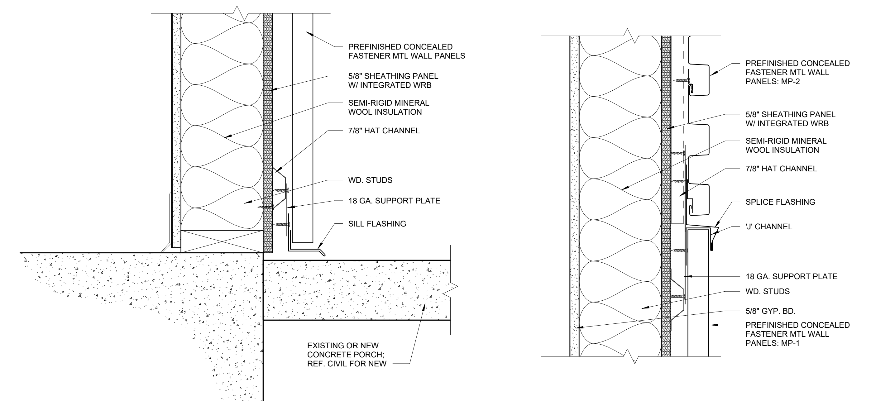
5 ENLARGED DETAIL - MP-1 BASE 3" = 1'-0"
