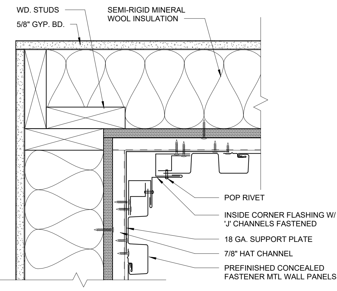
6 ENLARGED DETAIL - MP-1 INSIDE CORNER 3" = 1'-0"
