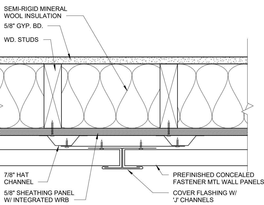
3 ENLARGED DETAIL - MP-2 SPLICE 3" = 1'-0"
