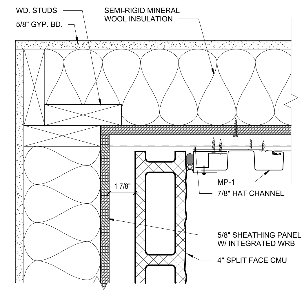
12 ENLARGED DETAIL - MP-1 TO CMU INSIDE CORNER 3" = 1'-0"
