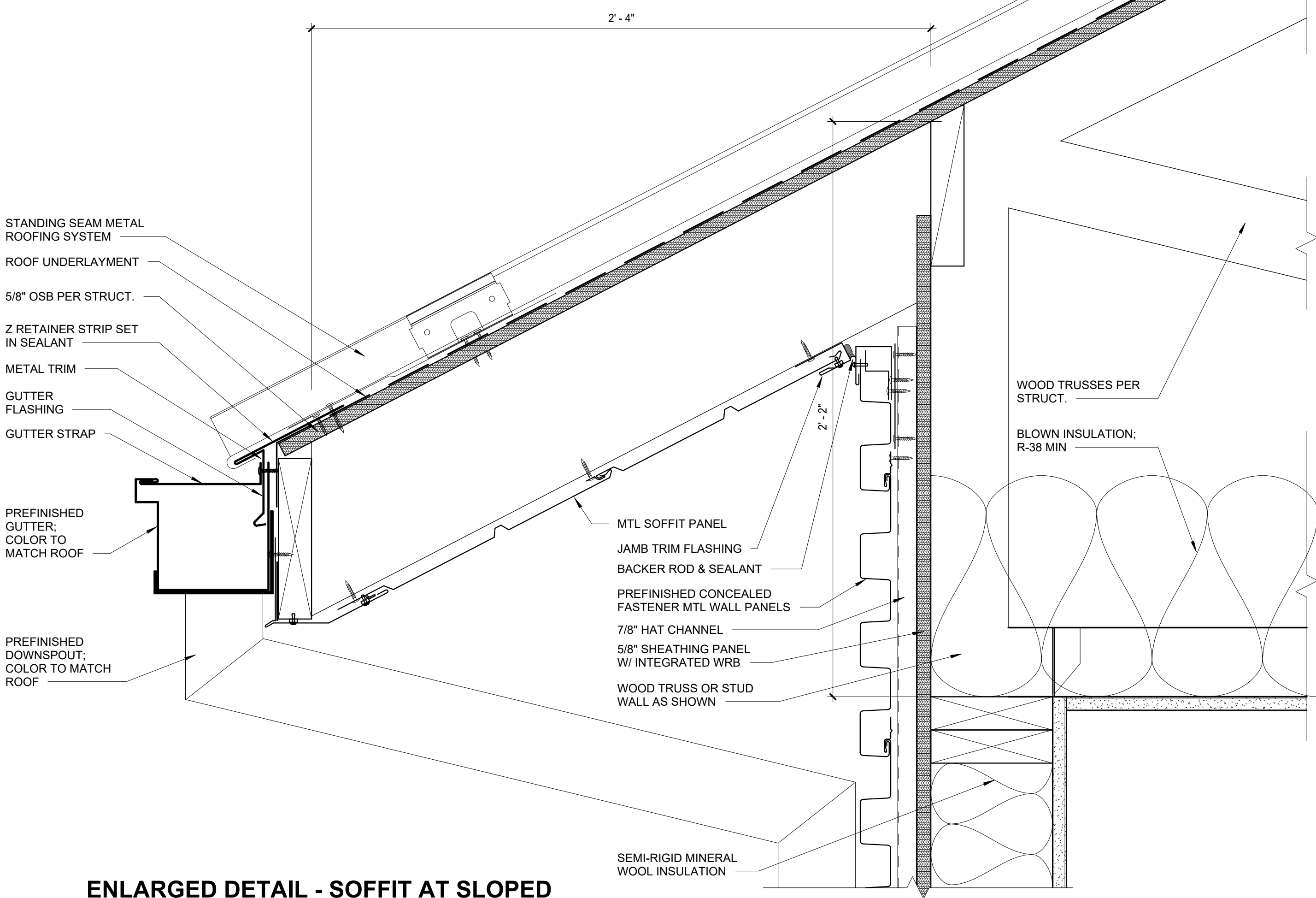
9 ENLARGED DETAIL - SOFFIT AT SLOPED ROOF 3" = 1'-0"
