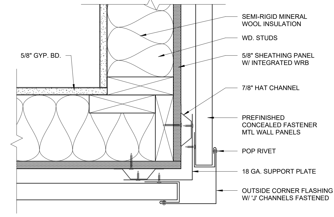
2 ENLARGED DETAIL - MP-2 OUTSIDE CORNER 3" = 1'-0"
