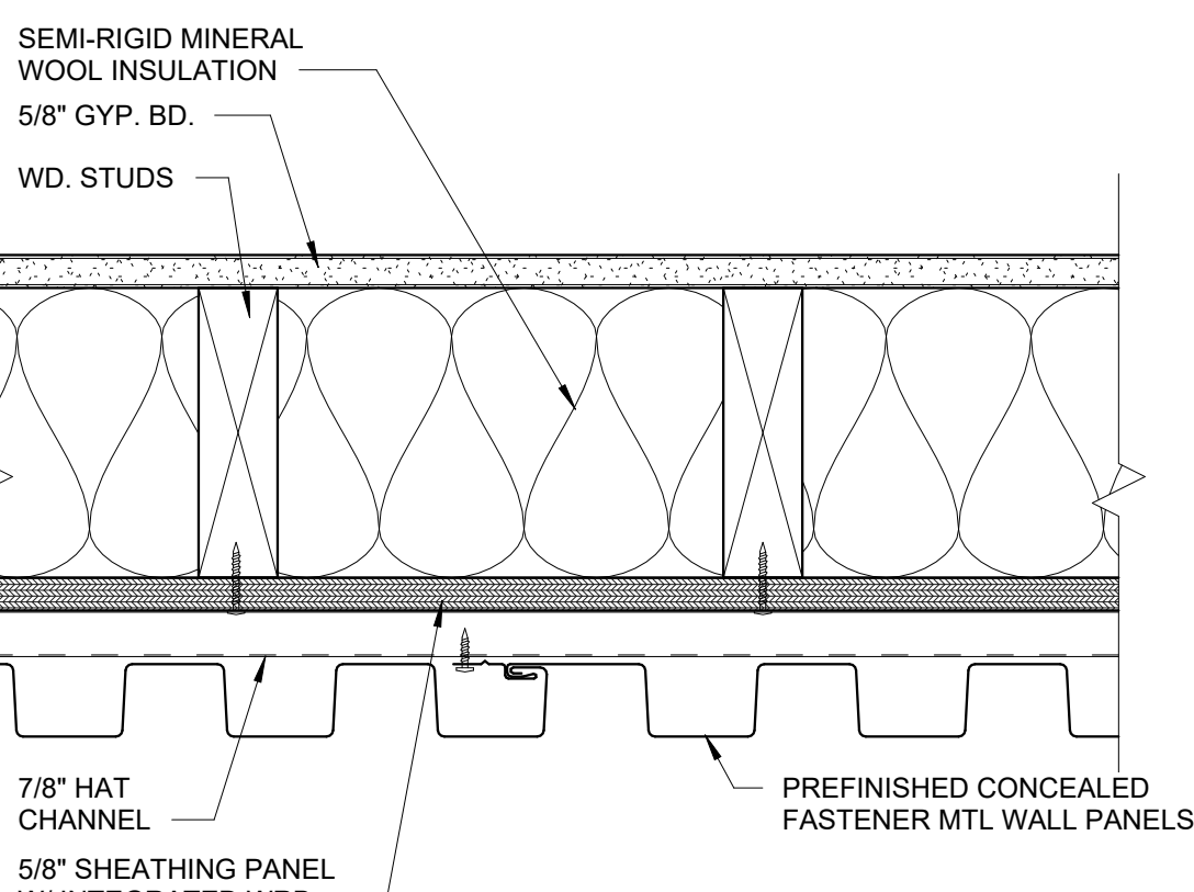
8 ENLARGED DETAIL - MP-1 TYPICAL 3" = 1'-0"
