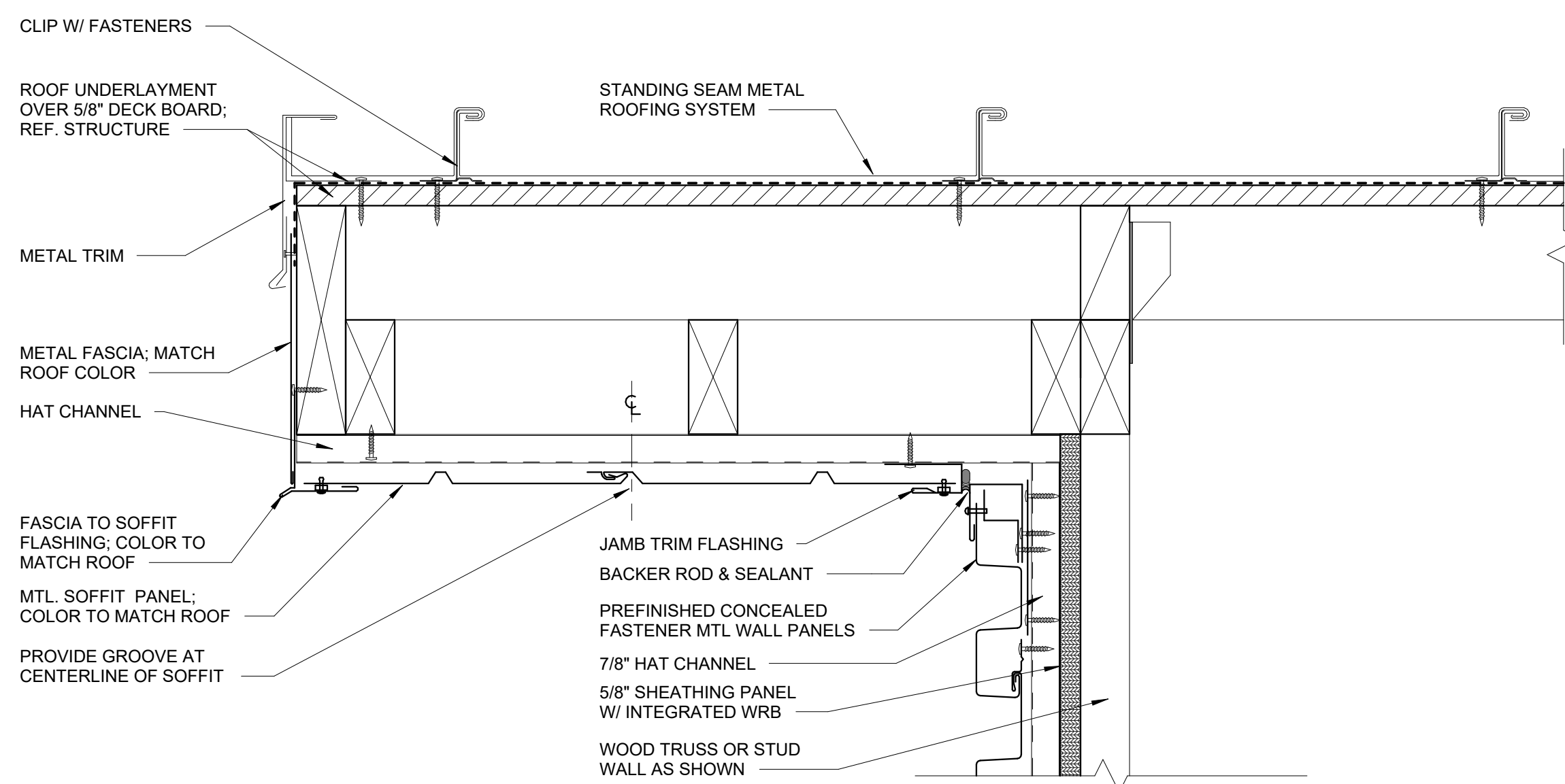
13 ENLARGED DETAIL - SOFFIT SPLICE 3" = 1'-0"
