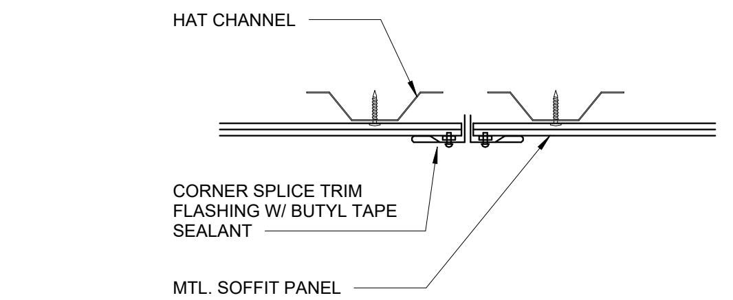
13 ENLARGED DETAIL - SOFFIT SPLICE 3" = 1'-0"
