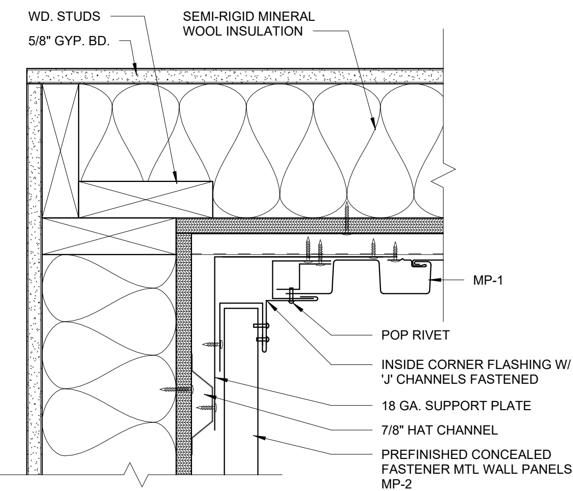
10 ENLARGED DETAIL - MP-1 TO MP-2 INSIDE CORNER 3" = 1'-0"
