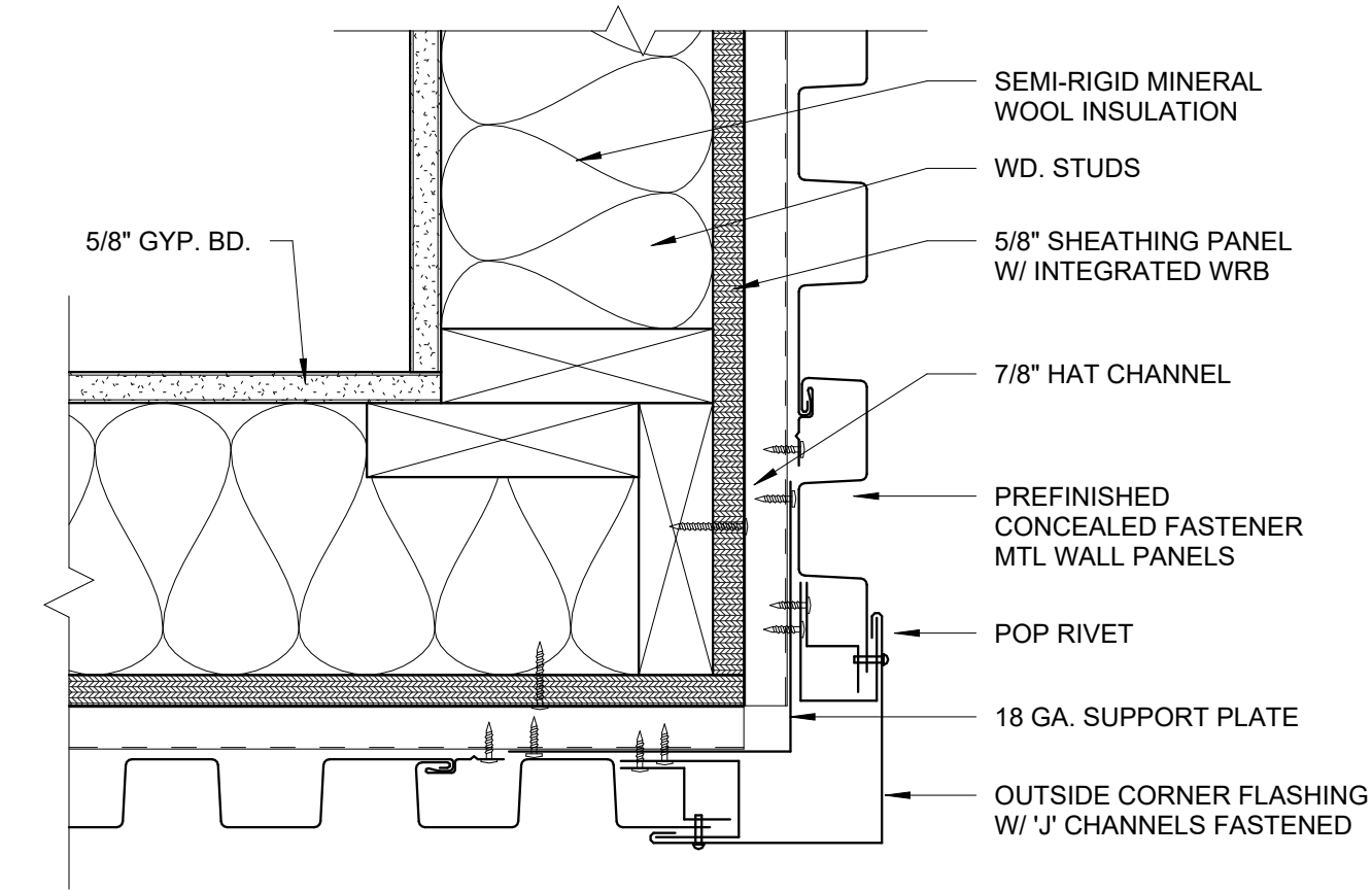
7 ENLARGED DETAIL - MP-1 OUTSIDE CORNER 3" = 1'-0"
