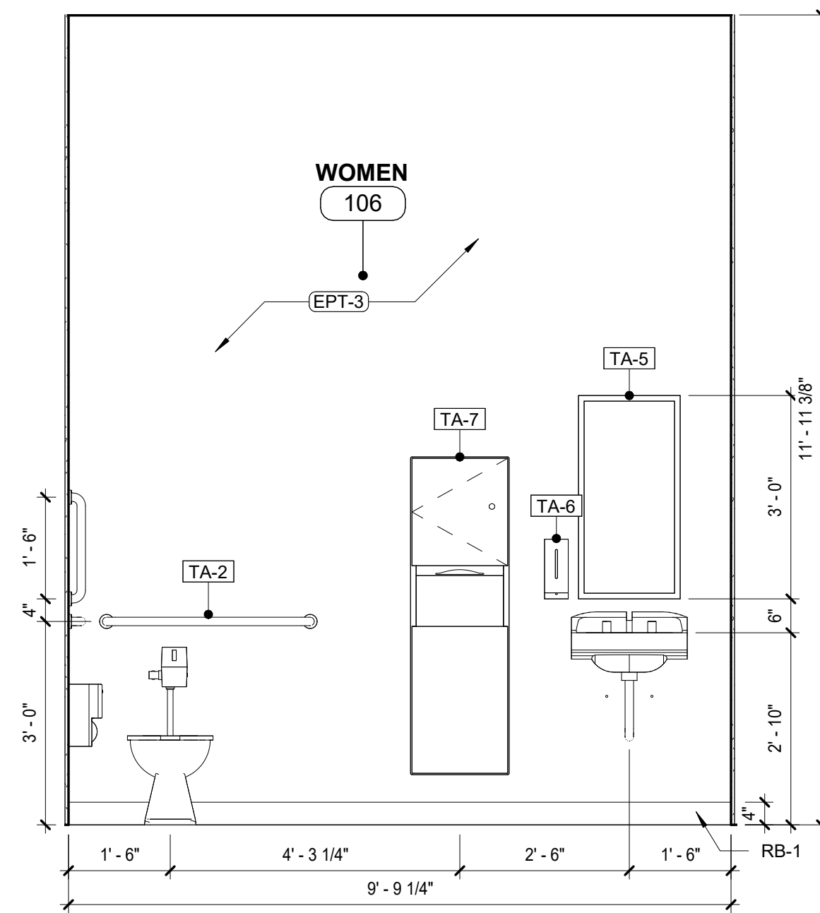
7 TOILET ELEVATION 1/2" = 1'-0"
