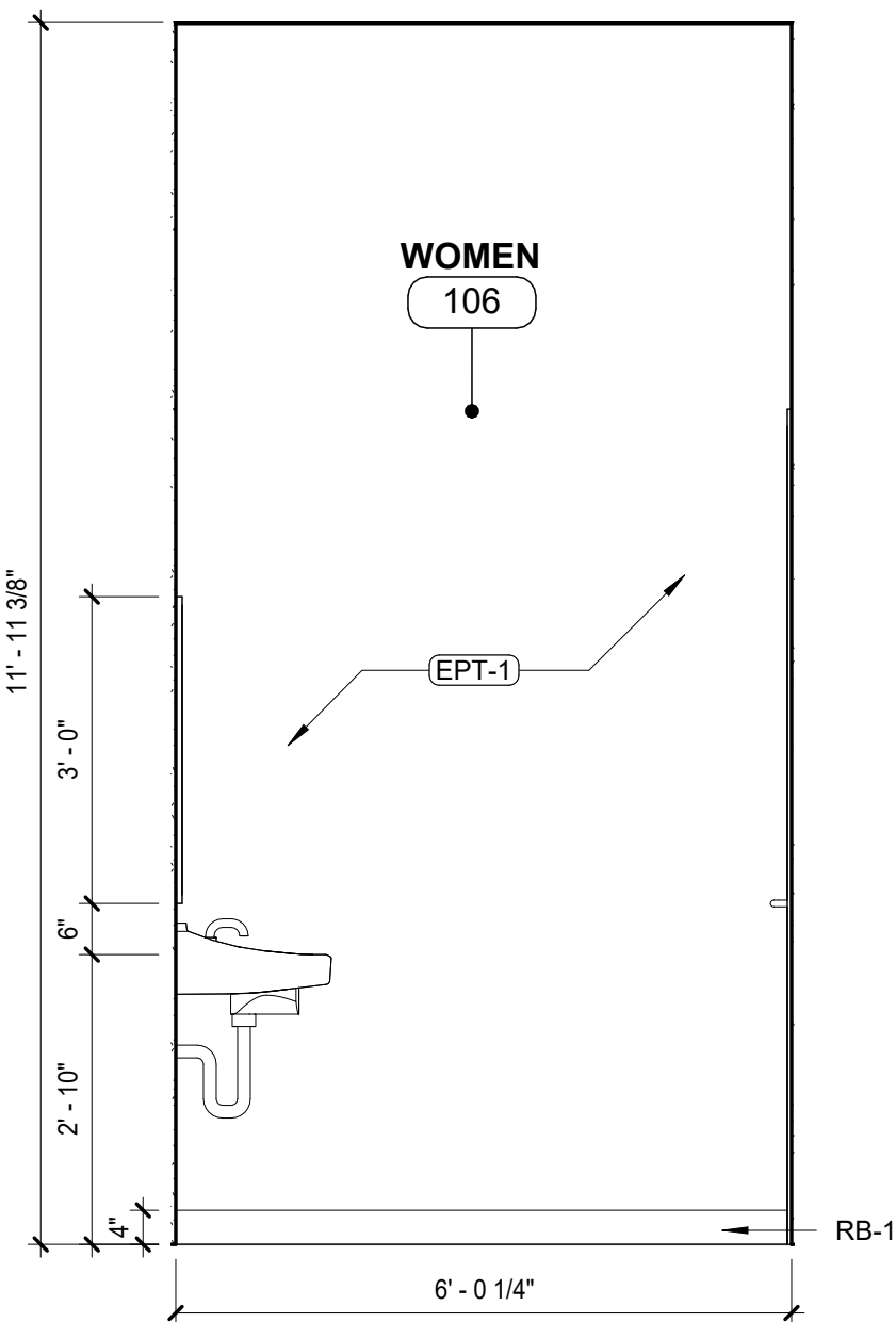
10 TOILET ELEVATION 1/2" = 1'-0"
