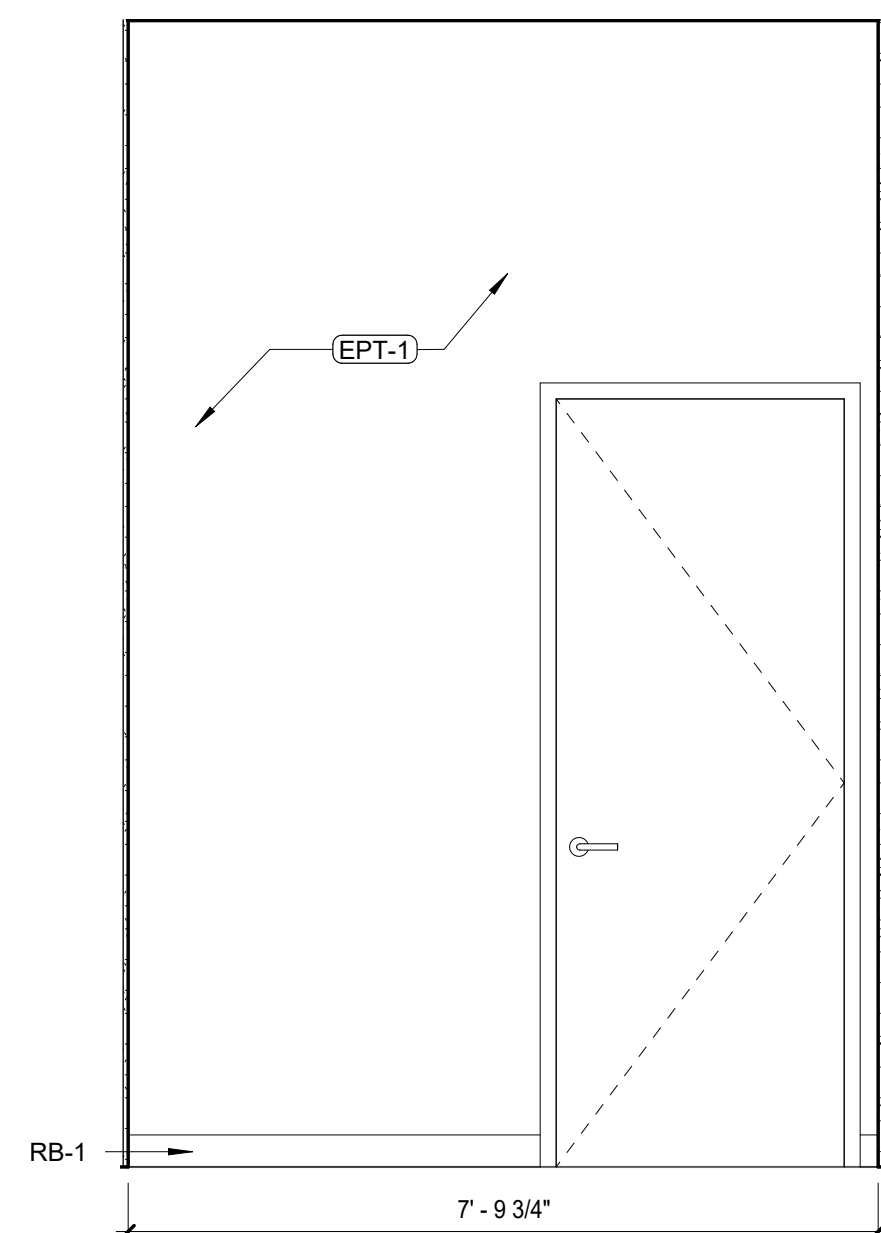
2 TOILET ELEVATION 1/2" = 1'-0"
