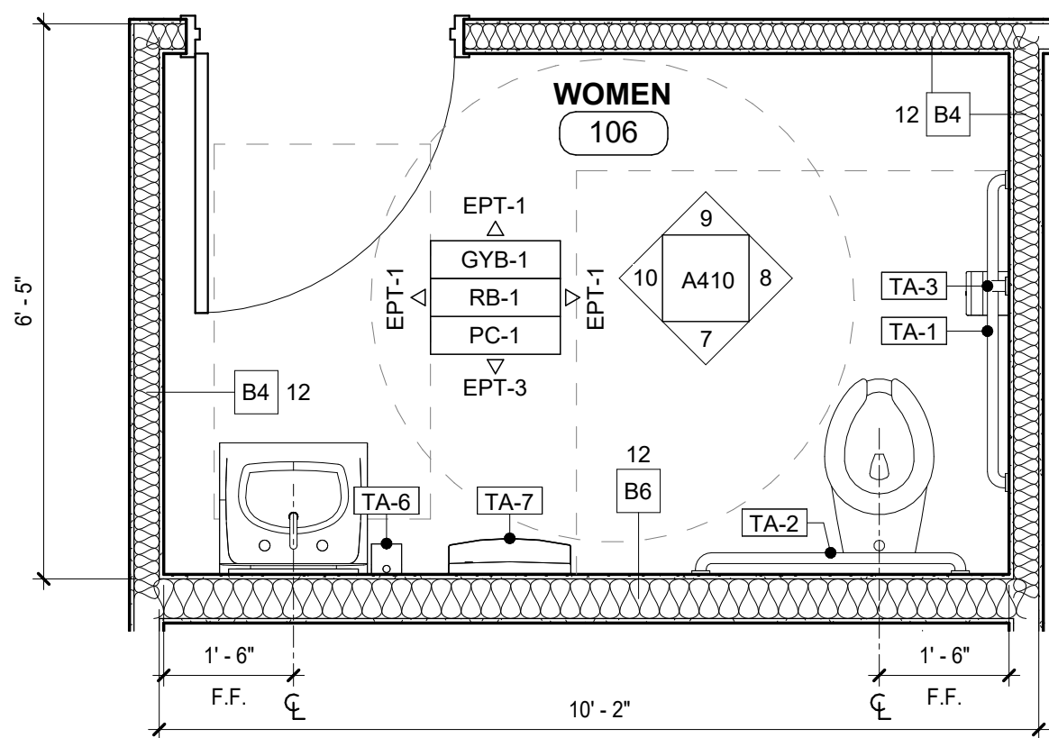
6 ENLARGED TOILET PLAN 1/2" = 1'-0"
