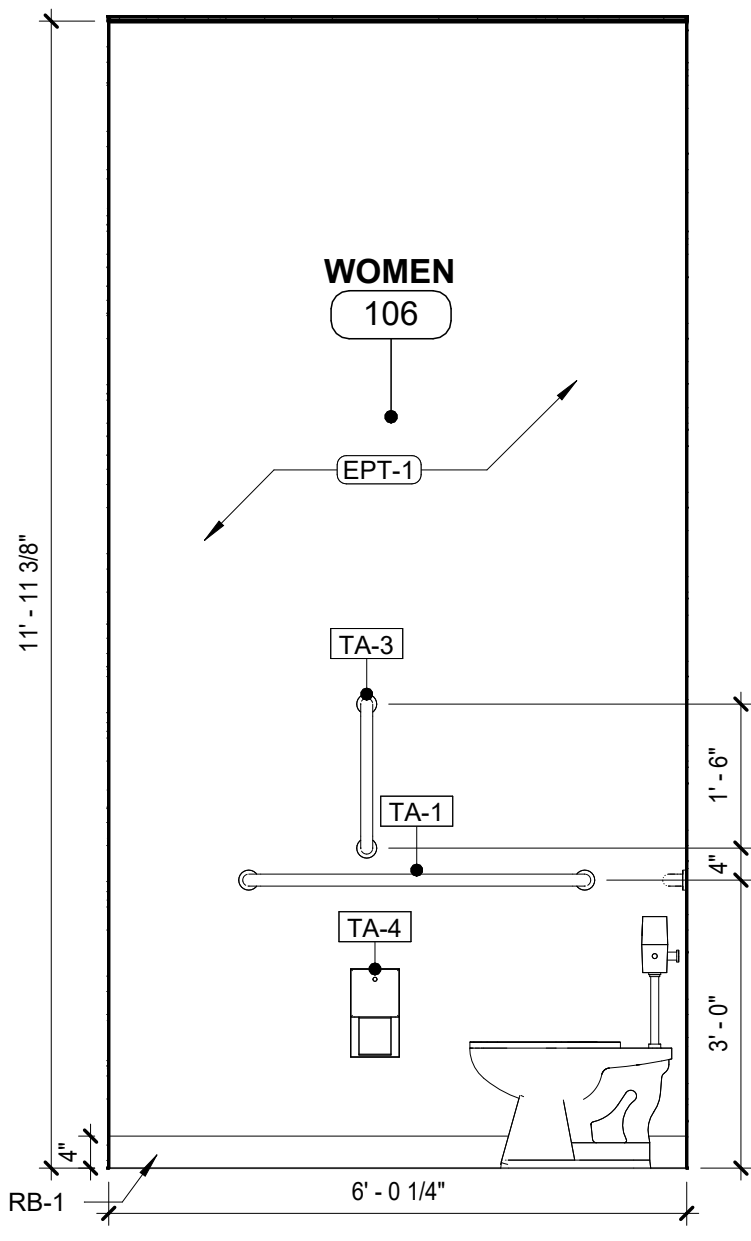
8 TOILET ELEVATION 1/2" = 1'-0"
