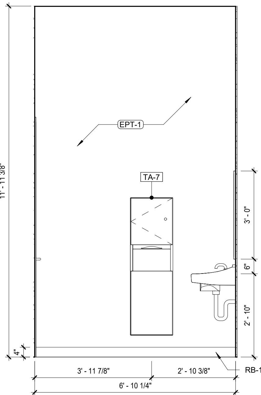
5 TOILET ELEVATION 1/2" = 1'-0"
