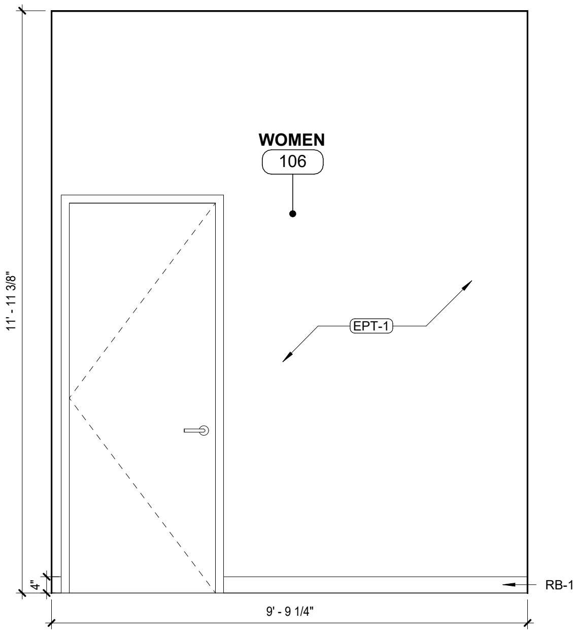
9 TOILET ELEVATION 1/2" = 1'-0"
