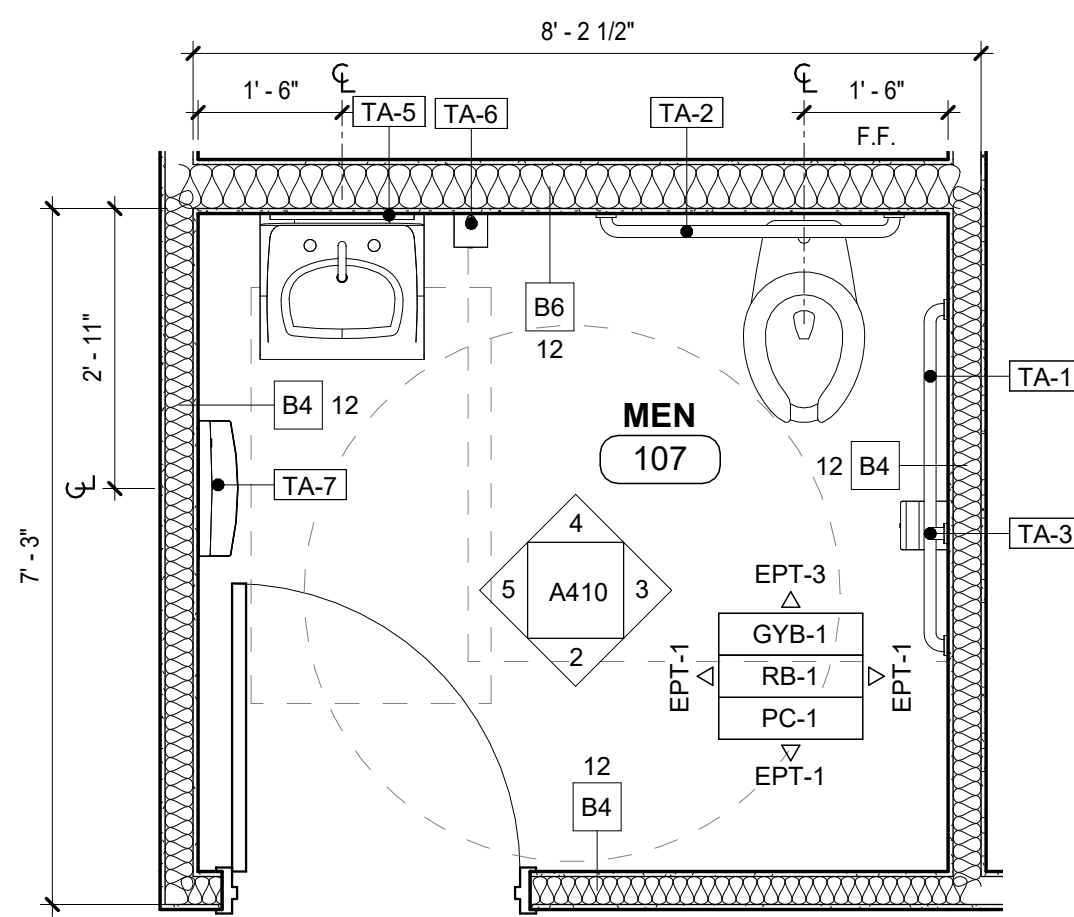
1 ENLARGED TOILET PLAN 1/2" = 1'-0"
