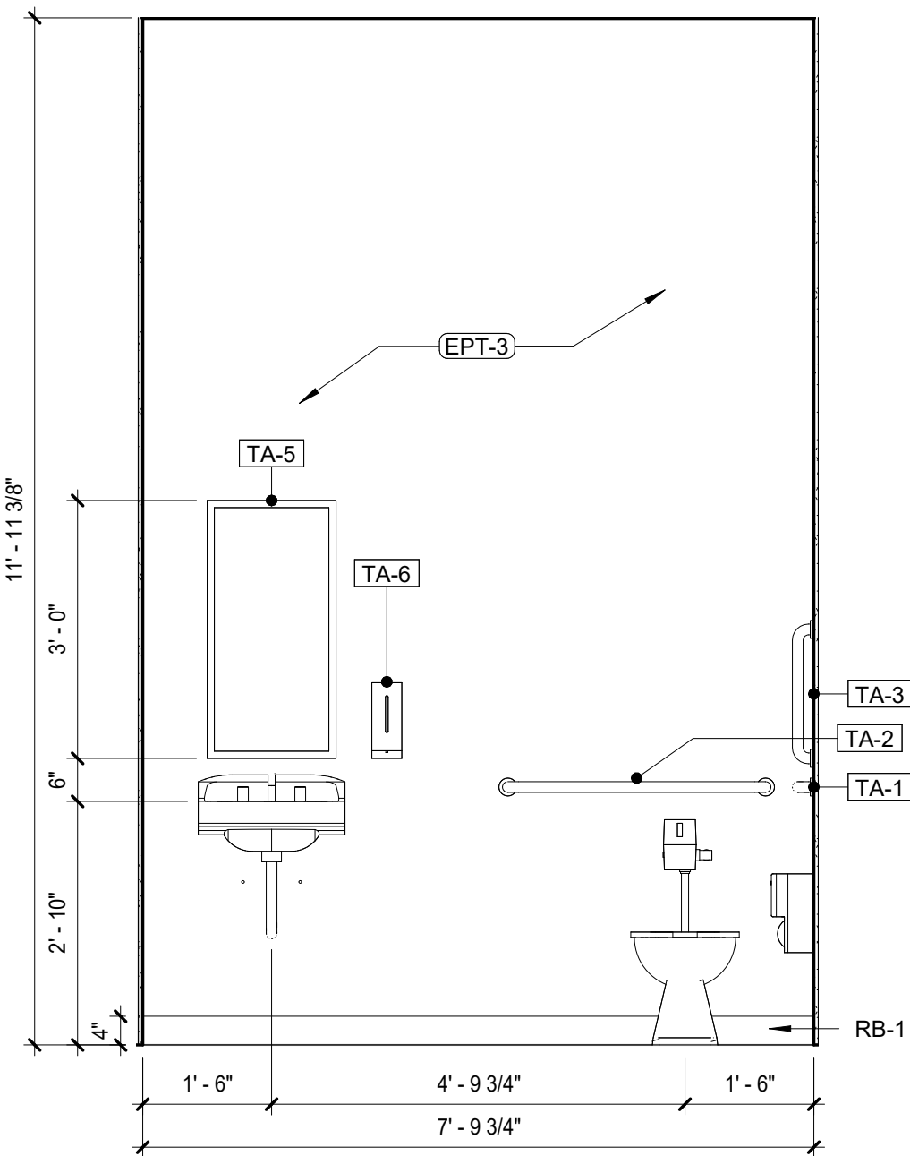
4 TOILET ELEVATION 1/2" = 1'-0"
