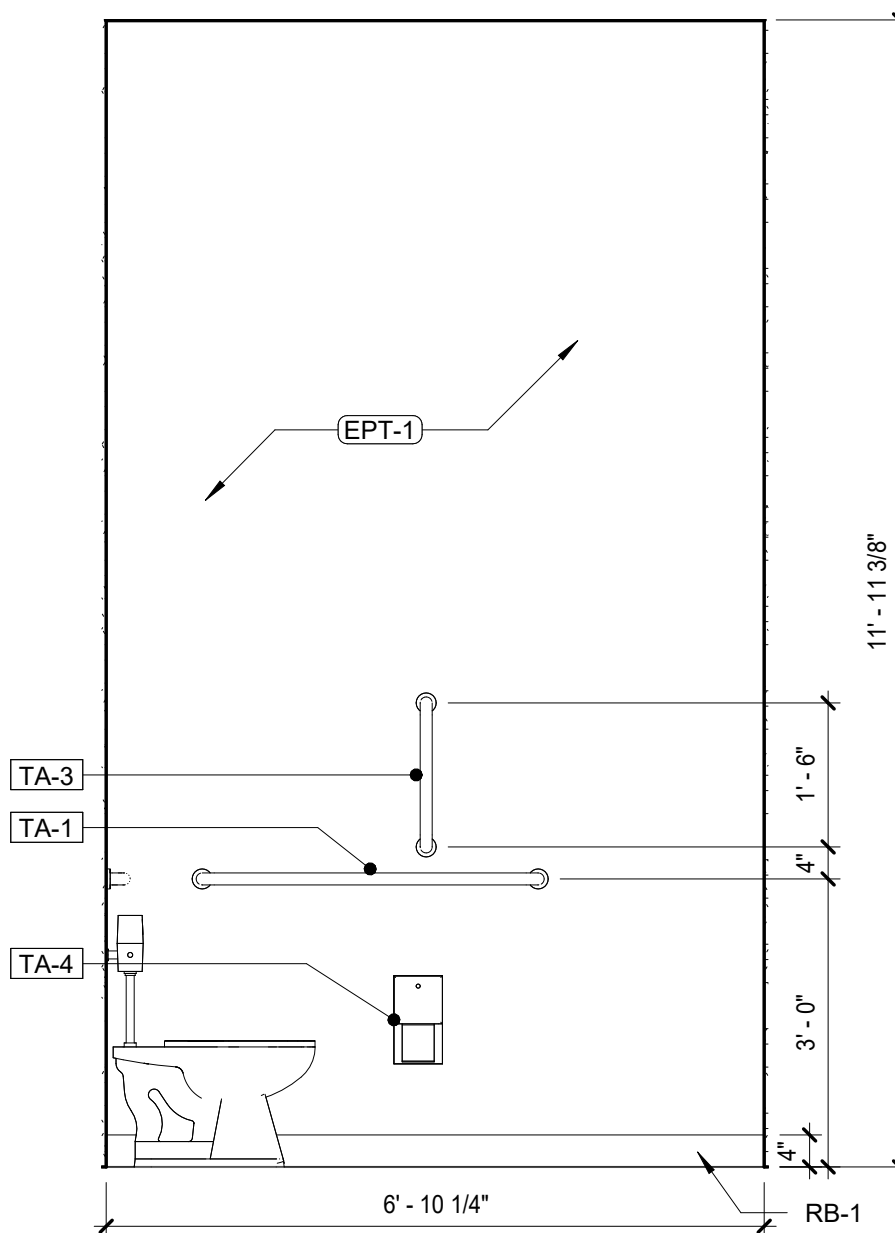
3 TOILET ELEVATION 1/2" = 1'-0"
