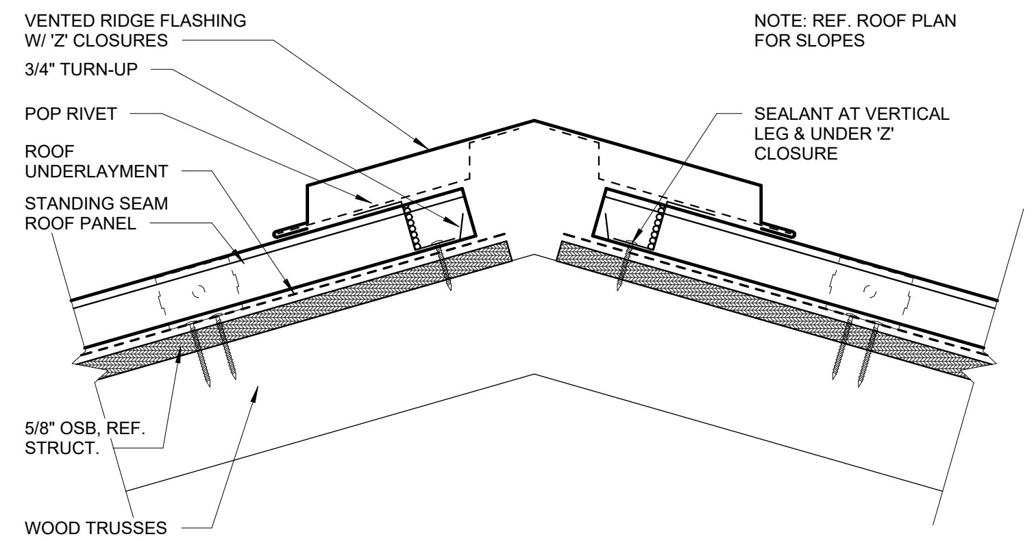
6 ROOF DETAIL - RIDGE VENT 3" = 1'-0"
