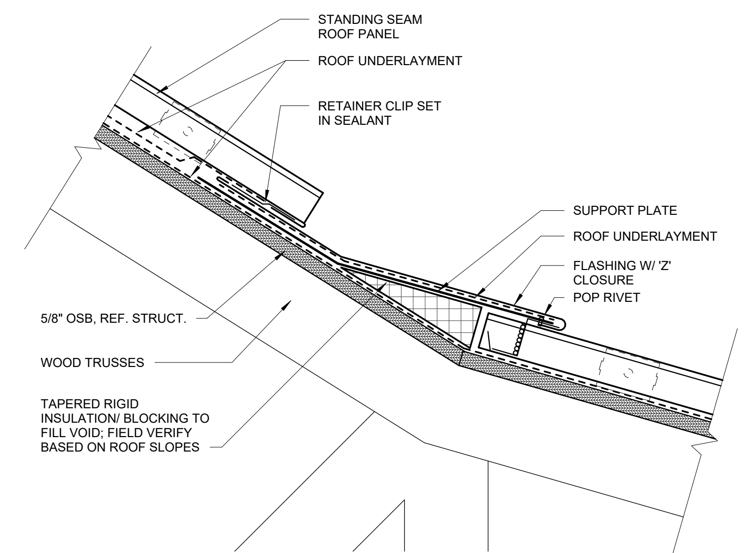
3 ROOF DETAIL - SLOPE TRANSITION 3" = 1'-0"
