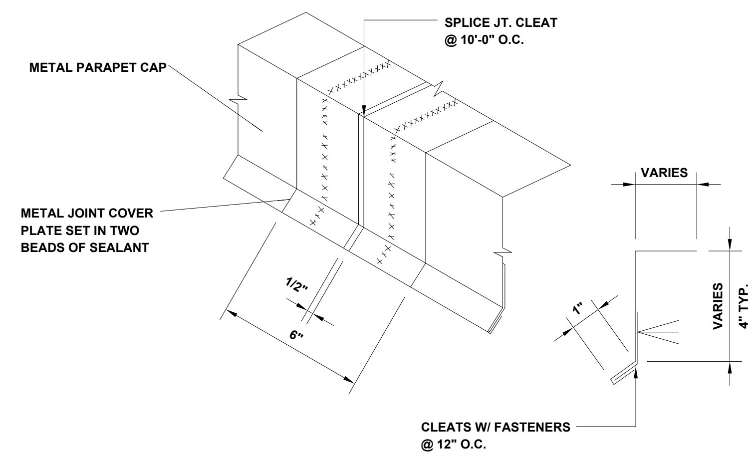
4 ROOF - TYPICAL CAP / COUNTER FLASHING N.T.S.
