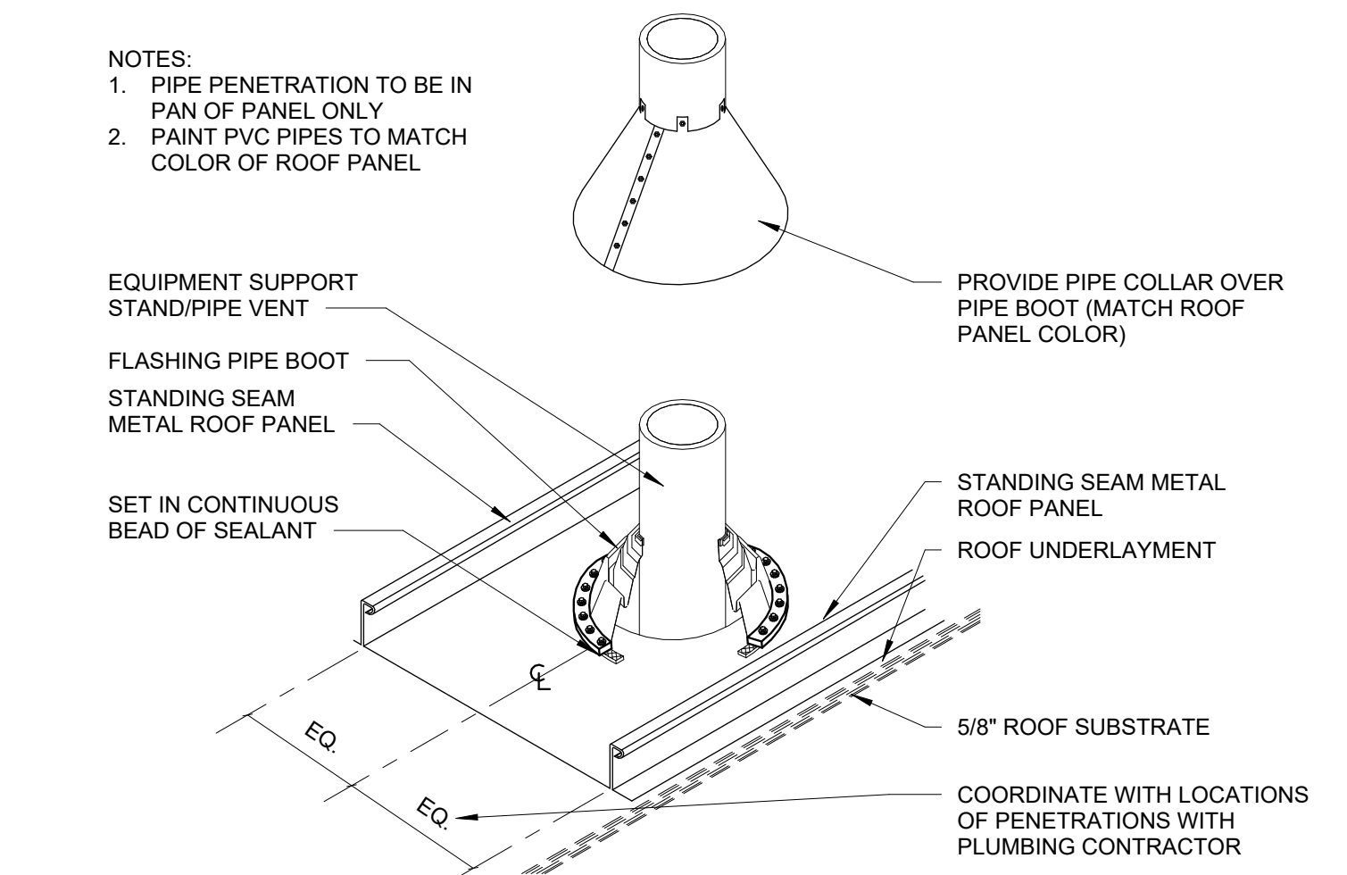
5 ROOF DETAIL - PIPE PENETRATION 1 1/2" = 1'-0"
