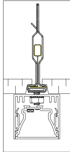
Tegular Tile
