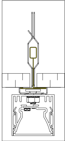
Standard Tile
