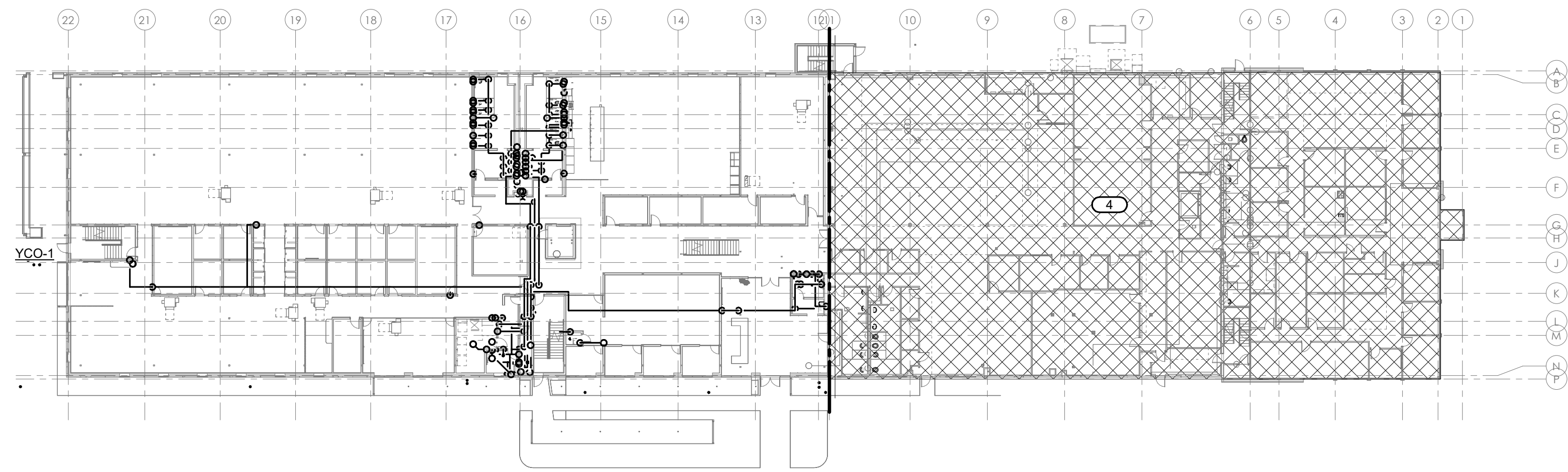
2 LEVEL 01 PLUMBING PLAN 1/32" = 1'-0"
